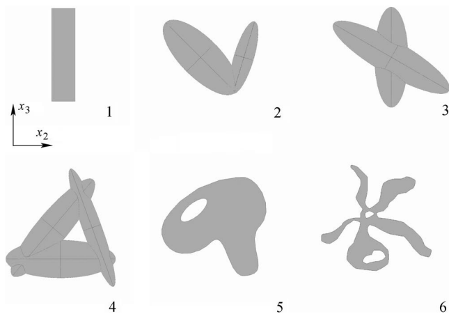
Figure 9. Irregular vertical cracks. All fractures are planar; their normals are directed along the x_1 -axis. The faces of cracks 2, 3, and 4 have sharp edges. Geometries 4, 5, and 6, that contain interior rock islands, represent partially closed fractures.
