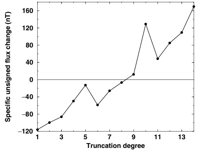
Figure 4. Change in specific integrated unsigned flux between epoch 2000.5 and 2001.5 as a function of model truncation. For example, at degree 7, B_r is calculated at both epochs with Gauss coefficients only up to and including l = 7 .
