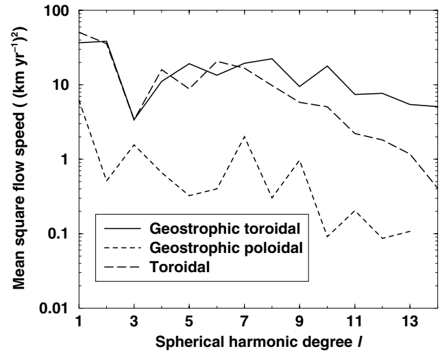
Figure 8. Power spectra for flows. For a geostrophic flow truncated at degrees 13–14, the poloidal power at degree 14 is required to be 0.
