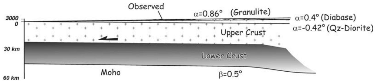
Figure 17. Model results. Topographic slopes obtained for different compositions of the lower crust (granulite, diabase or quartz-diorite). The values of the effective viscosities and shear stresses for granulite and diabase are sufficient to reproduce the observed topographic slopes in the Fars.
