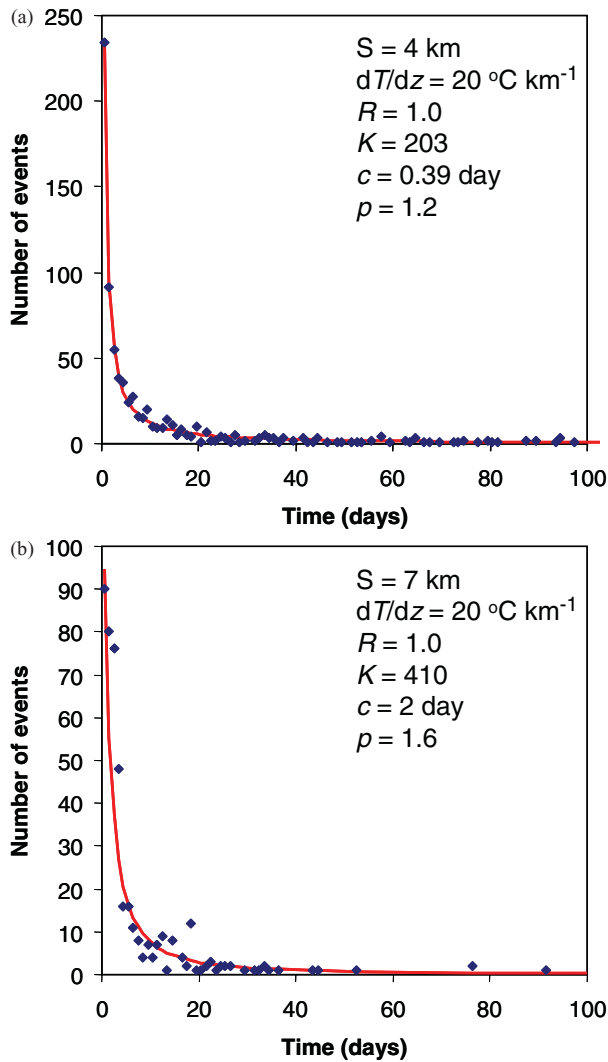
Figure 6. (a) Daily rates of aftershocks in a 3-D model realization having a weak sedimentary cover of 4 km, R = 1.0 , and temperature gradient of 20^{\circ}\text{C km}^{-1} . The line gives least-squares fit to the data points based on the modified Omori law with parameters given in the legend. (b) Same as (a) with a weak sedimentary cover of 7 km.
