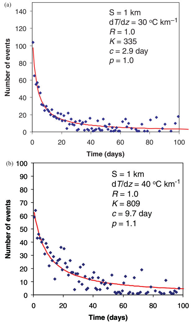
Figure 7. (a) Daily rates of aftershocks in a 3-D model realization having a temperature gradient of 30^{\circ}\text{C km}^{-1} , R = 1.0 , and weak sedimentary cover of 1 km. The line gives least-squares fit to the data points based on the modified Omori law with parameters given in the legend. (b) Same as (a) with a temperature gradient of 40^{\circ}\text{C km}^{-1} .
