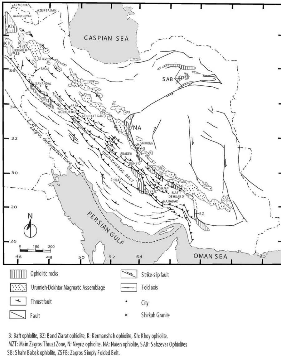
Fig. 2. Simplified structural map of Zagros Orogenic Belt (derived from Alavi, 1994).
