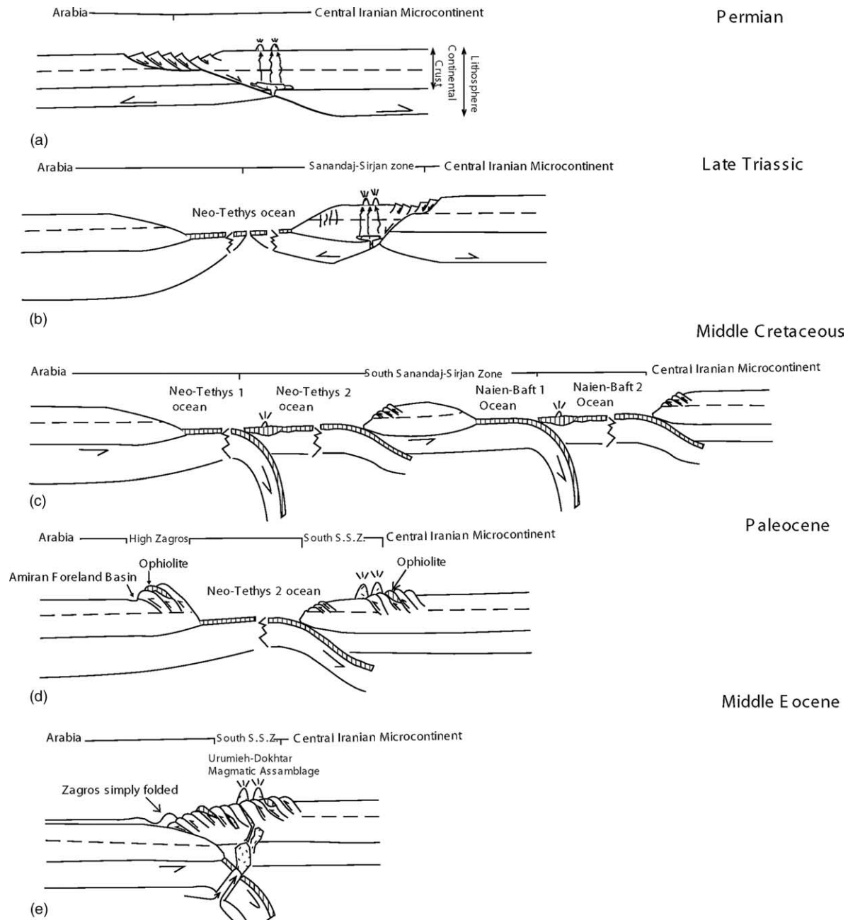
Fig. 3. Tectonic evolution of the South Sanandaj–Sirjan Zone (SSZ). (a) Permian rifting; (b) second rifting phase in Late Triassic; (c) the closure of the Neo-Tethys and Naien-Baft Oceans occurred at first as a collision with an oceanic island arc; (d) ophiolite emplacement along the SSZ and on the Central Iranian Microcontinent; (e) Middle Eocene slab break-off.
