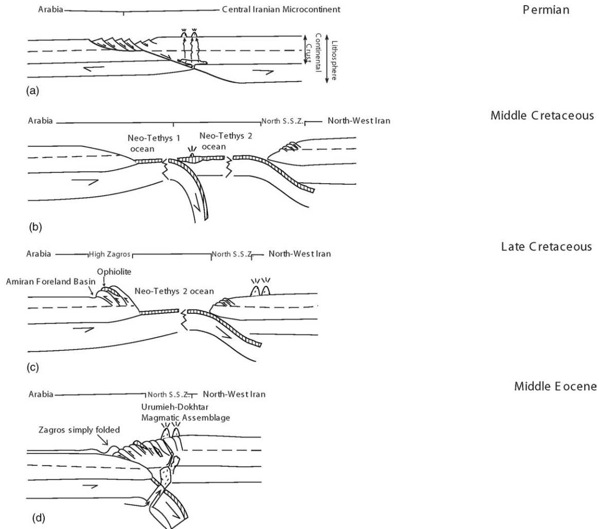
Fig. 4. Tectonic evolution of the North Sanandaj–Sirjan zone (NSSZ). (a) Permian rifting; (b) closure of the Neo-Tethys Ocean commencing with an oceanic island arc collision; (c) ophiolite emplacement along the NSSZ; Middle Eocene slab break-off.
