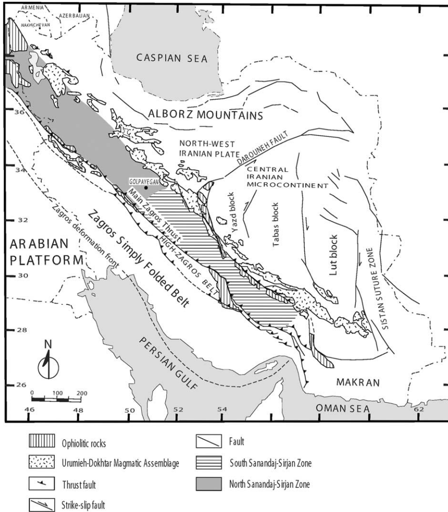
Fig. 1. Main tectonic units of Iran.
