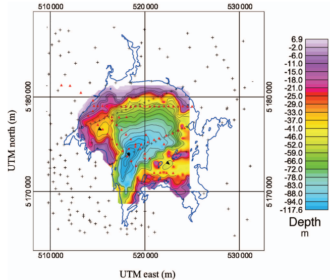
Figure 5. Bathymetry of Lake Wanapitei. The greatest depths of approximately 120 m are found in the southern bay (L'Heureux et al., 2005). Old gravity stations are shown as black crosses; new stations are shown as red triangles; lake outline is in blue. Contour interval is 10 m.
