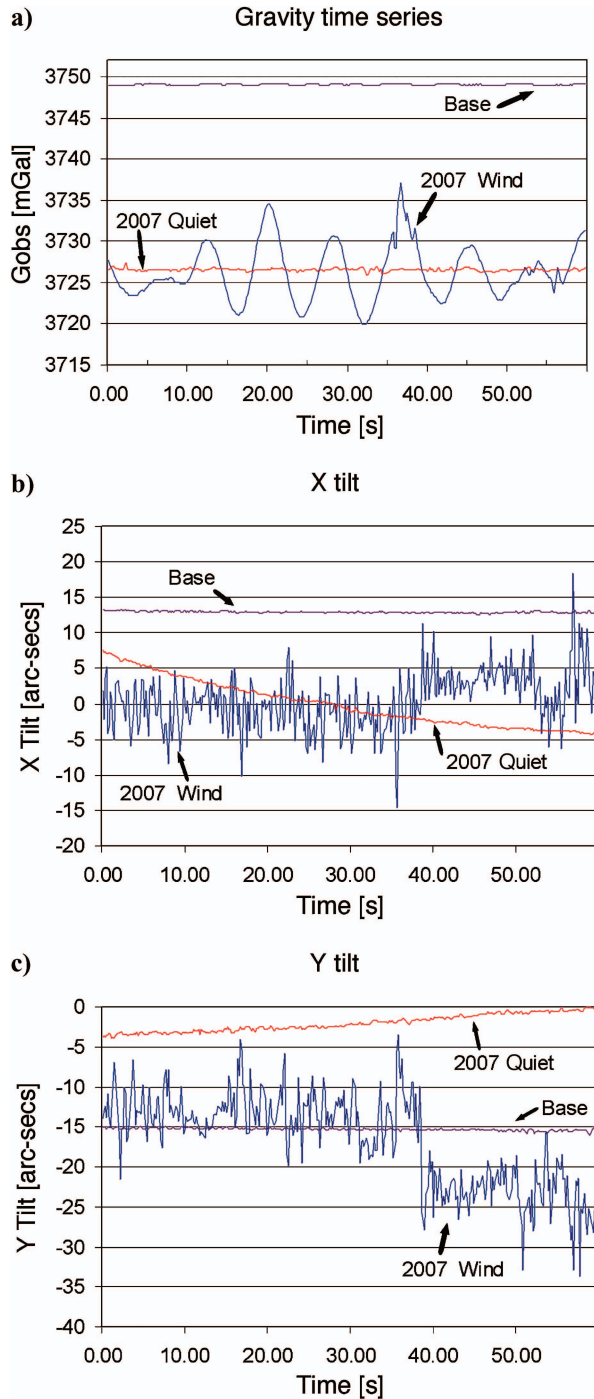
Figure 4. (a) Gravity, (b) X-tilt, and (c) Y-tilt recordings for three stations: the base station (purple line), a station under windy conditions (blue line), and a station under calm conditions (red line).
