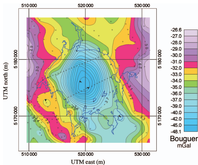
Figure 2. Bouguer gravity anomaly over Wanapitei Lake, as published by Dence and Popelar (1972). Gravity stations are shown as black crosses; lake outline is in blue (extracted from Dressler, 1982). Contour interval is 1 mGal; amplitude of the anomaly is 15 mGal. Data are from the Geological Survey of Canada (GSC).
