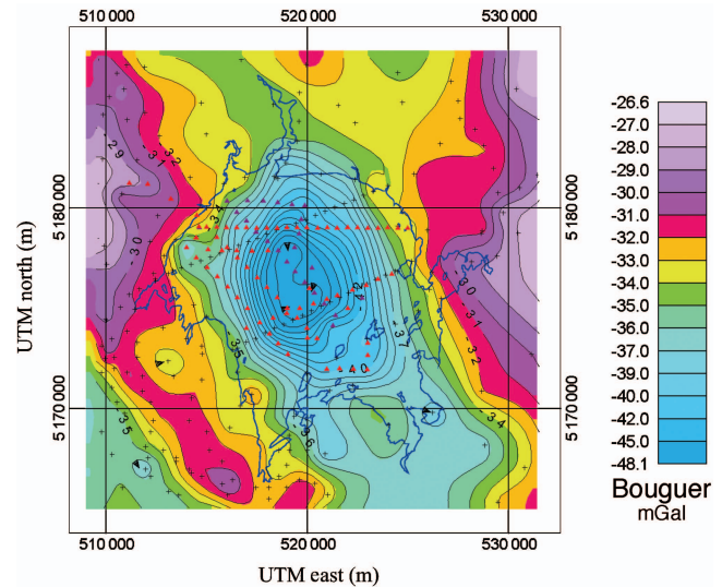
Figure 6. Bouguer gravity anomaly over Wanapitei Lake after compiling new and old data. Old gravity stations are shown as black crosses; new stations are red (2003) and blue (2004) triangles; lake outline is in blue. Contour interval is 1 mGal. Data are not terrain corrected.
