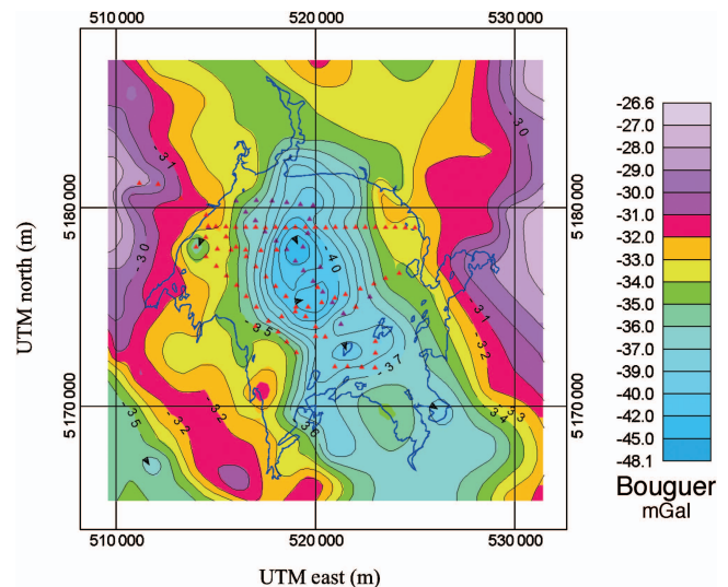
Figure 7. Compiled (1969, 2003, and 2004 data) and terrain-corrected Bouguer gravity anomaly over Wanapitei Lake. Old gravity stations are shown as black crosses, new gravity stations are shown as red triangles, and lake outline is in blue. Contour interval is 1 mGal. The amplitude of the anomaly is reduced to 7 mGal.
