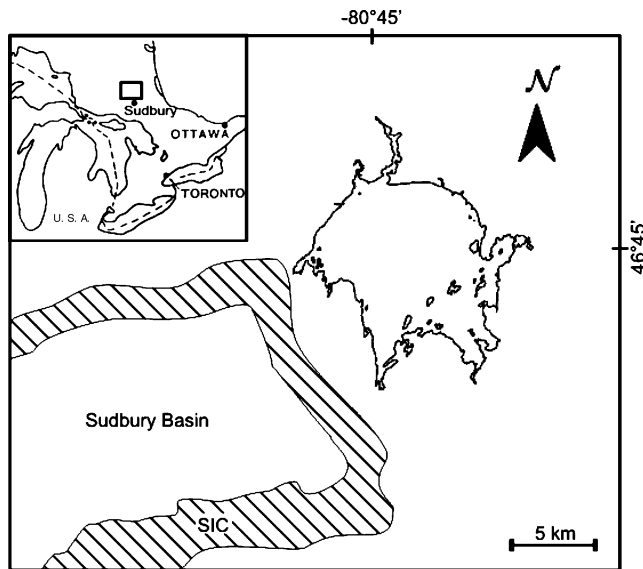
Figure 1. Lake Wanapitei location map. The square in the inset shows the location of the area of study in the detailed map. The eastern portion of the Sudbury Basin is shown for scale and location purposes. SIC is the Sudbury Igneous Complex.
