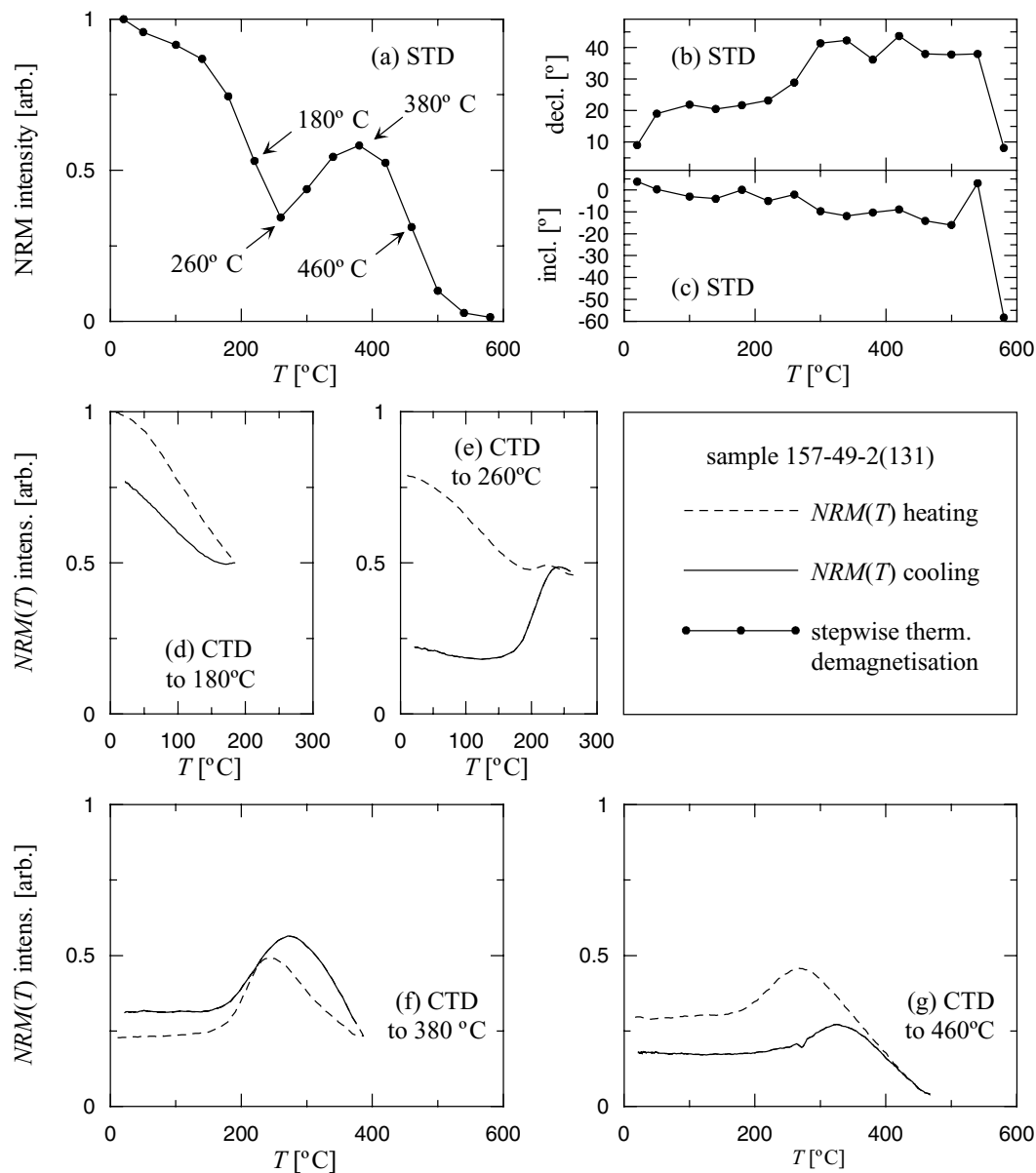
Figure 4. Stepwise (STD) and continuous (CTD) thermal demagnetization of sample 157 with self-reversal or partial self-reversal of NRM ( cf. figure caption of Fig. 2).
