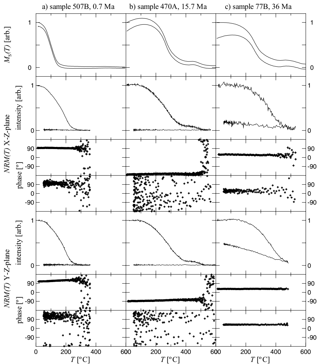
Figure 1. Comparison of strong field thermomagnetic curves M_S(T) with continuous thermal demagnetization NRM(T) of NRM for oceanic basalt samples 507B (a), 470A (b), 77B (c), 556 (d), 170 (e) and 550B (f). For M_S(T) a strong field thermomagnetic curve is given before (upper curve) and after (lower curve) correction for paramagnetism. NRM(T) is given for two perpendicular measurement planes (X-Z, Y-Z). All magnetizations in arbitrary units, the phase information (direction of magnetization within core coordinate X-Z or Y-Z-plane) is for arbitrary zero position. The phase information for a single NRM(T) curve is given in separate panels for the heating (crosses) and the cooling (diamonds) curve.
