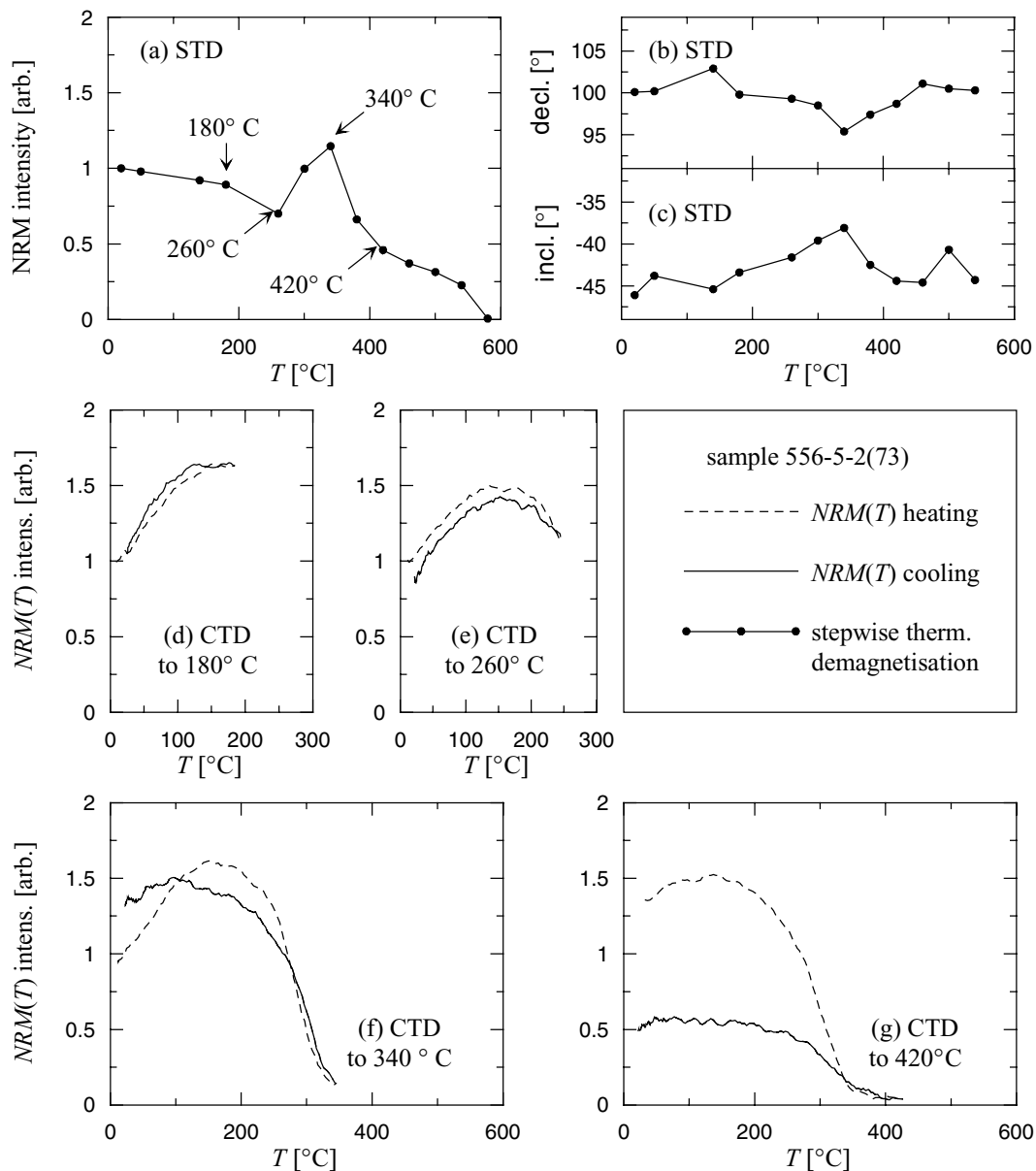
Figure 2. Stepwise (STD) and continuous (CTD) thermal demagnetization of sample 556. Intensity (a) and directional (b, c) information from STD. The CTD experiments in (d)–(g) with NRM(T) heating (dashed lines) and cooling (full lines) curves were performed to progressively higher maximum temperatures (also indicated by arrows in a).
