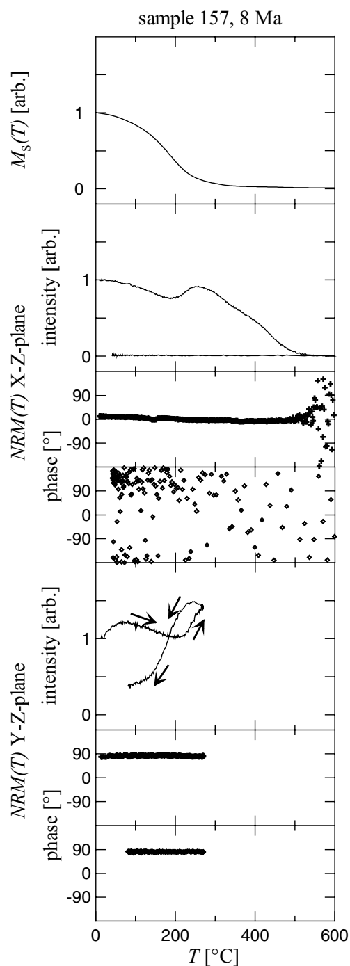
Figure 3. Comparison of strong field thermomagnetic curves M_S(T) with continuous thermal demagnetization NRM(T) for oceanic basalt sample 157 with self-reversal or partial self-reversal of NRM ( cf. figure caption of Fig. 1).
