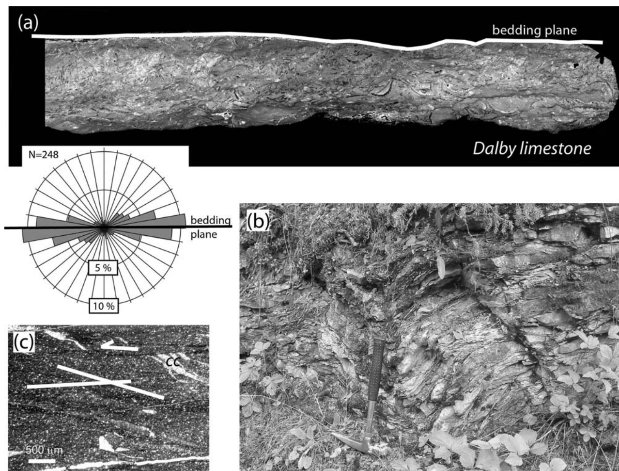
Fig. 10. a) Orientation analysis (rose diagram) of shells and elongated particles of Dalby limestone shows a shape-preferred orientation parallel to the bedding plane and suggests a primarily sub-horizontal deposition. The sample is from the Kraterstigen trail at the southern Tandsbyn syncline limb (Loc. II; Fig. 7). Inclination of bedding is 35°. b) Meter-scale fold in Dalby limestone (Loc. XIII; Fig. 7). The fold is exposed near the entrance of the Kraterstigen circuit. c) Microstructural analysis of slates of (b) revealed that folding resulted from tectonic deformation of solid rock, not from slumping in an unlithified state. Note the acute angle between bedding and slaty cleavage, localized shearing and strained calcite-bearing tension gashes (c).
