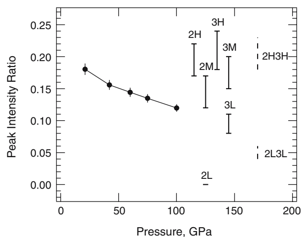
Fig. 3 Comparison between the observed and calculated intensity ratios between the \text{K}\beta' satellite peak at about 7.045 KeV ( I' ) and the \text{K}\beta_{1,3} main peak at about 7.058 KeV ( I ) in X-ray emission spectra of the Al-PV. Solid circles with error bars are experimental data (Li et al. 2004). Vertical lines and a bar shows the ranges or the value of intensity ratios calculated for various iron types, denoted by its valence state (2 = \text{Fe}^{2+} , 3 = \text{Fe}^{3+} ) and spin state (H high-spin, M intermediate-spin, L low-spin). The intensity ratio for each iron type is calculated according to I'/I = N/(N+2)/c , where N is the number of unpaired electrons in the incomplete 3d shell of iron, c is the empirical correction factor (Tsutsumi et al. 1976). The calculated ranges of intensity ratios reflect the range of values assigned to the correction factor c (between 3 and 4), arising from the uncertainty in the actual value of c for iron in the Al-PV and its possible variation with pressure, site occupancy, valence state, and spin state of iron. Dashed lines indicate the ranges of intensity ratios calculated for two possible spin states of iron in the Al-PV, by summing up contributions from all iron types according to I'/I = \sum (f_i \cdot N_i / (N_i + 2)) / c , where the subscript i refers to a specific iron type, f_i refers to the fraction of i , N_i refers to the number of unpaired electrons in type i . The fraction of \text{Fe}^{3+} is 53% (Table 1) and does not change with pressure (the apparent change is attributed to a possible spin crossover)
