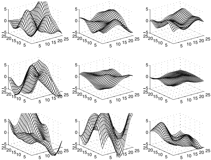
Figure 6. Realizations of T-distributed RFs with \nu = 1 .
