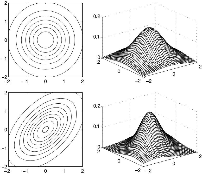
Figure 5. Upper: T_2(0, \Omega, 7) -distribution with unit variance and no correlation. Lower: T_2(0, \Omega, 7) -distribution with unit variance and correlation 0.5.
