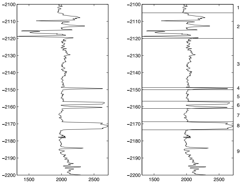
Figure 1. Left: Bulk density log from well C33 of the Gullfaks field in the North sea. Right: Layer interpretation of the log.
