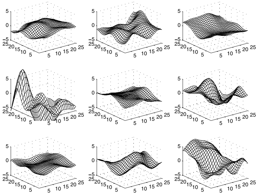
Figure 7. Realizations of T -distributed RFs with \nu = 3 .
