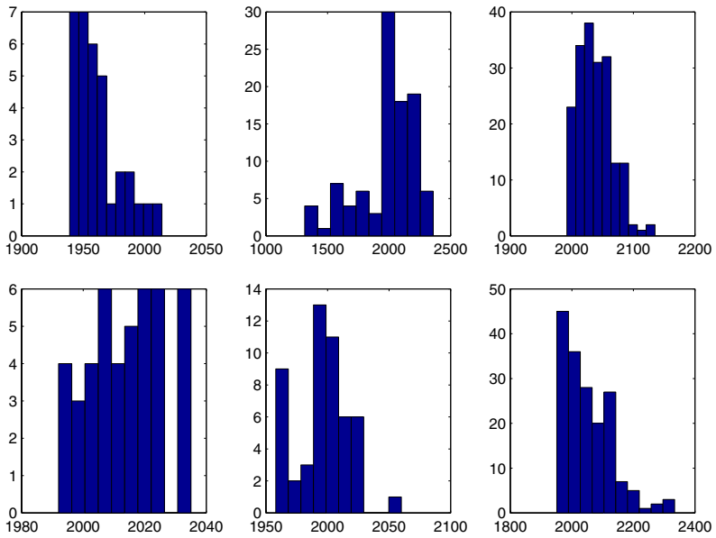
Figure 2. Histogram of density observations in each of the pooled layers. Upper: Layer 1,2,3. Lower: Layer 5,7,9.
