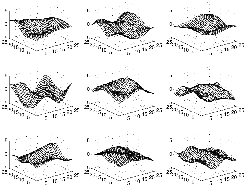
Figure 8. Realizations of T-distributed RFs with \nu = 5 .
