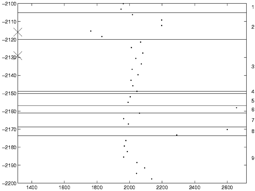
Figure 10. Bulk density log observations from well C33 from the Gullfaks field in the North sea with layer interpretation. The two locations to be predicted are marked (x).
