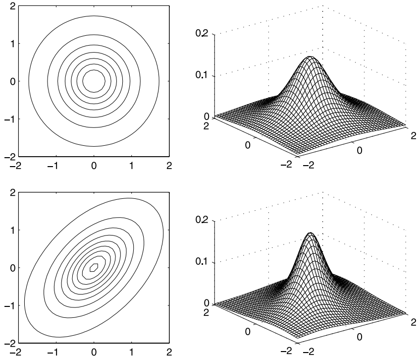
Figure 4. Upper: T_2(0, \Omega, 1) -distribution with unit variance and no correlation. Lower: T_2(0, \Omega, 1) -distribution with unit variance and correlation 0.5.
