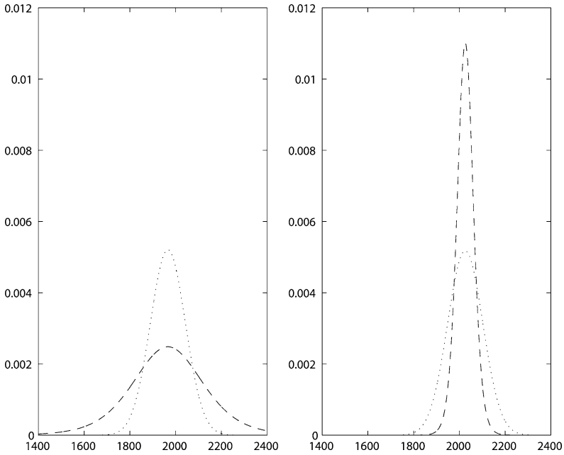
Figure 13. Prediction pdf based on the inferred Gaussian RF model (· · ·) and the inferred T-distributed RF model (— —) in layer 2 ( left ) and layer 3 ( right ).
