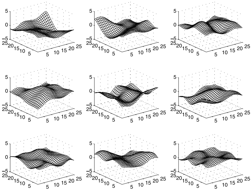
Figure 9. Realizations of T -distributed RFs with \nu = \infty , i.e. Gaussian RFs.
