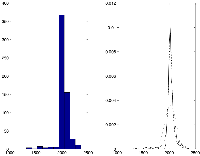
Figure 3. Left: Histogram of density observations in pooled layers. Right: Kernel estimate of pdf (—); Gaussian estimate of pdf (···); and Student-T estimate of pdf (---).
