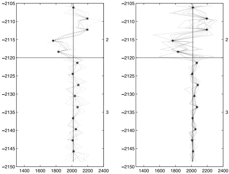
Figure 12. Left: Ten conditional realizations from the inferred Gaussian RF model. Right: Ten conditional realizations from the inferred T-distributed RF model.
