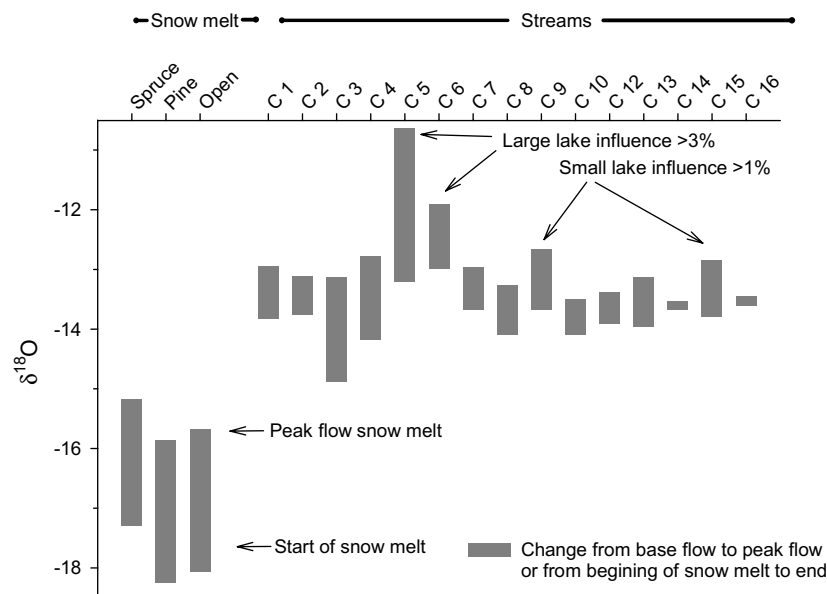
Figure 5 Change in \delta^{18}\text{O} signature during the spring flood, from baseflow to peak flow in the 15 streams and from beginning of snow melt to the termination of snow melt from lysimeters in three types of vegetation: closed canopy spruce forest, open canopy pine forest and open field. Note that the \delta^{18}\text{O} signal in snow melt water goes from light to heavy, whereas the opposite is true for the stream water.
