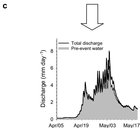
Figure 3 Evolution of event and pre-event water during the spring flood through the forested catchment soils, in C2 (a). A schematic view of the soil hydrological flow pathways during snow melt, where snow melt waters infiltrate through the topsoil because of permeable soil frost (grey ovals), raising the groundwater level into soil horizons of higher hydrologic conductivity which results in more rapid lateral flow (b). The resulting stream spring hydrograph in the forested catchment is dominated by pre-event water (c).
