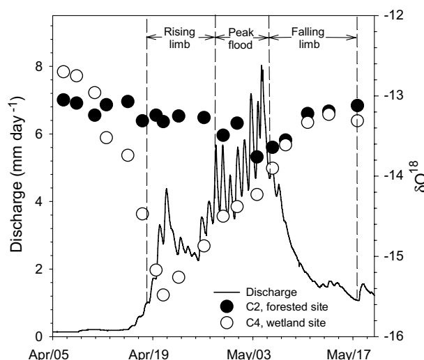
Figure 2 Spring flood discharge at catchment, C7, defining the rising limb, peak flood and falling limb periods as used in this study. Oxygen-18 ( \delta^{18}\text{O} ) values for catchments C2 and C4 are shown.
