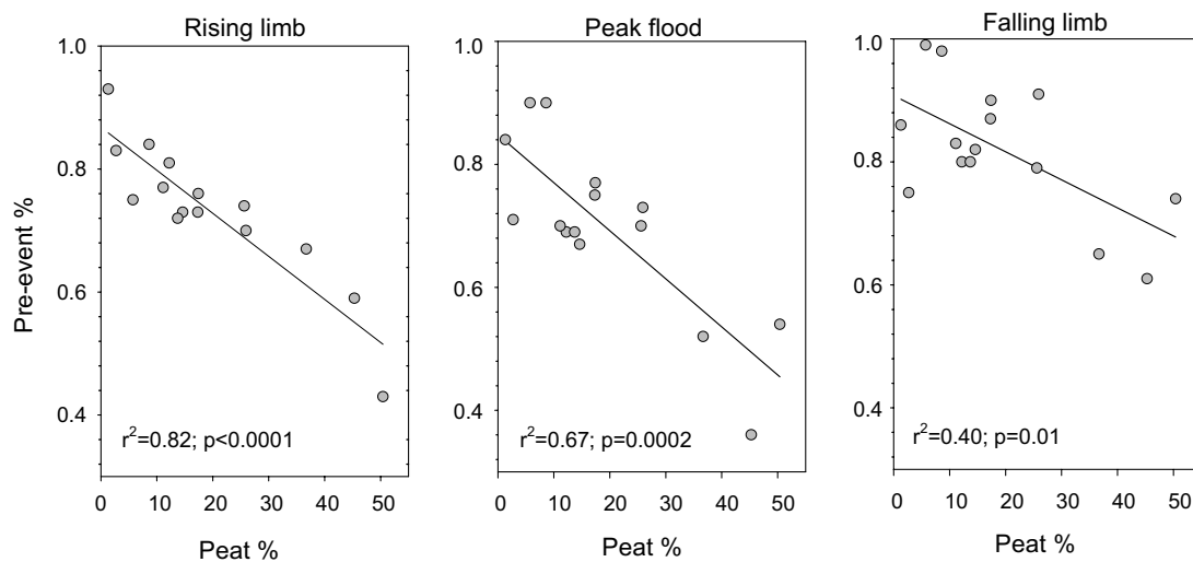
Figure 6 Correlation between peat percent coverage and pre-event water fraction during rising limb, peak flood, and falling limb.
