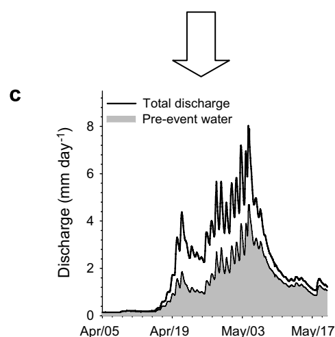
Figure 4 Evolution of event and pre-event water during the spring flood through the wetland peat, in catchment C4 (a). A schematic view of the subsurface hydrological flow pathways where snow melt waters cannot infiltrate the soil because of impermeable soil frost (grey rectangles) and instead runoff as overland flow or through preferential flow pathways (b). The resulting stream spring hydrograph in the wetland catchment has similar proportions of event and pre-event water (c).
