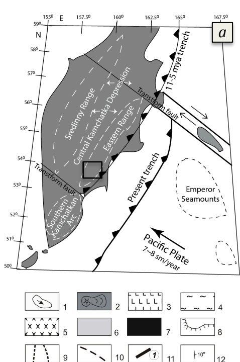
Fig. 1 a) General plate tectonic position of the Kamchatka and location of the Verhnevachinskaya caldera (black square).
