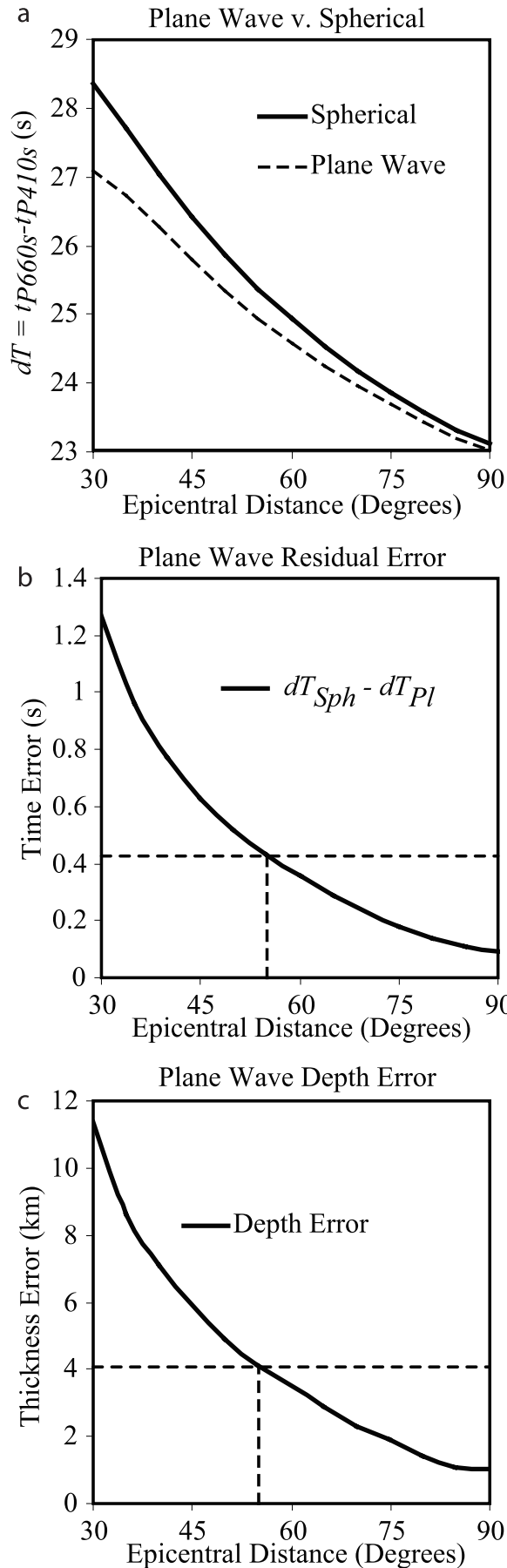
Figure 10. The plane wave approximation underestimates the (a) theoretical time delay between Pds and P , resulting in an over estimation of the (b) time delay anomaly and (c) transition zone thickness anomaly. The reference slowness used by Chevrot et al. [1999] corresponds to the depth error marked by the dashed line (4 km).
