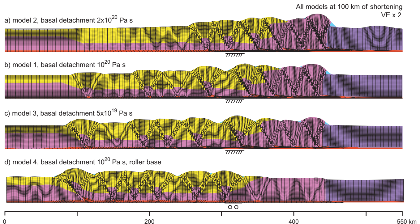
Figure 7. The propagation of deformation through the models is to a large degree influenced by the level of decoupling at the base of the upper crust. (a–c) Models 1–3 illustrate the sensitivity to the viscosity value of the basal detachment. (d) Model 4 with a roller basal boundary condition (free horizontal movement) shows efficient transfer of shortening through the basin. The models are shown at 100 km of shortening. Vertical exaggeration is 2.
