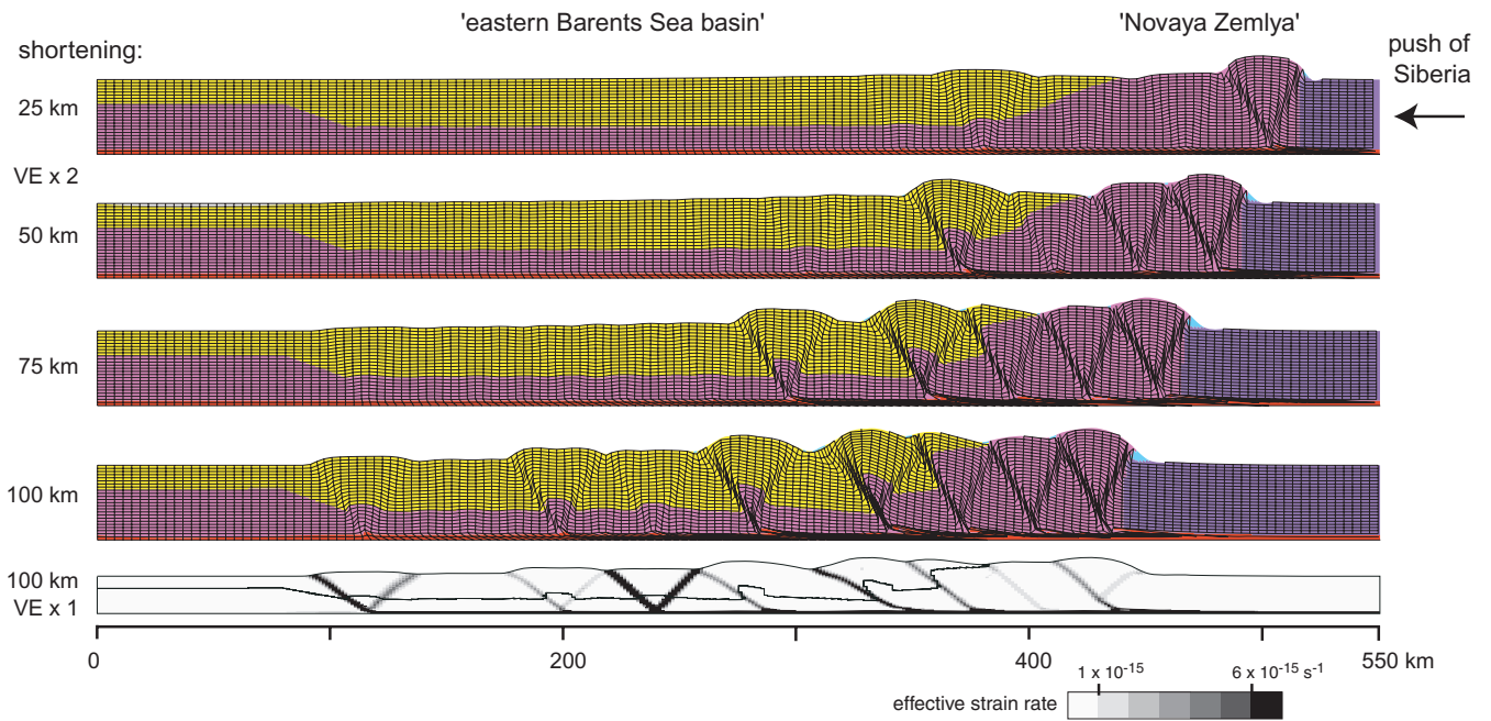
Figure 6. Evolution of reference model 1. The total amount of shortening is indicated at the left-hand side of the models. Shear-zones and fault-bend-folds develop in the frictional-plastic basin sediments and underlying crust due to the basinward movement of a strong crustal block over a linear-viscous detachment (viscosity 10^{20} Pa s). The grid is a Lagrangian tracking grid of which every 8th line in the horizontal and vertical direction is shown. The model setup is shown in Fig. 5a. Vertical exaggeration is 2 (except for bottom figure).
