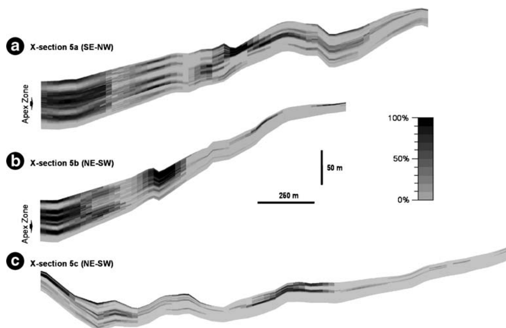
Fig. 5 a–c Sections across the axial alluvial fan deposits showing probability of sand facies occurrence resulting from the interpolation of the indicator variable. See location of these sections in Fig. 2a and compare to the facies model in Fig. 8a, where the same sections are shown. Vertical exaggeration is \times 3
