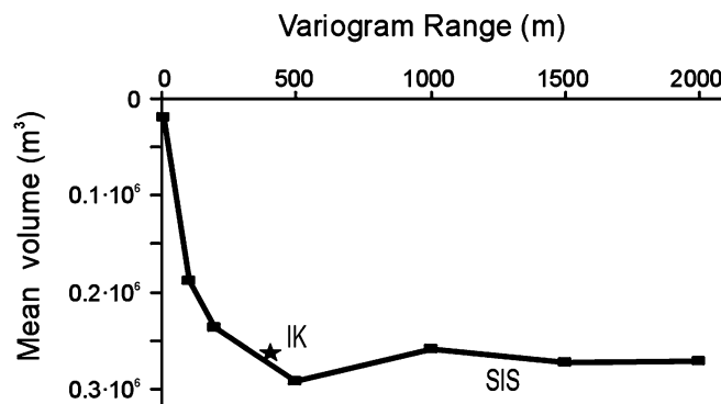
Fig. 7 Test comparing the mean sand body volume obtained from IK using the fitted variogram ( star ), and SIS varying horizontal variogram ranges ( line ) for the axial alluvial fan in interval 13A. Mean sand body volumes from 10 realizations were averaged to obtain each SIS mean volume in order to average ergodic fluctuations (fluctuations of results from diverse simulations built on the same initial parameters). Vertical variogram ranges and proportions in SIS were kept constant, equal to those used for IK. Only bodies with volumes exceeding 11,300\text{ m}^3 were averaged, because smaller bodies will correspond in most cases to ribbons
