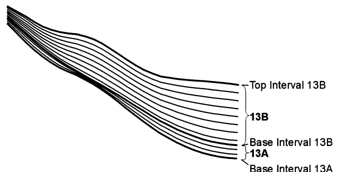
Fig. 4 Detail of a vertical section showing the proportional grid layering style in the two reconstructed sub-grids. Note that only one-tenth of the grid layers are shown
