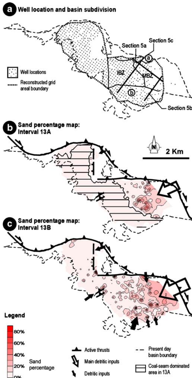
Fig. 2 a Well location in sequence 13 (note regular spacing), and subdivision of the eastern subbasin area according to sand deposition patterns: a) alluvial fans attached to the northern, tectonically active margin; b) alluvial fans fed from the southern inactive margin; (MBZ) marginal basin zone; (IBZ) inner basin zone. Position of sections in Figs. 5 and 8a is also shown. b, c Sand percentage maps for the intervals 13A and 13B. Arrows show the main alluvial feeding points of coarse-grained facies, with the largest ones corresponding to the axial alluvial fan. Active structures during sedimentation of the sequence 13 are based on Ferrús (1998) and Santanach et al. (2005). The coal-seam dominated area in interval 13A is also shown; the boundary encloses the area where coal percentage exceeds 60%. See location of the basin in Fig. 1b
