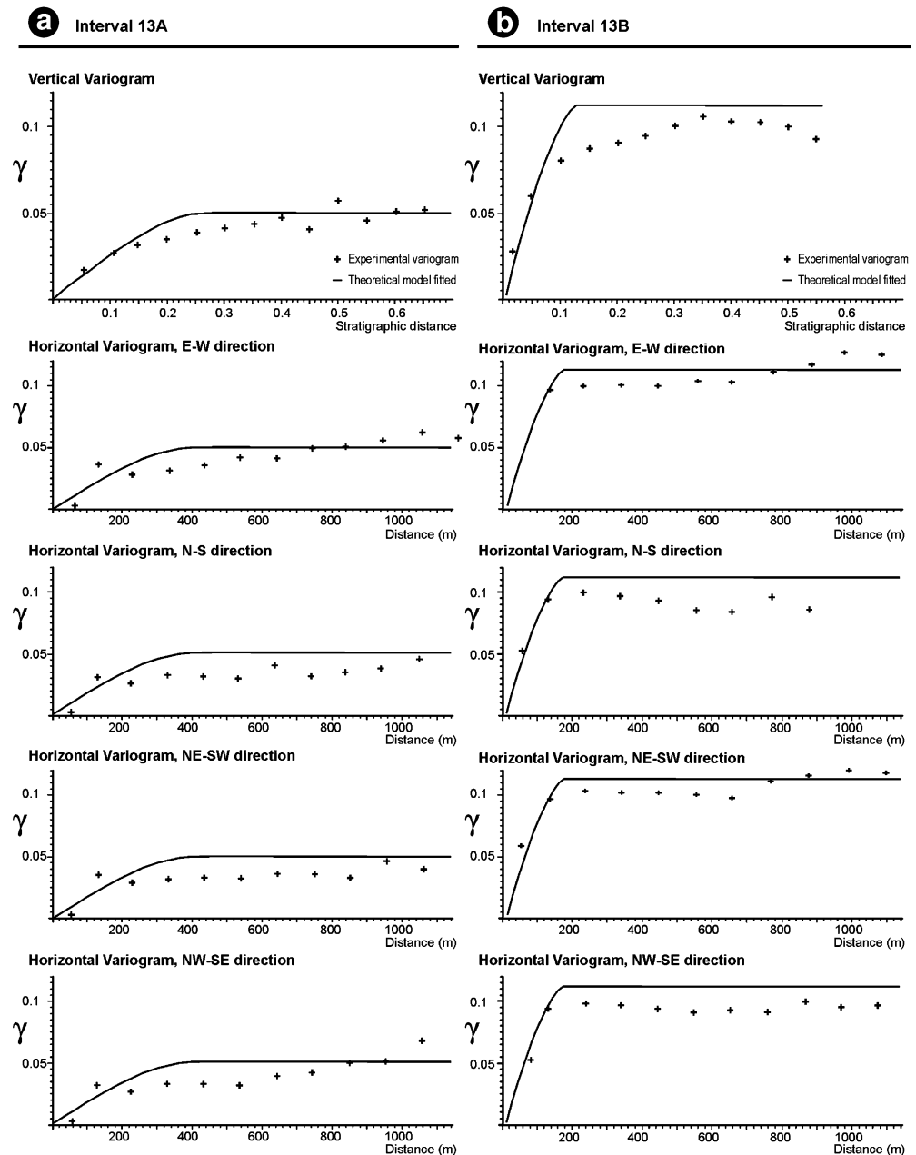
Fig. 6 Indicator variograms for sand facies in the axial alluvial fan for intervals 13A and 13B. Experimental variograms were computed using the logs up-scaled to the size of grid cells. Horizontal experimental variograms were computed by considering pairs of points belonging to the same grid layer, and with a tolerance angle of 45° and a bandwidth of 300m for each direction. Vertical variograms were computed by considering only pairs of points in the same well. Theoretical variogram models were fitted assuming spherical models (see ranges in Table 1). Because a proportional grid was used, with variable vertical spacing, vertical variogram distances are expressed in fractions of grid thickness
