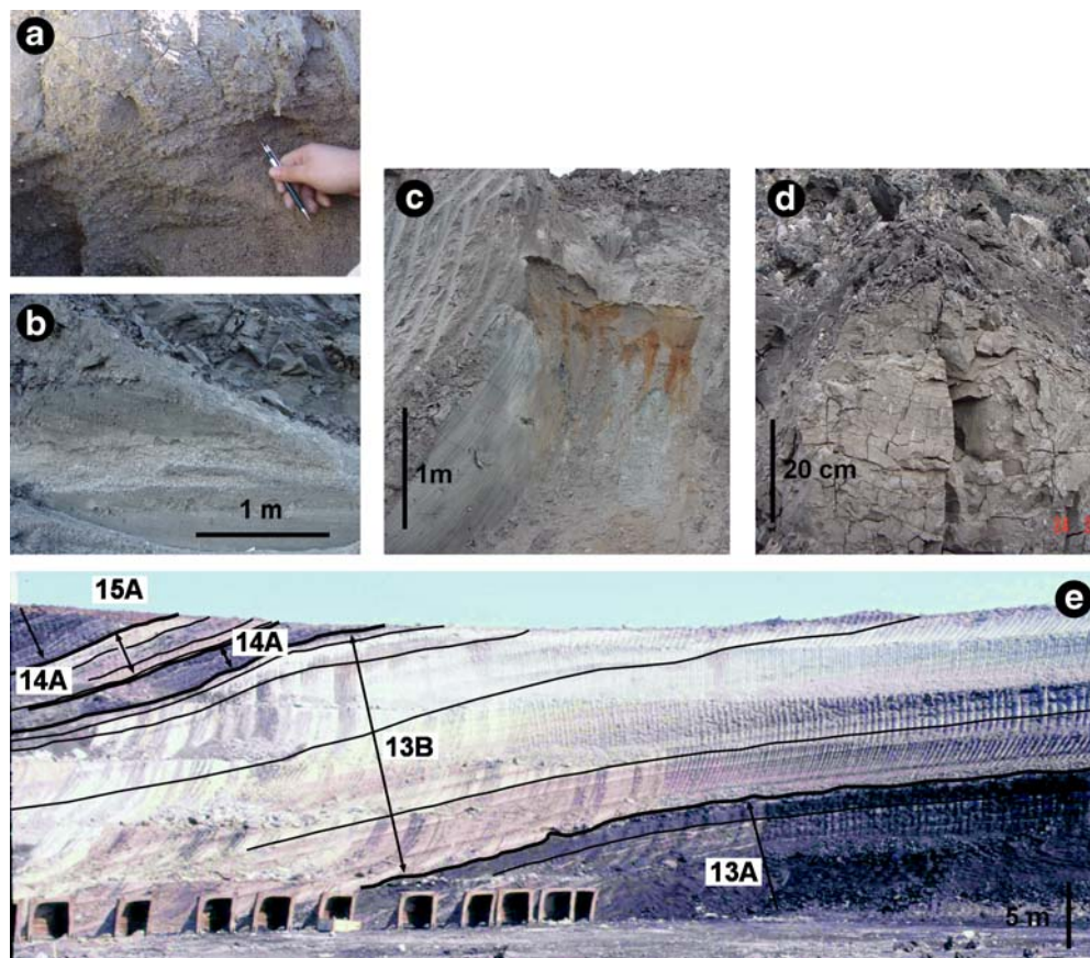
Fig. 3 Facies examples from the open-pit mining trenches in the basin. a Poorly sorted, massive to cross-laminated sands, corresponding to a laterally extensive sand body in the medial part of the axial alluvial fan. b Well-sorted ribbon sand lens embedded within brown coal facies in the inner basin zones, and accumulated by the distributive fluvial network. c Mudstones. d Dark brown coal facies. e Example of an open-pit mining trench showing sequence 13 in the inner basin zone
