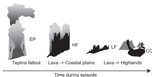
Fig. 2. Sketches representing the eruptive phases distinguished in this study: EP, explosive; HF, high fountaining; LF, low fountaining; CO, cone building. Transitions from one phase to another were gradational.
