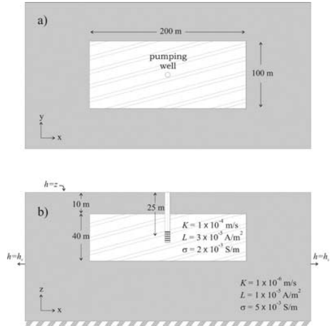
Figure 10. Heterogeneous half-space with pumping well: (a) model in plan view, showing outline of subsurface aquifer; (b) model in cross-section, showing hydraulic boundary conditions and physical properties of aquifer and half-space. Well screen length is 10 m.
