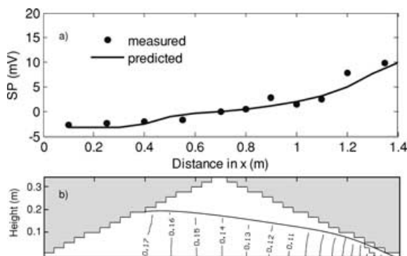
Figure 7. Homogeneous embankment subject to steady-state seepage from an 18 cm reservoir: (a) Measured and predicted SP data at surface and (b) predicted hydraulic head distribution (m).
