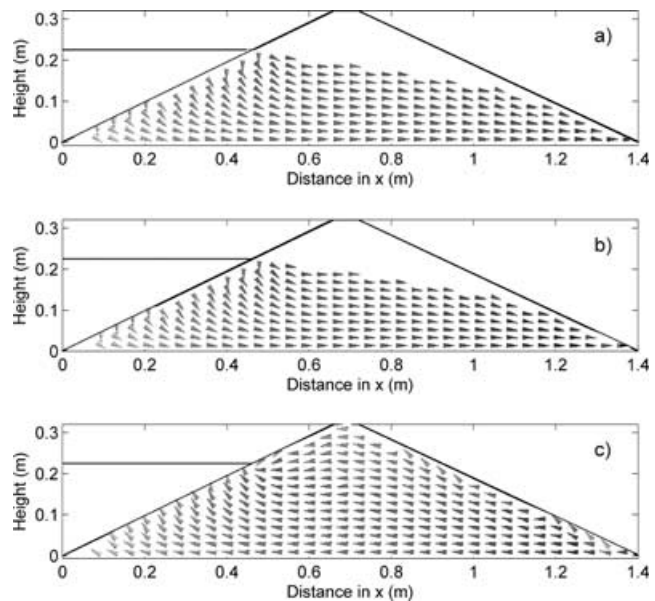
Figure 9. Homogeneous embankment subject to steady-state seepage from a 22.5 cm reservoir: (a) fluid flux q ; (b) streaming current and (c) conduction current J .
