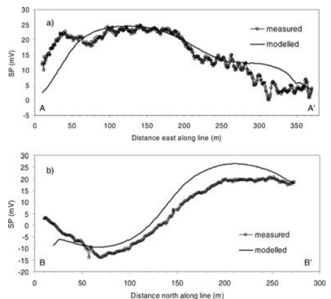
Figure 17. Embankment subject to seepage from the reservoir at high pool: (a) Measured and predicted SP data at the surface of the reservoir above the diversion dam (survey line A-A') and (b) Measured and predicted SP data at the surface of the reservoir in a N-S direction across the grout curtain (survey line B-B').
