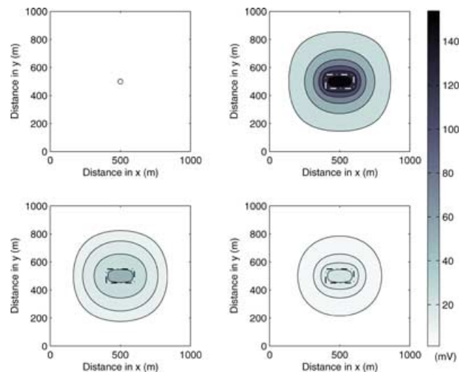
Figure 13. Surface plan map of SP: (a) homogeneous half-space; (b) heterogeneous K half-space; (c) heterogeneous K and L half-space and (d) heterogeneous K , L and \sigma half-space.
