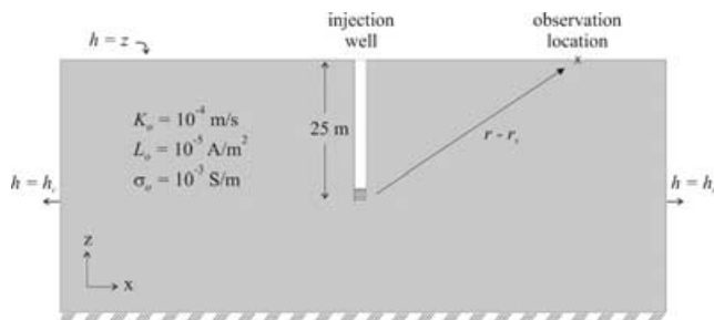
Figure 3. Homogeneous half-space model with injection well showing hydraulic boundary conditions and physical properties of aquifer.
