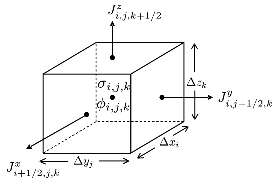
Figure 2. Single grid cell showing cell dimensions, location of components of current density \mathbf{J} at cell faces, and location of potential \phi and conductivity \sigma at the cell centre.
