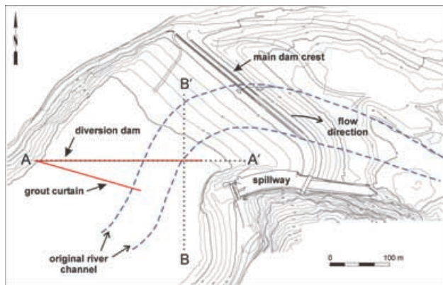
Figure 15. Plan map of the embankment dam site, indicating key structural features and survey lines A-A' and B-B'.
