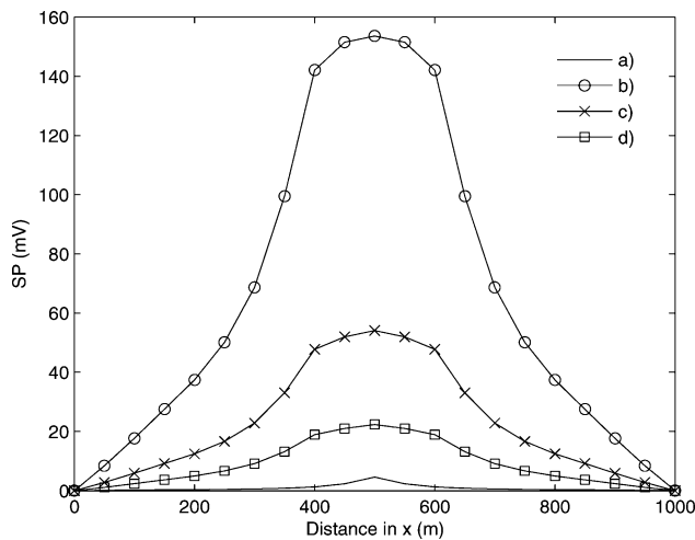
Figure 14. Surface profiles of SP at y = 500 m: (a) homogeneous half-space; (b) heterogeneous K half-space; (c) heterogeneous K and L half-space and (d) heterogeneous K , L and \sigma half-space.
