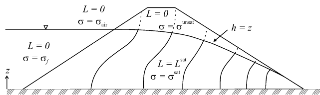
Figure 6. Schematic cross-section of a homogeneous earth embankment, illustrating the distribution of electrical properties. Hydraulic head equipotential lines are indicated in the figure, with dotted lines representing hydraulic head in the unsaturated zone. Superscripts sat and unsat refer to representative properties of the saturated and unsaturated zones, respectively. The value \sigma_f represents the electrical conductivity of the impounded water. The value \sigma_{\text{air}} is typically chosen as 1 \times 10^{-8} \text{ S m}^{-1} .
