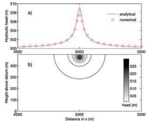
Figure 4. Hydraulic head distribution resulting from a point injection well in a homogeneous half-space: (a) analytical and numerical solutions at surface and (b) predicted head contours (1 m interval).
