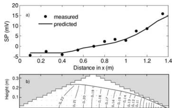
Figure 8. Homogeneous embankment subject to steady-state seepage from a 22.5 cm reservoir: (a) Measured and predicted SP data at surface and (b) predicted hydraulic head distribution (m).
