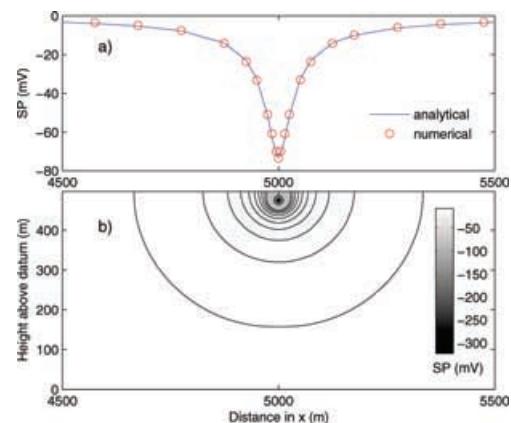
Figure 5. SP distribution resulting from a point injection well in a homogeneous half-space: (a) analytical and numerical solutions at surface and (b) predicted SP contours (5 mV interval).
