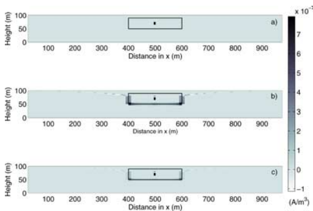
Figure 12. Vertical cross-section of streaming current source density in the plane of the pumping well: (a) homogeneous half-space; (b) heterogeneous K half-space and (c) heterogeneous K and L half-space. The total magnitude of primary streaming current sources at the well screen is 7.8 \times 10^{-6} \text{ A m}^{-3} .
