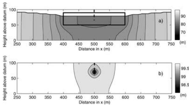
Figure 11. Vertical cross-section of hydraulic head in the plane of the pumping well: (a) heterogeneous half-space model; (b) homogeneous half-space ( K = 1 \times 10^{-4} \text{ m s}^{-1} ) for comparison.
