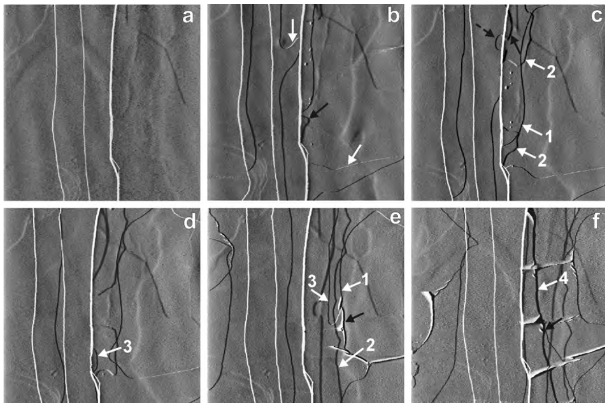
Figure 1. Ion-exchange reaction \text{K}^+ \rightarrow octylammonium at 20^\circ\text{C} : (a) pristine phlogopite surface with cleavage steps; (b) 41 min after the start of octylammonium solution flow ( i.e. 41 min after the first image); the exchange reaction between \text{K}^+ and organic ions causes the formation of swelling fronts (height \approx 18 \text{ \AA} ); (c–f) 94, 158, 262 and 568 min after the first image: the arrows with labels indicate the different locations of the reaction fronts within the respective interlayers; front ‘4’ is \sim 100 \text{ \AA} in height. Phlogopite No. 1, scan size 8.8 \mu\text{m} \times 8.8 \mu\text{m} .
