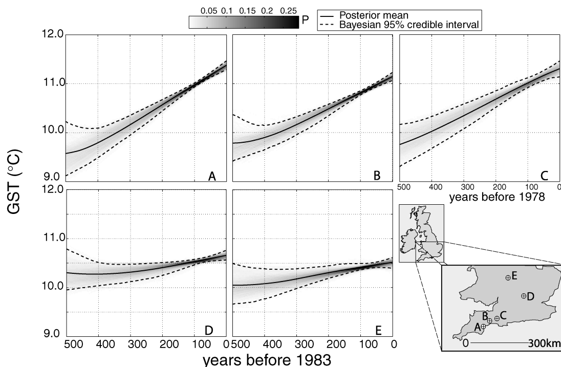
Figure 7. Posterior probability distributions for the individually inverted boreholes. The locations of these are shown in the inset map, and the details are given in Table 1.
