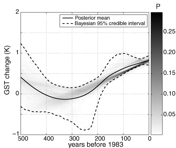
Figure 8. Posterior probability distribution for the simultaneous inversion of the five boreholes shown as deviations from the steady state.
