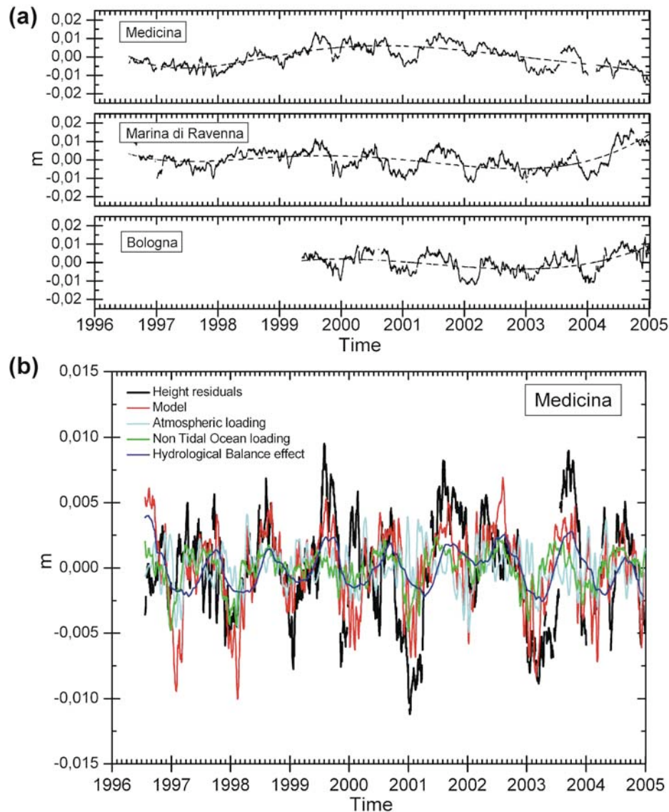
Figure 2. (a) GPS seasonal and long-term oscillations (continuous black line); linear trends have been subtracted. The nonlinear long-term signal present in the Medicina and Marina di Ravenna series has been approximated by fitting a fifth-order polynomial, while for Bologna, a third-order polynomial was used (dashed lines). (b) Observed GPS height seasonal oscillations (black line) at the Medicina station together with the seasonal model (red line) obtained by summing the air pressure (light blue line) and nontidal ocean loading (green line) as well as the effect of hydrology (blue line). The nonlinear long-term signal and the linear trend have been subtracted.
