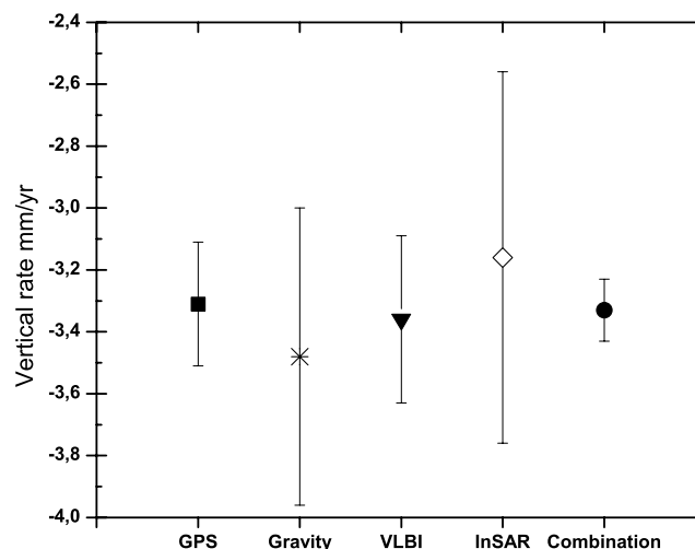
Figure 12. Different vertical rates estimated at Medicina from the various techniques. The combined solution (dot) is also presented.
