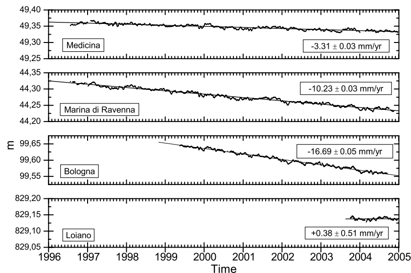
Figure 3. GPS long-term trends. They have been estimated by removing the long-term signal and the modeled seasonal oscillations from the daily height time series for the Medicina, Marina di Ravenna, and Bologna stations.
