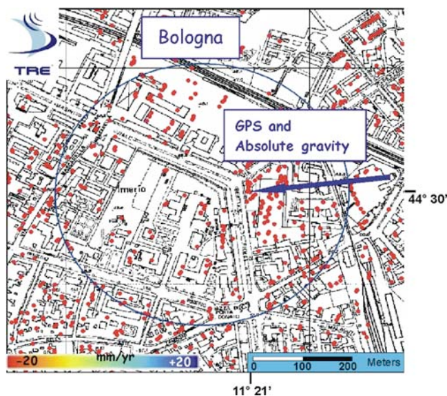
Figure 6. Sector of the city of Bologna showing the large amount of PSs available, the remarkable subsidence rate, and the location of the GPS and absolute gravity station.
