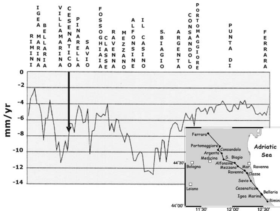
Figure 8. Estimate of subsidence rates along a line from Rimini to Ferrara from high-precision leveling data acquired in the period 1990–1999 [after Benedetti et al. , 2000]. The location of the leveling line is shown in the lower right corner.
