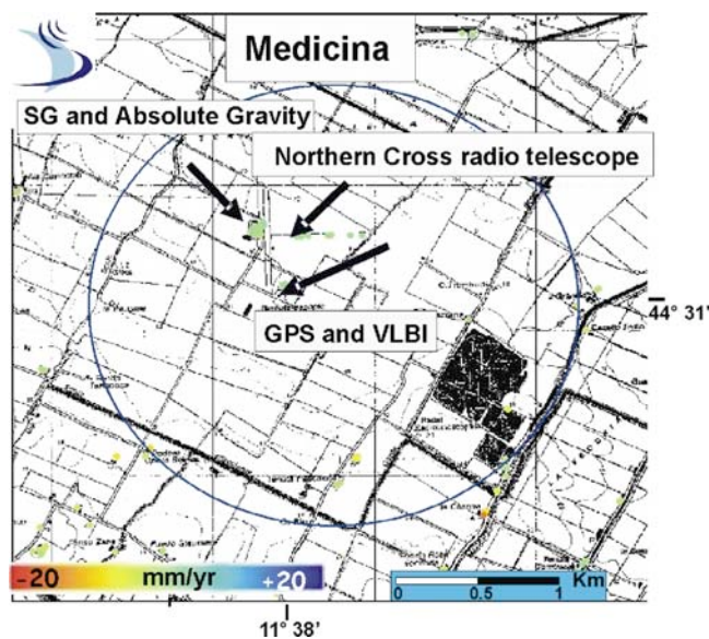
Figure 5. The Medicina station area. The image shows a limited number of PSs because this is a rural environment.
