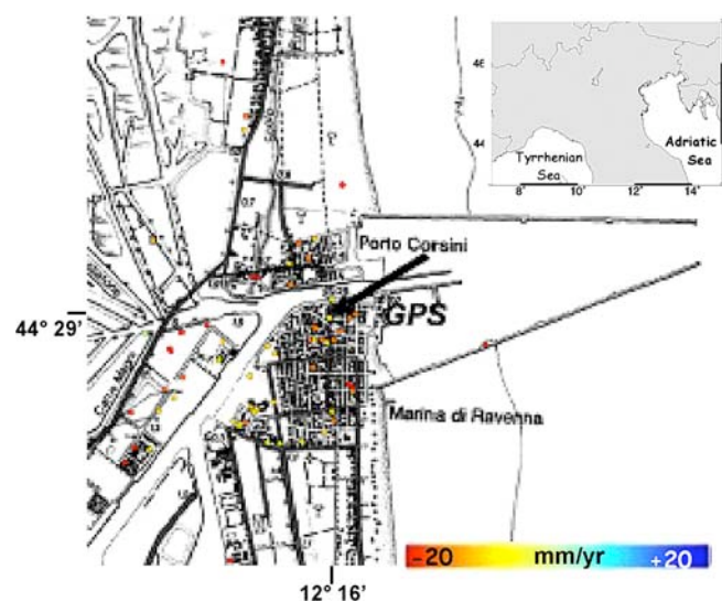
Figure 7. Distribution of PSs in the Marina di Ravenna area, relevant subsidence rates, and location of the GPS station. The location of the SAR images is shown in the right upper corner.
