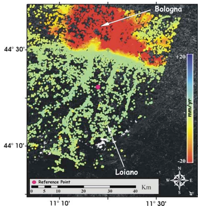
Figure 9. The Bologna and Loiano areas. The image shows the large amount of PSs available and the relevant vertical rates. The magenta dot identifies the location of the reference point for the InSAR data analysis.
