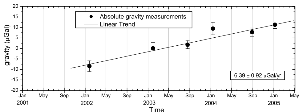
Figure 11. Bologna station. Series of six absolute gravity measurements (dots) and linear trend.
