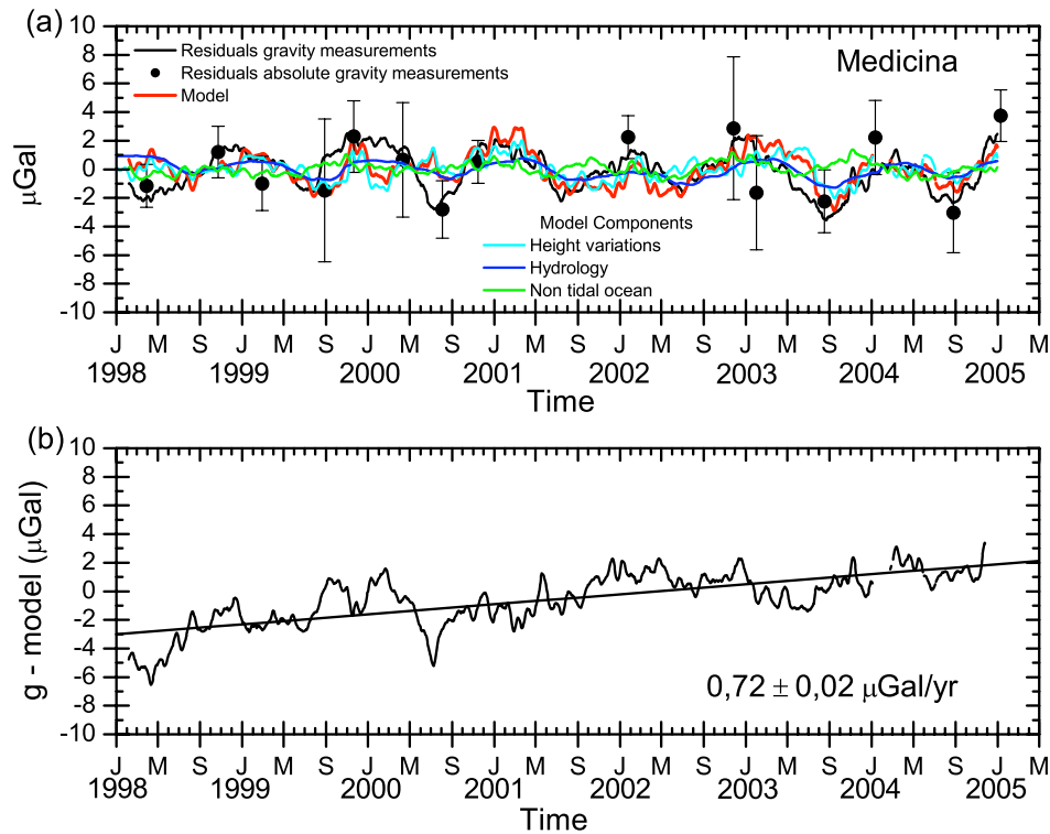
Figure 10. (a) Observed gravity seasonal oscillations (black line) and absolute gravity FG5 measurements (black dots), both detrended. The seasonal model is represented by the red line. The model is the sum of the gravimetrical contributions due to height variations (light blue line), nontidal oceanic effect (green line), and local hydrology (blue line). (b) Estimate of the long-term trend. The seasonal model has been removed from the time series before estimating the long-term trend.
