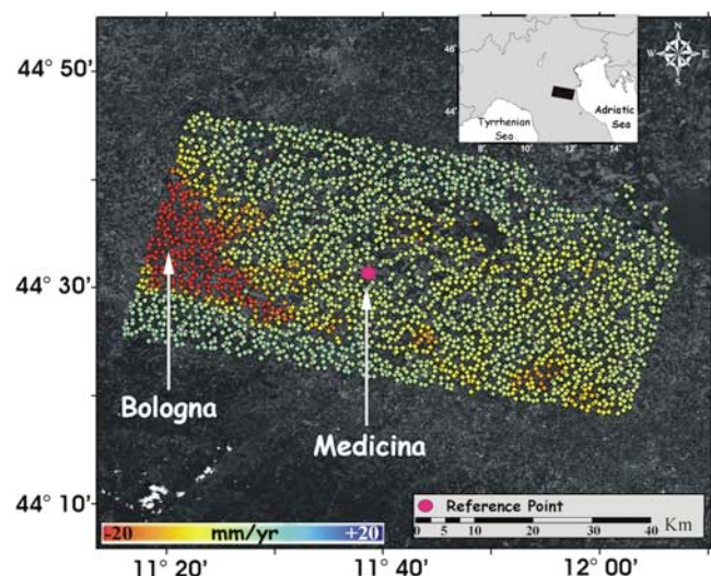
Figure 4. The ensemble of PSs available in the Bologna and Medicina area and the relevant vertical rates. The magenta dot identifies the location of the reference point for the InSAR data analysis. The location of the SAR images is shown in the right upper corner.
