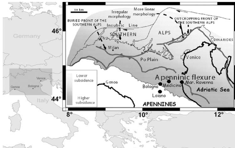
Figure 1. Distribution of natural subsidence rates in northeastern Italy [after Carminati et al. , 2003] and location of the permanent GPS stations (black dots). Except for the Loiano site, which is on the uplifting and extensional belt of the Apennines, the other three stations are located in the area of the Po Plain where natural subsidence is highest. Bologna and Medicina are in the southern Po Plain, close to the Pede-Apenninic margin, while Marina di Ravenna lies on the easternmost coastal Plain on the Adriatic Sea at the very front of the Apennines' accretion prism [ Doglioni , 1993].
