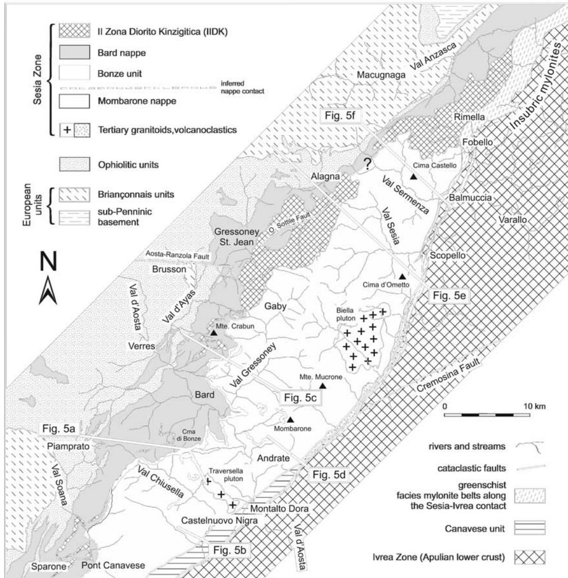
Figure 2. Lithotectonic map of the Sesia Zone and adjacent units. Map shows tectonic subdivision of the Sesia basement (Mombarone, Bard, and IIDK nappes), Mesozoic metasediments (Bonze and Canavese units), and the location of cross sections in Figure 5.
