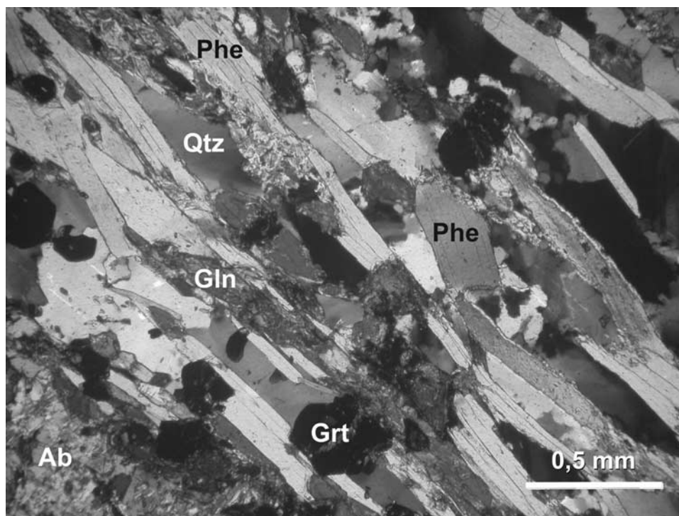
Figure 8. Microstructural relationship between zoned D2 glaucophanes and phengites. Rb-Sr phengite-feldspar isochron yields a younger age limit for D2 Chiusella shearing of ~64 Ma (see Appendix A). Sample MK52, location, Val Chiusella; H, 5043395; R, 396392 (referred to Gauss-Boaga net).
