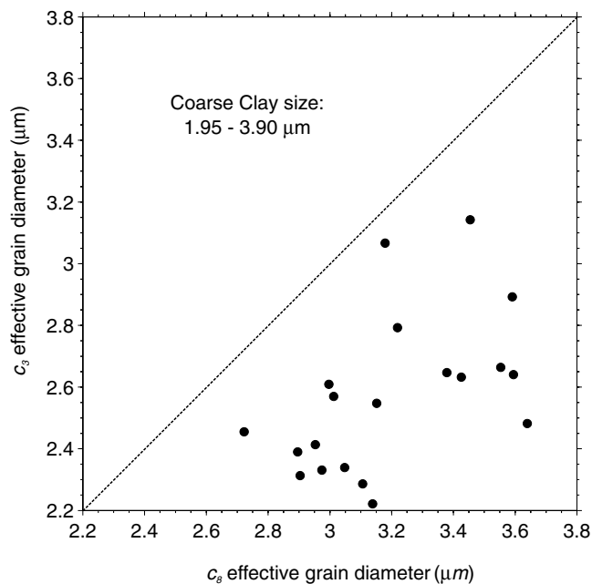
Figure 13. Using eq. (1) to determine effective particle size for the low c_8 and high c_3 concentration suspensions reveals that the small magnetic particles appear to be attached to larger sediment grains in the size range of coarse clay.
