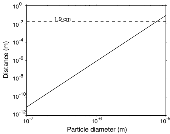
Figure 4. For sediment particles descending through the sample cube ( \sim 1.9 cm in height) it is important to consider the relative magnitudes of the times required for descent and randomization by Brownian motion. By determining the distance travelled by a particle moving at terminal velocity in time \tau it is clear that full randomization should occur for all but the very largest magnetic sediment particles.
