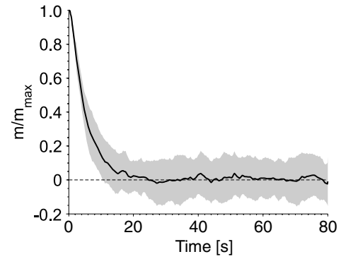
Figure 8. Individual runs of the numerical model consisting of 20 particles. For each configuration, 50 runs were calculated with the particles in different initial positions. The final decay curve for a given configuration was obtained by stacking the 50 runs (arithmetic mean, shown as the black line) and determining their standard deviation at each time point (shaded area). It can be seen that at some points the magnetization becomes negative, however, the magnitude of the negative value is substantially smaller than the standard deviation of the signal.
