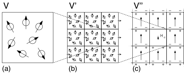
Figure 7. The n particles that are simulated are situated inside the centre box V of a cube V' consisting of 27 boxes. The other 26 boxes contain shifted images of the centre box. This should account for more realistic conditions while simulating the experiment, since the number of particles that can be handled at once is rather small. The large black arrows in (c) denote the average magnetization within each box. H_d is the demagnetizing field.
