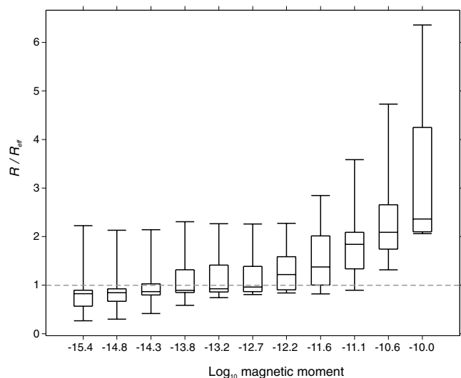
Figure 9. A box and whisker plot showing the distribution of R/R_{\text{eff}} as a function of particle magnetic moment. The lower and upper lines of the 'box' are the 25th and 75th percentiles of the sample. The distance between the top and bottom of the box is, therefore, the interquartile range. The line in the middle of the box is the sample median. If the median is not centred in the box, that is an indication of skewness. The 'whiskers' are lines extending above and below the box showing the extent of the rest of the results. The dashed grey line marks R/R_{\text{eff}} = 1 which is where the model result is expected to occur for a suspension with no magnetostatic interactions and no particle-particle collisions. The clear shift to R/R_{\text{eff}} > 1 for high particle moments demonstrates the effect of magnetostatic interactions increasing the magnetization decay rate.
