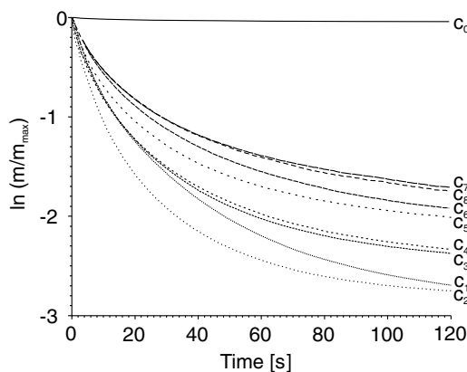
Figure 5. Experimental magnetic relaxation data for a typical sediment sample. The natural logarithm of the decay of nine different suspension concentrations is plotted against time. The highest concentration ( c_0 ) acts as a slurry and shows only a small decrease in magnetization while the other suspensions relax far more quickly. If the decay curves were exponential then when plotted as the natural logarithm they would appear as straight lines. This is clearly not the case for the suspension samples.
