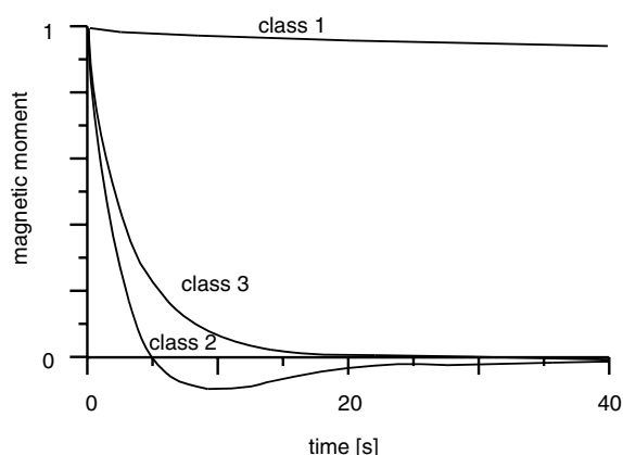
Figure 1. Experimental results of Yoshida & Katsura (1985), using a sediment suspension consisting mainly of reddish-brown clay, show three different classes of magnetic relaxation pattern. Class 1 and Class 2 are attributed to electrostatic and magnetostatic interactions within the sediment suspension, respectively. Class 3 is thought to represent a non-interacting system that is dominated by Brownian motion.
