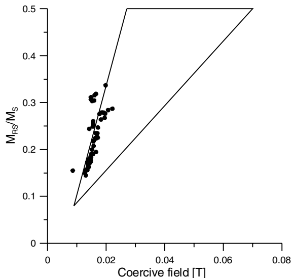
Figure 2. Ratio of saturation remanent magnetization to saturation magnetization ( M_{RS}/M_S ) plotted against the coercive field. According to Tauxe et al. (2002), data that plot within the triangle can be considered to represent mixtures of single domain magnetite particles and superparamagnetic material. The samples plot along the left edge of the triangle, which, according to Tauxe et al. (2002), corresponds to a mixture containing uniaxial single domain magnetite with a length to width ratio of 1.3.
