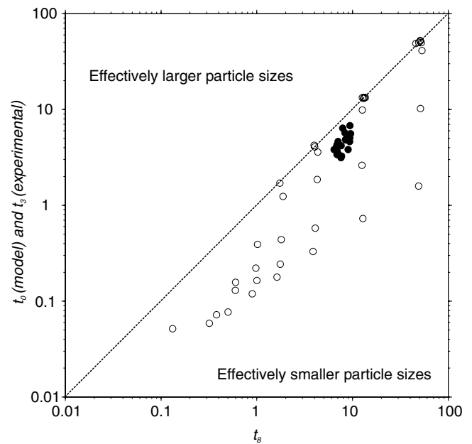
Figure 12. A comparison of the characteristic magnetization decay times for the numerical simulations (open symbols) reveals a difference in the effective particle size of low- and high-concentration systems. Points below the line of unity indicate a more rapid decay in the high-concentration system, demonstrating the effect of magnetostatic interactions. When plotted in the same space, the results of the laboratory experiments (closed symbols) show similar behaviour, which provides evidence for the presence of significant magnetostatic interactions in the prepared sediment suspensions.
