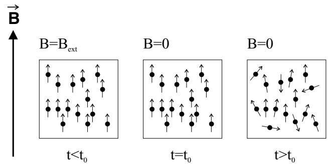
Figure 3. When a sediment suspension is exposed to a magnetic field for 30 s, the particles align with the external field. At time t = t_0 , the field is switched off and measurement of the magnetization commences. The decay of magnetization is recorded as a function of time for 120 s.
