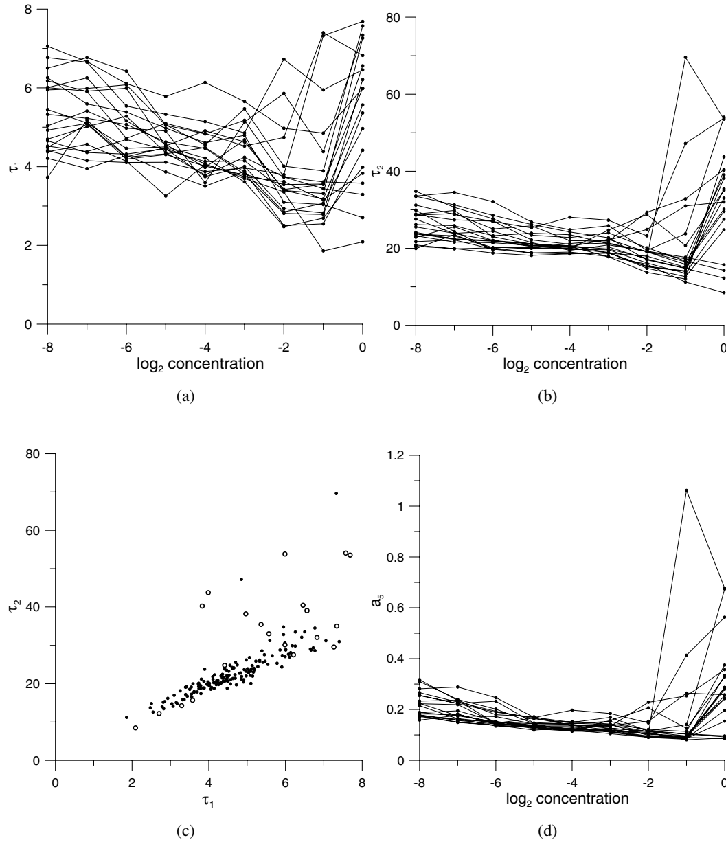
Figure 6. (a) Relaxation time \tau_1 plotted against a \log_2 based concentration. Out of 20 samples, 16 displayed a significant decrease in relaxation time moving from low to high concentrations and an increase in relaxation time moving from second highest to highest concentration. From left to right, the data points represent concentrations c_8 through to c_0 . (b) Relaxation time \tau_2 plotted against a \log_2 based concentration. Out of 20 samples, 15 displayed a significant decrease in relaxation time moving from low to high concentrations and an increase in relaxation time moving from second highest to highest concentration. (c) Relaxation time \tau_1 plotted against relaxation time \tau_2 . The samples display an apparently linear relationship between \tau_1 and \tau_2 . The majority of samples that do not follow the trend correspond to the highest concentration suspensions that show little decrease in magnetization (open symbols). (d) Constant a_5 plotted against a \log_2 based concentration. There is a sharp increase in a_5 moving from the second highest ( c_1 ) to the highest ( c_0 ) concentration. This increase can be attributed to increased flocculation of magnetic and non-magnetic particles resulting in locking of the magnetic particles.
