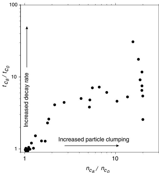
Figure 11. A number of the model systems demonstrate particle clumping, producing ratios of n_{c_8}/n_{c_0} (the number of particles remaining in the lowest concentration assemblage divided by the number of particles remaining in the highest concentration assemblage) greater than 1. Each simulation consisted of 20 particles, therefore, n_{c_8}/n_{c_0} can take a maximum value of 20. It is also apparent that the magnetization decay time for low-concentration assemblages is longer than for their high-concentration counterparts ( t_{c_8}/t_{c_0} > 1 ). The monotonically increasing relationship between the particle and time ratios shows that increased suspension concentration results in greater particle clumping, which in turn reduces magnetization decay time.
