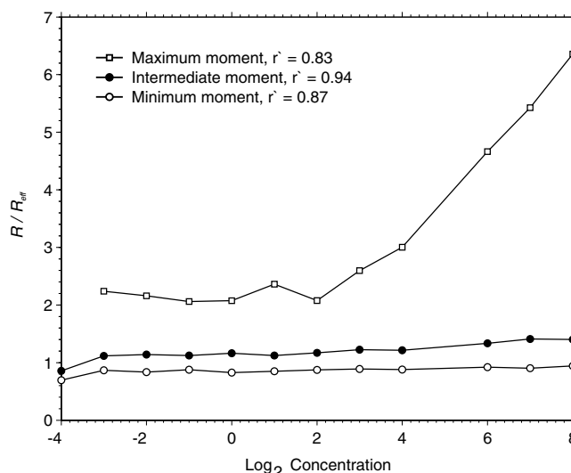
Figure 10. The ratio R/R_{\text{eff}} shows a significant monotonic increase, indicating increased magnetization decay rate, as a function of suspension concentration. The overall effect is slight in the systems with low and intermediate magnetic moments, demonstrating the weak effect of the magnetostatic interactions. In contrast, a strong effect is observed in the high moment system once a threshold concentration of 4 ppm is passed. The Spearman rank correlation coefficient of each line is given by r' .
