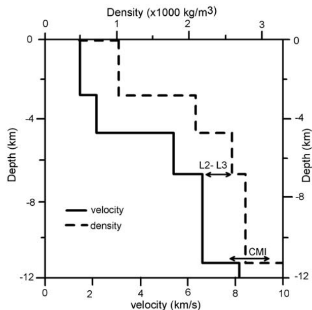
FIGURE 5 | Velocity-depth structure obtained by King et al. (1997) with the estimated densities via Nafe and Drake's relationship (in Grant and West, 1965, p. 200). Positions of the L2-L3 discontinuity, as well as the CMI are depicted (arrows), as reported by King et al. (1997).
