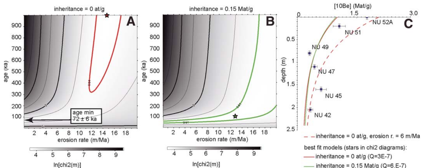
Figure 12. Results of the ^{10}\text{Be} analysis on surface S1 in Noyan Uul. A and B: Plots of the results of the chi-square inversion. Stars represent the best-fit solutions, and colored curve defines the associated 1\sigma uncertainties. The inversion gives a minimum age of 72 \pm 6 ka for the model with no inheritance and 50 \pm 8 ka for the model with 0.15 M atoms/g of inheritance. C: Plot of the ^{10}\text{Be} concentration of the samples along the depth profile and best-fit theoretical models issued from the chi-square inversion.
