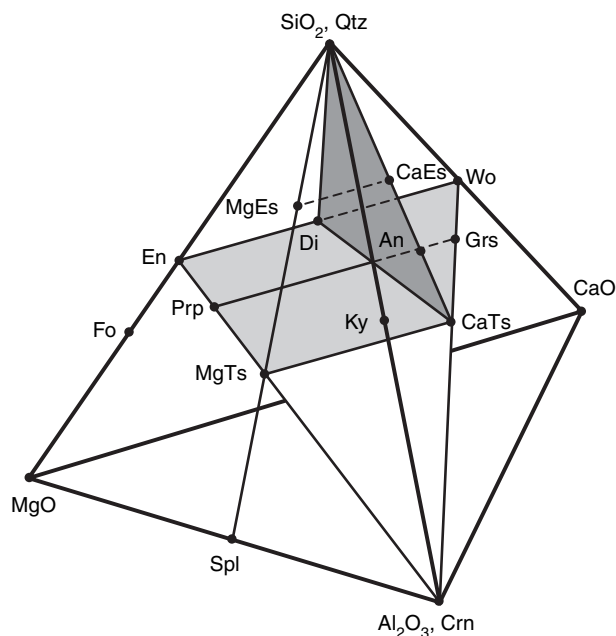
Fig. 1. Compositions in the system CaO-MgO-Al 2 O 3 -SiO 2 (CMAS). All formula units and abbreviations are listed in Table 1. The joins Di-CaTs, Prp-Grs, and MgTs-CaTs lie in the plane En-Wo-Crn.
