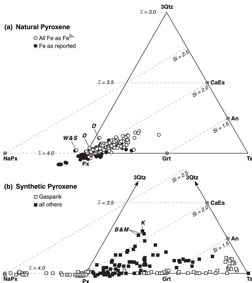
Fig. 3. Natural and synthetic pyroxene compositions in condensed oxide space. (a) Natural pyroxene. Filled circles: analyses with Fe as reported; open circles: all Fe calculated as \text{Fe}_2\text{O}_3 . W&S indicates the sample reported by Wang & Sueno (1996). D indicates two of the samples summarized by Deer et al. (1978) (b) Pyroxene compositions synthesized in NCMAS. Open squares: Gasparik (1984a,b, 1985a,b, 1989, 1996). Closed squares: All others (Kushiro, 1969; Bell & Mao, 1971; Khanukhova et al. , 1976a,b, 1977; Wood & Henderson, 1978; Wood, 1979). B&M: Bell & Mao, 1971. K: Khanukhova et al. , 1976b). Contours of Si and \Sigma as in Fig. 2. Contours of Ca, Mg and Al are no longer possible because of the projection. Uncertainties ( \pm 2\sigma ) for standard microprobe analyses are probably about one or two times the size of the symbols. The plotting coordinates in terms of cations per six oxygen are: 3\text{Qtz} = 0.33(\text{Si} + \text{Ti} - \text{Fe}^{2+} - \text{Mn} - \text{Ni} - \text{Mg} - \text{Ca}) - 0.67(\text{Na} + \text{K}) ; \text{Ts} = \text{Ti} + 0.5(\text{Al} + \text{Cr} + \text{Fe}^{3+} - \text{Na} - \text{K}) ; \text{Px} = -\text{Ti} - 0.25(\text{Al} + \text{Cr} + \text{Fe}^{3+}) + 0.5(\text{Fe}^{2+} + \text{Mn} + \text{Ni} + \text{Mg} + \text{Ca}) + 1.25(\text{Na} + \text{K}) (Table A2).
