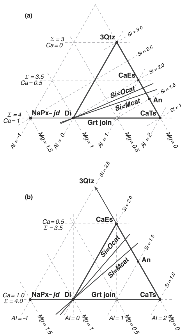
Fig. 2. Two coordinate systems for pyroxene compositions in CMAS. (a) Di-CaTs-3Qtz. (b) Di-CaTs-CaEs; abbreviations in Table 1. Dashed lines are contours of constant cation content and 'Σ' is total cations (per six-oxygen formula unit). The point labelled 'Grt join' marks the piercing point of the Prp-Grs join (Fig. 1). 'Ocat' is the sum of all cations excluding Si. 'Mcat' is the sum of M-site cations, excluding Si. The Si = Ocat line intersects the CaTs-3Qtz and CaTs-CaEs joins at X_{\text{CaTs}} = 0.6 and 0.2 respectively. The Si = Mcat line intersects these joins at X_{\text{CaTs}} = 0.66 and 0.33 respectively. See text for further discussion.
