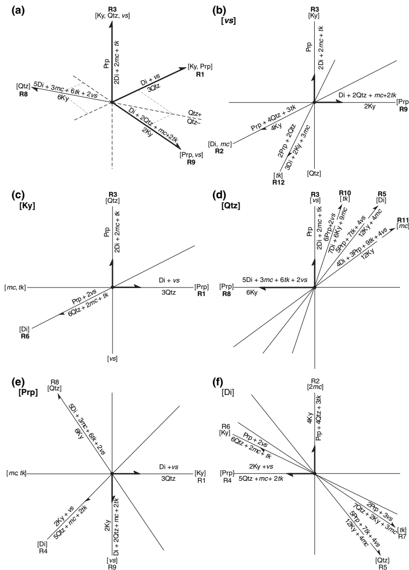
Fig. 4. Reaction space for eclogite in CMAS. All reactions among phase components are positive as written in Table 2. Basis vectors are shown as heavy arrows with arbitrary unit lengths and are positive in the direction shown by arrows. Reactants written on same side of reaction as arrowhead. Components written in square brackets are conserved in the labelled reaction. The component written in the top left of each figure is conserved in all reactions in that plane. (a) Basis vectors in the three-dimensional reaction space. Reaction R8 is a Qtz-conservative reaction that lies in the R1–R9 plane. Reactions R8 and R3 define a Qtz-conservative plane that separates Qtz-producing and Qtz-consuming half-spaces. All linear combinations of the basis vectors that pass behind this plane produce Qtz; those that pass in front consume Qtz. All subsequent diagrams illustrate a plane in the reaction space. (b) R3–R9 plane. Contains all [vs] reactions. (c) R3–R1 plane. Contains all [Ky] reactions. (d) R3–R8 plane. Contains all [Qtz] reactions. (e) R1–R9 plane. Contains all [Prp] reactions. (f) R2–R4 plane. Contains all [Di] reactions.
