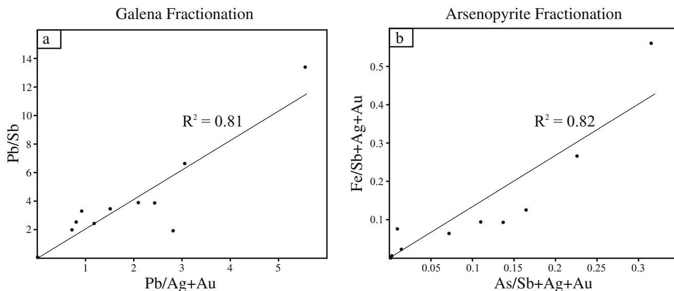
Fig. 4 Fractionation of the Pb–As–Sb–Ag–Au–S melt at Montauban. a Fractionation of through galena crystallisation. b Fractionation of through arsenopyrite crystallisation
