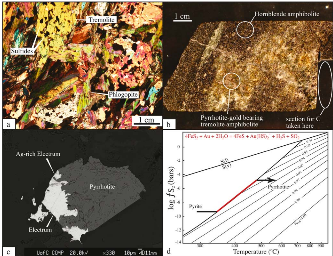
Fig. 2 Pre- to syn-peak metamorphic hydrothermal alteration of amphibolite and consequent sulphidation in the wall rock at Montauban. a Photomicrograph showing tremolite–phlogopite alteration in detail. b Drill core showing dark coloured hornblende being replaced by tremolite + pyrrhotite. Note the position from which a thin
