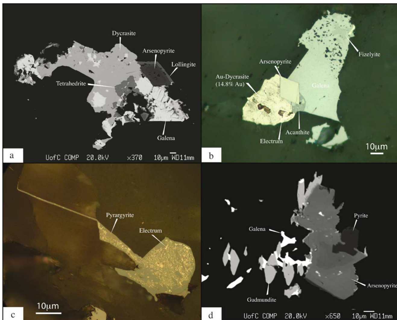
Fig. 3 Textures and mineral associations resulting from sulphide melt remobilisation at Montauban. a and b Minerals crystallised from stage 1 melt. c Pyrargyrite and electrum in part of a stage 2 sulphide melt
