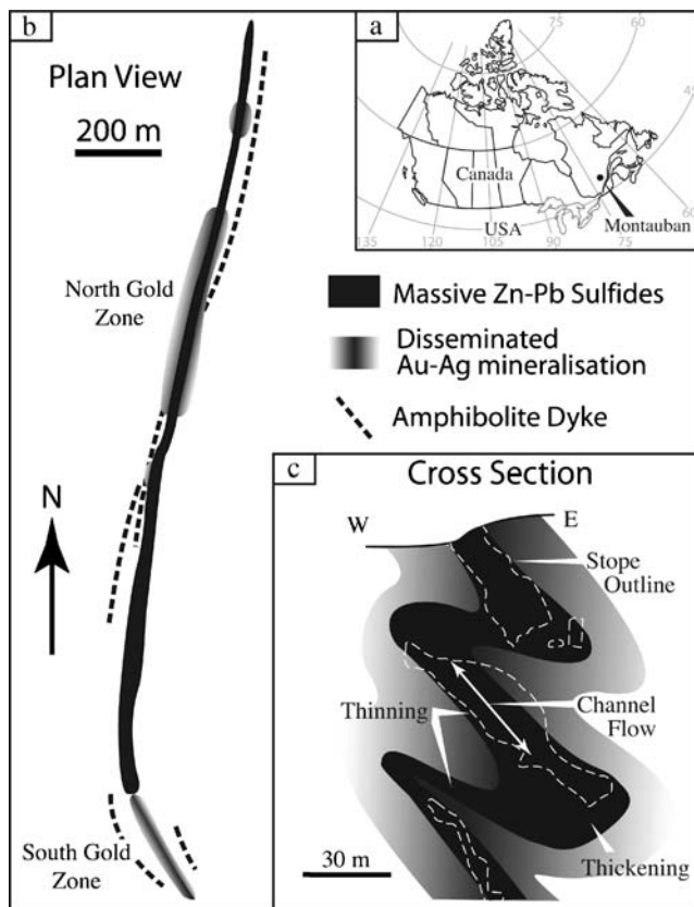
Fig. 1 a Location of the Montauban deposit. b Plan view of the deposit showing the projected to surface geometry of the ore body (modified from Bernier et al. 1987; Jourdain 1993). c Schematic cross-section highlighting the pre-mining morphology of the massive sulphides. The position of a late cross-cutting mafic dyke has been removed to estimate the original morphology. Modified from Jourdain (1993)
