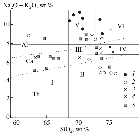
Fig. 4. (Na_2O + K_2O) vs. SiO_2 diagram. (1–4) Acid rocks with positive Eu anomalies: (1, 2) vein granite: (1) potassic, (2) sodic; (3, 4) blastomylonite: (3) potassic, (4) sodic; (5) host rocks. (I) Tonalite; (II) plagiogranite, (III) granite, (IV) leucogranite; (V) subalkaline granite, (VI) subalkaline leucogranite. Compositional fields of granitoid series: Al—alkaline, Ca—calc-alkaline, Th—tholeiitic (after [12]).
