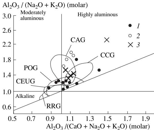
Fig. 3. Al_2O_3/(Na_2O + K_2O) vs. Al_2O_3/(CaO + Na_2O + K_2O) diagram for (1) potassic granite, (2) sodic granite, and (3) blastomylonite. Compositional fields of granites from various geodynamic environments (after [11]): CAG—continental arc granites, CCG—continental collisional granites, RRG—rift-related granites, POG—postorogenic granites, CEUG—continental epeirogenic granites.
