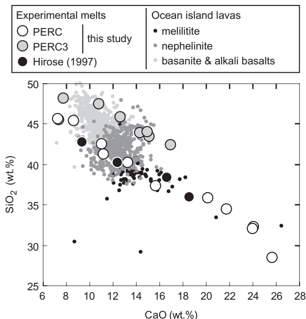
Fig. 9. Normalized CaO (wt.%) vs SiO 2 (wt.%) for silicate partial melts of carbonated peridotite from this study and from Hirose (1997) compared with those of melilitites, nephelinites, basanites, and alkali basalts from oceanic islands (GEOROC database: http://georoc.mpch-mainz.gwdg.de/georoc/ ). The CaO–SiO 2 trend for partial melts from PERC3 is distinct from those of PERC and Hirose (1997), which suggests that CaO–SiO 2 relations depend on the bulk CO 2 concentration of peridotite sources.
