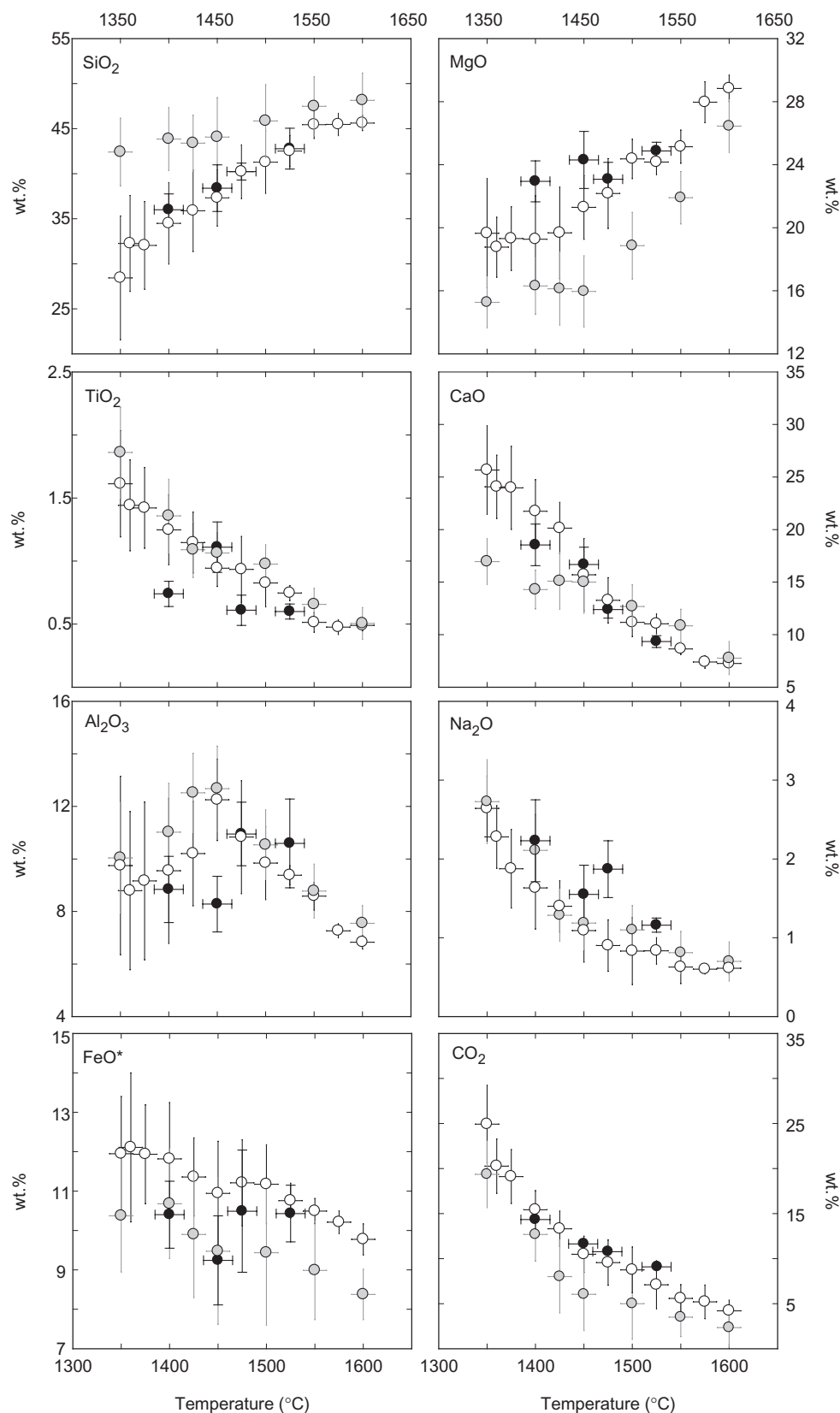
Fig. 3. Composition of carbonate-bearing silicate partial melts from PERC (white circles) and PERC3 (grey circles) carbonated peridotite partial melting experiments at 3 GPa. Concentrations of \text{SiO}_2 , \text{TiO}_2 , \text{Al}_2\text{O}_3 , \text{FeO}^* , \text{MgO} , \text{CaO} , and \text{Na}_2\text{O} are calculated on a volatile-free basis and that of \text{CO}_2 is derived by the difference between 100% and the average total from replicate electron microprobe analyses. Also included for comparison are carbonated silicate partial melt compositions from the study of Hirose (1997) (●). Concentrations of \text{CO}_2 in the experiments of Hirose (1997) are estimated from bulk \text{CO}_2 in the experiments and estimates of melt fractions. The latter are estimated from mass balance for experiments at 1400 and 1525°C, where mineral phases are reported, and by linear interpolation of these melt fractions vs temperature for experiments at 1450 and 1475°C. Error bars in temperature are \pm 12^\circ\text{C} and \pm 15^\circ\text{C} for this study and Hirose (1997) respectively and for composition \pm 1\sigma (wt.%) for both studies.
