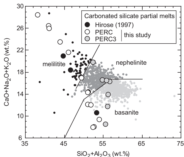
Fig. 11. Classification of alkaline to strongly alkaline ocean island lavas (GEOROC database: http://georoc.mpch-mainz.gwdg.de/georoc/ ) as melilitites, nephelinites, and basanites, following the scheme of LeBas (1989). Also plotted are carbonated silicate partial melts of peridotite derived from this study and from Hirose (1997).
