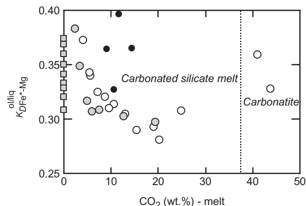
Fig. 10. Olivine–liquid Fe * –Mg distribution coefficient, K_{\text{DFe}^*-\text{Mg}}^{\text{ol/liq}} , as a function of CO 2 concentration (wt.%) in partial melts of carbonated peridotite at 3 GPa (this study and Hirose, 1997) compared with results for nominally CO 2 -free silicate melts at the same pressure (Ulmer, 1989; Hirose & Kushiro, 1993; Walter, 1998). For experiments of Hirose (1997), melt CO 2 concentrations are estimated as described in the caption to Fig. 3. A slight dependence of decreasing K_{\text{DFe}^*-\text{Mg}}^{\text{ol/liq}} with increasing concentration of melt CO 2 content is apparent from our data; however, the average values of K_{\text{DFe}^*-\text{Mg}}^{\text{ol/liq}} remains similar to that for olivine–basaltic melt equilibria.
