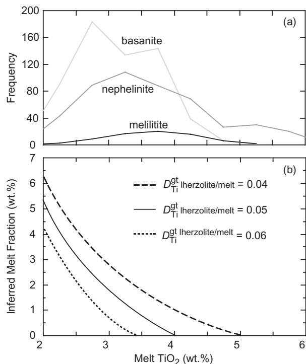
Fig. 13. (a) Frequency distribution for TiO 2 concentrations of basanitic, nephelinitic, and melilititic OIB depicted in Fig. 12, and (b) relations between concentration of TiO 2 and the extent of melting of fertile peridotite used to estimate melt fractions in sources of highly alkaline lavas in Fig. 14. Melt fractions in (b) are based on batch melting of garnet lherzolite with bulk TiO 2 content equal to 0.2 wt%, which is that of the primitive mantle (McDonough & Sun, 1995) and D_{\text{Ti}}^{\text{gt lherzolite/melt}} ranging from 0.04 to 0.06, estimated based on experiments from this study and that of Walter (1998). The overall high concentrations of TiO 2 in these lavas (a) require small-degree partial melting if we assume a normal peridotite source and that nephelinites and melilitites are, on average, enriched in TiO 2 relative to basanites and hence represent smaller degree partial melts.
