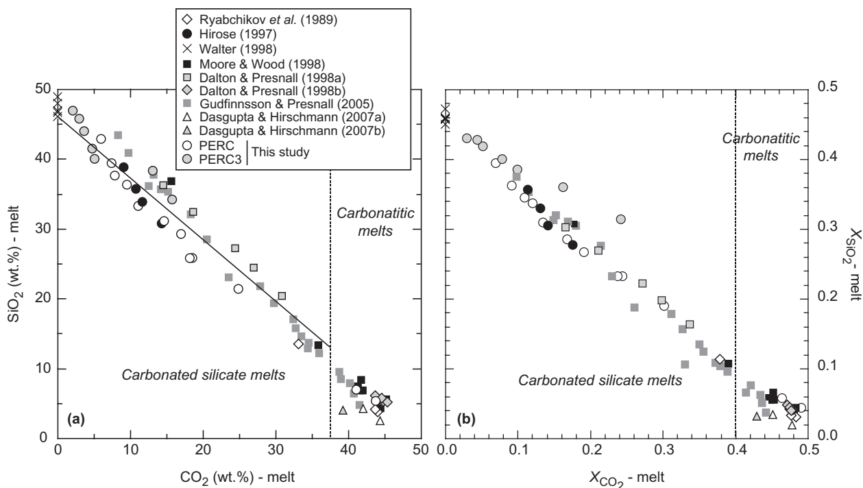
Fig. 7. Measured concentrations of SiO 2 vs estimated concentrations of CO 2 in carbonatite and carbonated silicate partial melts from this study and other studies in simple (Dalton & Presnall, 1998a, 1998b; Moore & Wood, 1998; Gudfinnsson & Presnall, 2005) and complex (Ryabchikov et al. , 1989; Hirose, 1997; Walter, 1998; Dasgupta & Hirschmann, 2007a, 2007b) peridotite ± CO 2 compositions from 2.8 to 8 GPa in terms of weight per cent (a) and oxide mole fraction (b). For the experiments of Hirose (1997), melt CO 2 concentrations are estimated as described in the caption to Fig. 3. All melts coexist with olivine and orthopyroxene, and consequently all have silica activity buffered. The linear fit of the melt compositions between 0 and 37 wt% CO 2 in the melt is given by C_{\text{SiO}_2}^{\text{liq}} = 46 \cdot 2 - 0.89 C_{\text{CO}_2}^{\text{liq}} , where C_{\text{SiO}_2}^{\text{liq}} and C_{\text{CO}_2}^{\text{liq}} are weight concentrations of SiO 2 and CO 2 in the melt. It should be noted that these SiO 2 concentrations are not normalized on a volatile-free basis, whereas melt SiO 2 concentrations in Figs 3, 9, 12 and 14 and in Table 3 are normalized to volatile-free compositions. This linear parameterization allows estimation of the SiO 2 concentrations of model melts as a function of bulk CO 2 content and extent of melting that is presented in Fig. 14.
