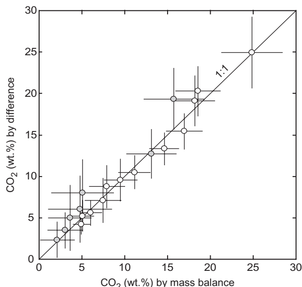
Fig. 6. Estimates of \text{CO}_2 concentration in the partial melts derived from PERC (white circles) and PERC3 (grey circles) carbonated peridotite based on differences between 100% and average analytical totals from replicate electron microprobe analyses vs the \text{CO}_2 concentrations estimated from melt proportion derived from mass-balance calculation and the assumption that all the carbon in the charge resides in the partial melt when crystalline carbonate is absent. The error bars in \text{CO}_2 derived from microprobe totals reflect the 1\sigma (wt%) uncertainties in the analytical totals, and the error bars in \text{CO}_2 estimates from mass-balance calculations are based on uncertainties in estimated phase proportions (Table 2). Close adherence of the data to the 1:1 line indicates good agreement between the two methods and lends confidence to our estimates of \text{CO}_2 concentrations in quenched carbonated silicate melts.
