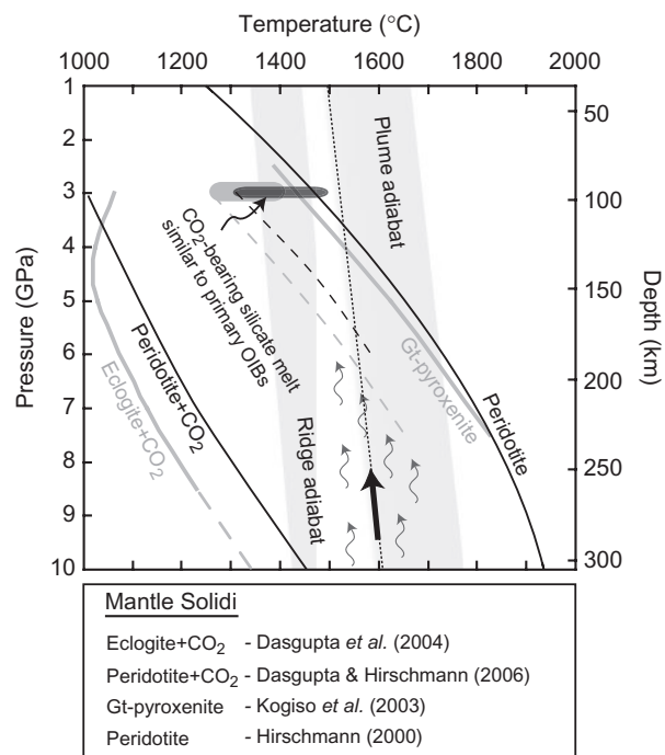
Fig. 15. Pressure–temperature diagram showing locations of various mantle solidi compared with the conditions of generation of carbonated silicate melts possibly similar to primary alkali ocean island basalts in equilibrium with peridotite (this study). Intersection between oceanic geotherms and carbonated mantle peridotite (Dasgupta & Hirschmann, 2006) and eclogite (Dasgupta et al. , 2004) solidi at very deep upper mantle conditions indicates likely generation of incipient carbonatitic melt at great depths. Reaction between buoyant carbonatitic melts (curved arrows) and overlying mantle peridotite will give rise to carbonated silicate melts at depths much shallower than carbonated mantle solidi, but significantly deeper than the solidus of volatile-free peridotite (Hirschmann, 2000). The P – T slopes of carbonated silicate melting for eclogite and peridotite are not experimentally constrained and so are plotted as dashed lines (grey for eclogite; black for peridotite) subparallel to the solidi of garnet pyroxenite (Kogiso et al. , 2003) and peridotite (Hirschmann, 2000), respectively.
