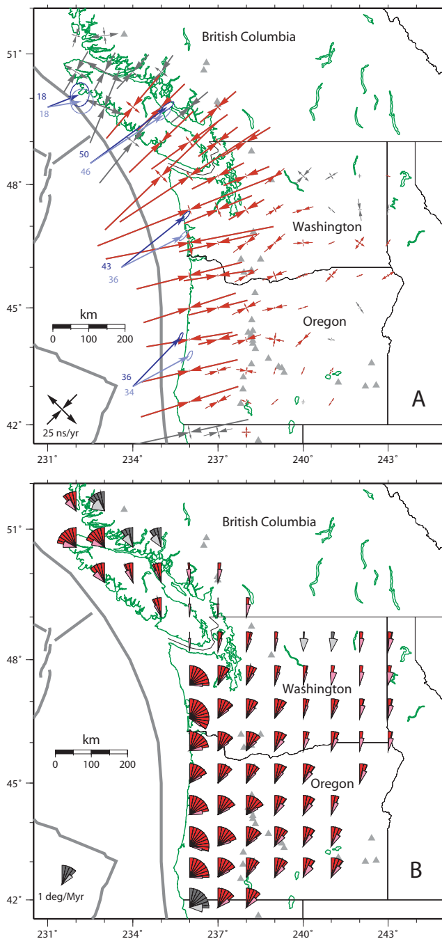
Figure 5. Principal strain and rotation rates derived from GPS velocities. Area is divided into bins of 2° in longitude by 1.6° in latitude in which the uniform strain and rotation rates are calculated from the GPS velocities contained within (minimum of six velocities). (a) Red symbols show principal strain rates where the uncertainty is less than or equal to 5 ns yr -1 and grey where uncertainty is between 5 and 10 ns yr -1 . Dark blue arrows show convergence of Juan de Fuca with North America, lighter blue arrows are convergence with the coastal blocks; both labelled in mm yr -1 . (b) Rotation rates for same regions. Red symbols show where the uncertainty is less than 0.3° Myr -1 and grey where it is between 0.3 and 0.6° Myr -1 . Fan symbols show the rate and sense of rotation (a fan opening 45° clockwise indicates 1° Myr -1 of clockwise rotation). The smaller attached fans show the 1σ uncertainty in the rotation rate.
