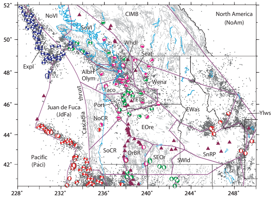
Figure 6. Shallow seismicity (dots; depth <20 km), earthquake focal mechanisms, domain boundaries (purple lines) and faults (thin grey lines) for the Pacific Northwest. Each domain is identified by a four-letter code as described in the text. Red focal mechanisms are from the Harvard CMT catalogue, blue from Braunmiller & Nabelek (2002) purple from miscellaneous sources (see Supplementary Material) green from a compilation by Pezzopane & Weldon (1993) Canadian earthquake quake data from http://www.pgc.nrcan.gc.ca/seismo/recent/eqmaps.html ; US quakes from http://www.ncedc.org/anss/catalog-search.html .
