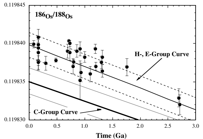
Fig. 4. The ^{186}\text{Os}/^{188}\text{Os} versus time for the Os-rich alloy data. The ^{186}\text{Os}/^{188}\text{Os} data for the Os-rich alloys are plotted versus TRD ages calculated from their respective ^{187}\text{Os}/^{188}\text{Os} ratios. The proposed ^{186}\text{Os}/^{188}\text{Os} time evolution curve for the upper mantle (H-, E-Group Curve) and the carbonaceous chondrite time evolution curve (based on Allende data) are shown as solid lines with respective \pm 2\sigma errors shown as dashed lines.
