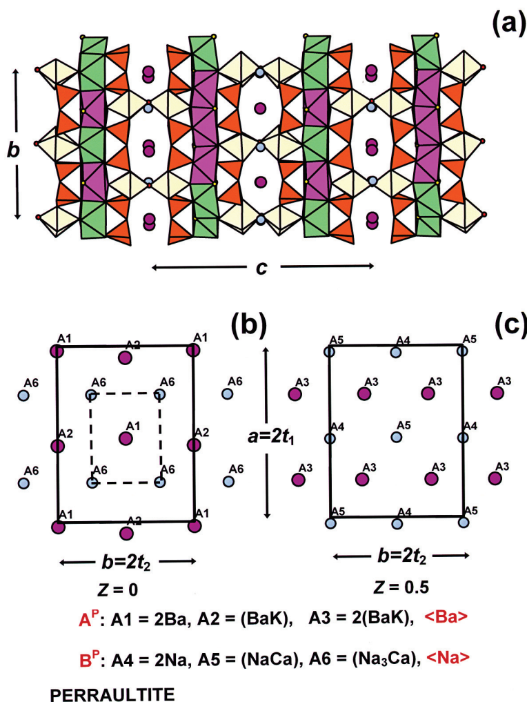
FIG. 20. Perraultite. General view of the crystal structure viewed down [100] (a), close-packed I layers of cations at z = 0 (b) and z = 0.5 (c). Legend as in Figure 12; the Mn^{2+} octahedra are magenta, and the Ba and Na atoms at the P sites are shown as large magenta and smaller blue circles. The minimal cell is shown by dashed lines in (b).
