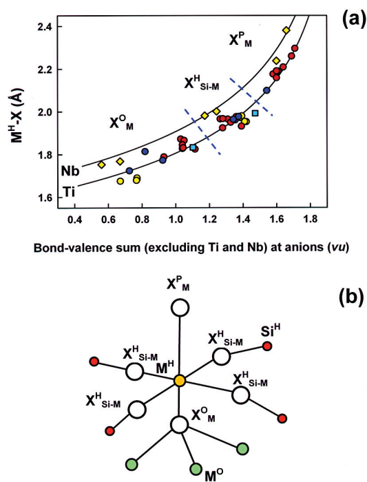
FIG. 31. The M^H-X distances (Å) versus bond-valence sums (excluding Ti and Nb) at X anions ( vu ), M^H = Ti, Nb (a). A schematic representation of the topology of the M^H site (b). Data for Group II (bussenite, hejtanite-P and yoshimurite), Group III (epistolite, vuonnemite, lamprophyllite-2M, lamprophyllite-2O and nabalamprophyllite) and Group IV (murmanite, lomonosovite, quadruphite, sobolevite and polyphite) are shown as navy blue, yellow and red circles ( M^H = Ti ) or diamonds ( M^H = Nb ). The data on orthoericssonite are shown as light blue squares. Dashed blue lines separate X_M^O , X_{Si-M}^H and X_M^P data. Solid black lines show ideal bond-valence curves for Ti^{4+} and Nb^{5+} . In diagram (b), M^H , M^O , Si^H and X sites are shown as medium yellow and green, small orange and large white circles.
