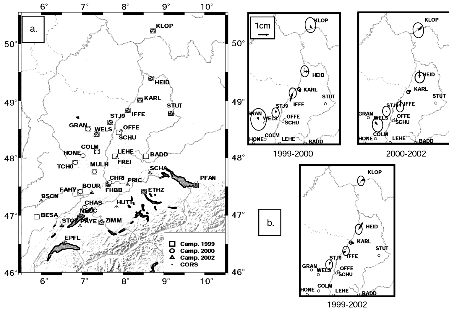
Fig. 30. Left panel (a): GPS network in the Upper Rhine Graben area. Squares: campaign 1999; circles: campaign 2000; triangles: campaign 2002. Right panels (b): differential horizontal displacements during various time spans relative to Karlsruhe (confidence of the error ellipses 95%).
