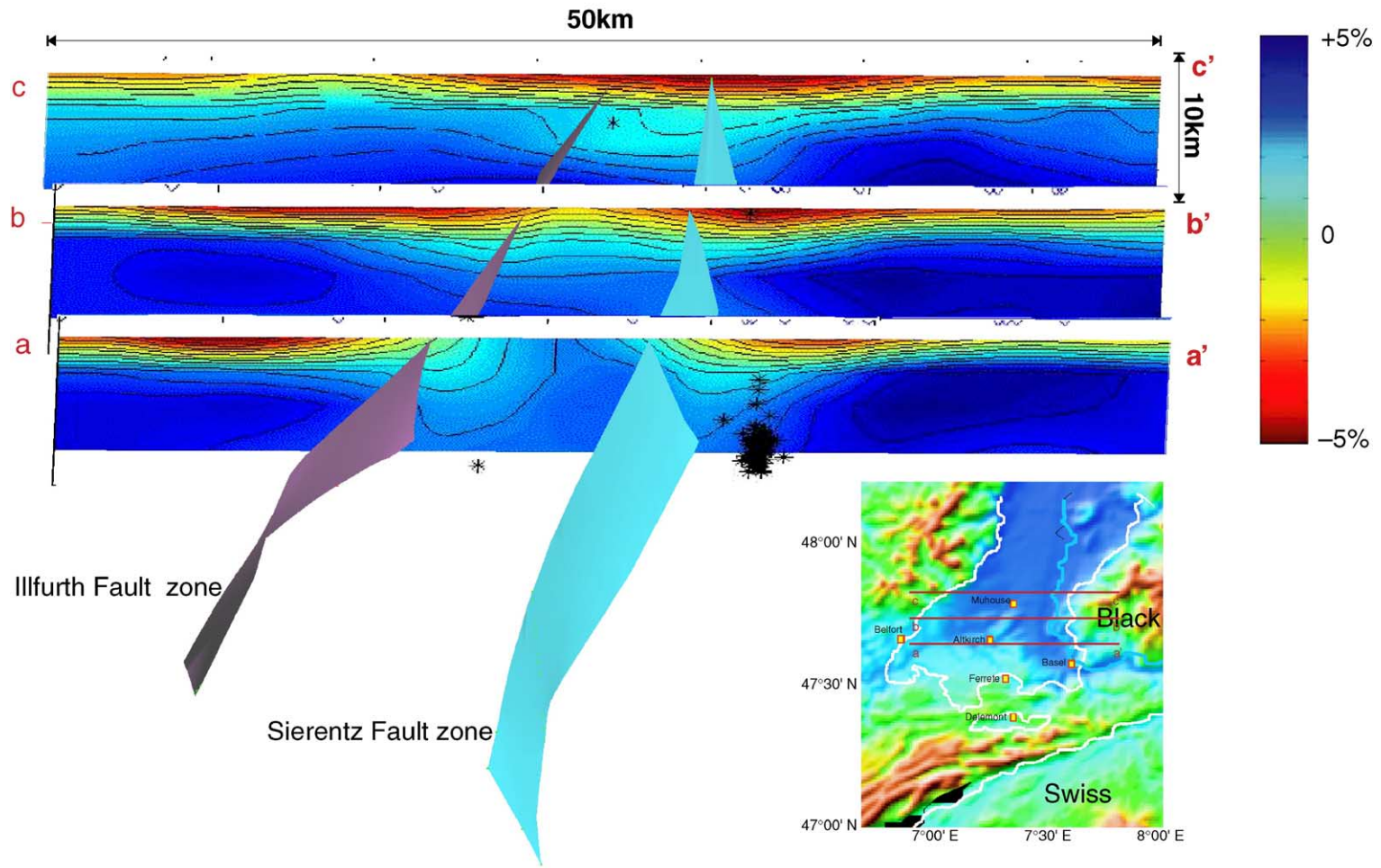
Fig. 26. E–W tomographic cross-sections of P-wave velocity travel time residuals through the southern part of Upper Rhine Graben, showing position of Illfurth and Sierentz faults that is constrained by reflection-seismic data on one of the cross-sections. Contour line interval is 1%. Black stars: earthquake hypocentres. For discussion, see text. The cross-sections have a length of 50 km, and a depth of 10 km. For location see topographic map. White lines denote the edge of the distribution of the Tertiary sediments in the Rhine Graben, Delémont Basin and Molasse Basin.
