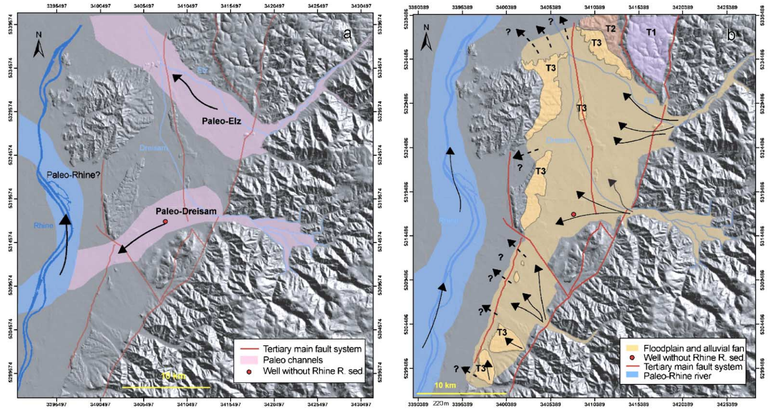
Fig. 33. Evolution of the drainage system during the Quaternary. (a) At the beginning of Quaternary, the Elz and Dreisam flow respectively toward the NW and the SW, following the channels identified on Fig. 3. (b) During Riss glacial age, sediments from the Black Forest form a continuous flood plain in the graben. Extension of this flood plain is not known because of subsequent erosion. (c) During Würm glacial age, the Rhine river shifts eastward, east of the Kaiserstuhl volcano (NW corner of the area). In the south, incision from the Rhine river reaches the trace of the Rhine river fault. (d) Today, the Rhine river has moved back west of the Kaiserstuhl, while the Elz and Dreisam are still flowing toward the NW.
