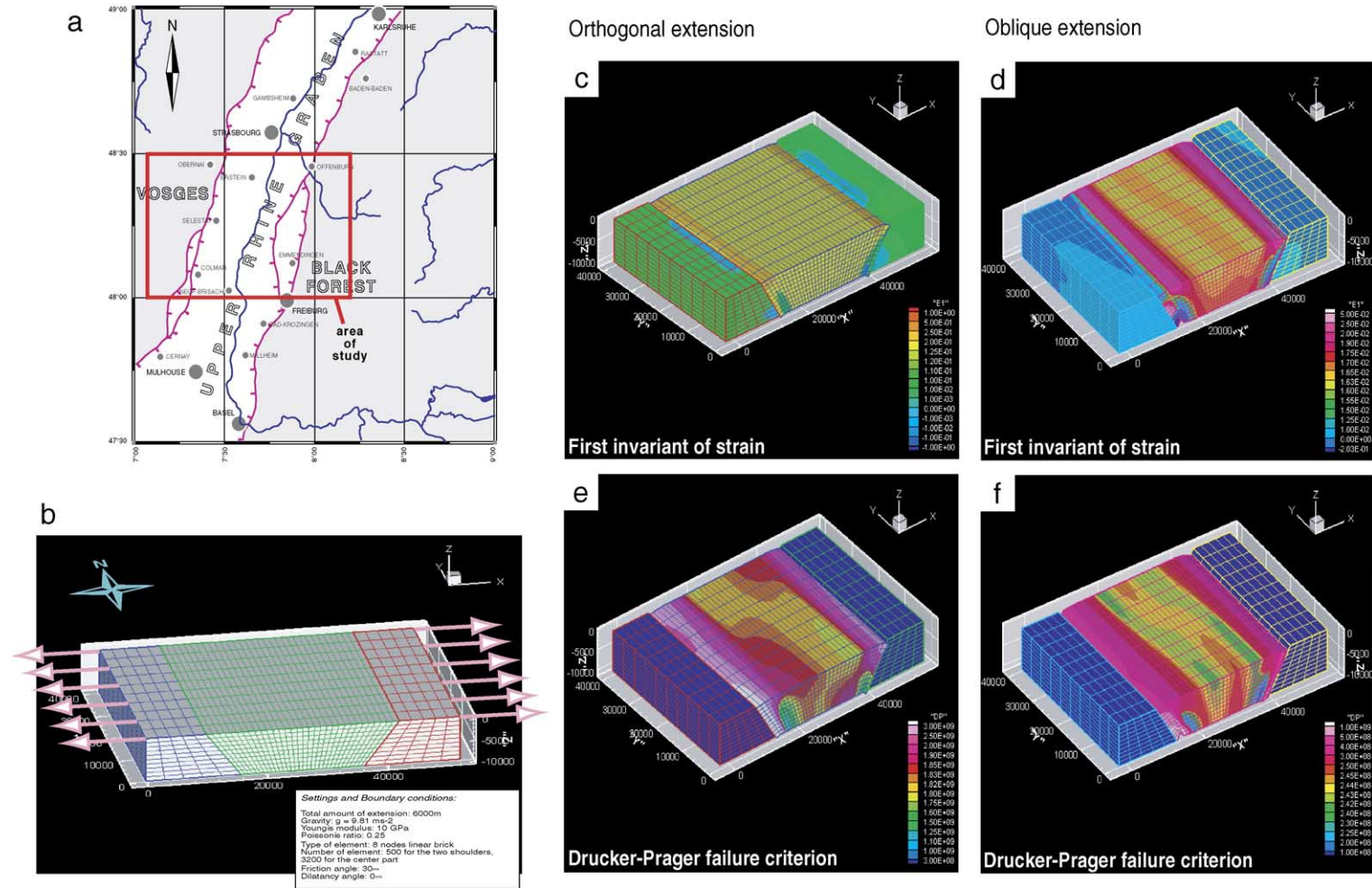
Fig. 22. (a) Sketch map of the southern part of the Upper Rhine Graben, showing the western and eastern main border faults, and the area covered by the numerical models shown in Fig. 23, denoted by the red rectangle. (b) Initial (i.e. pre-rift) geometry of the studied graben segment, used for the forward model. The two lateral blocks correspond to the future graben shoulders (i.e. Vosges and Black Forest Mountains to the west and the east, respectively). Their contact zones with the central block correspond to the border faults delimiting the Upper Rhine Graben. Right panel: Results of the forward model. Both purely orthogonal and partly oblique extension scenarios were tested. Results are presented in terms of the first invariant of strain E_1 (sum of the diagonal terms of the strain tensor): (c) orthogonal and (d) oblique extension. And in terms of the Drucker–Prager (DP) failure criterion (numerical equivalent of a Mohr–Coulomb criterion, see Appendix B for further details): (e) orthogonal and (f) oblique extension. Cartesian coordinates are in meters.
