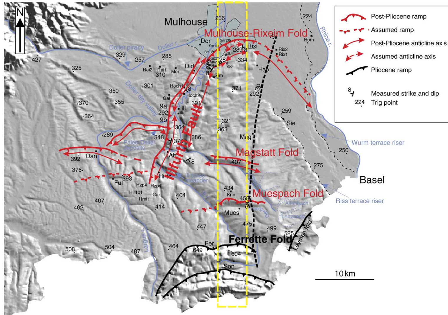
Fig. 37. Digital Elevation Model of Mulhouse Horst domain (vertical exaggeration \times 10 , source: IGN topomap) showing morphostructural interpretation (modified after Nivière and Winter, 2000). Dashed line yellow box: trace of cross-section given in Fig. 39.
