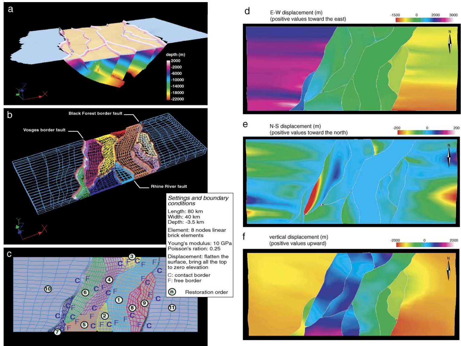
Fig. 23. Left panel: Construction of initial multi-block domain used for backward modelling (for location see Fig. 22). (a) Present-day geometry of the geological domain. (b) Finite elements domain built from this geological domain. (c) Contact sequence of movement used for backward modelling the contact borders, (C) are borders containing the “slave” nodes and free borders, (F) those containing “target” nodes. Right panel: Results of backward model, presented in terms of displacement (m), showing the top surface of all blocks, (d) displacement along the E–W x -axis, (e) displacement along the N–S y -axis, (f) displacement along the vertical z -axis.
