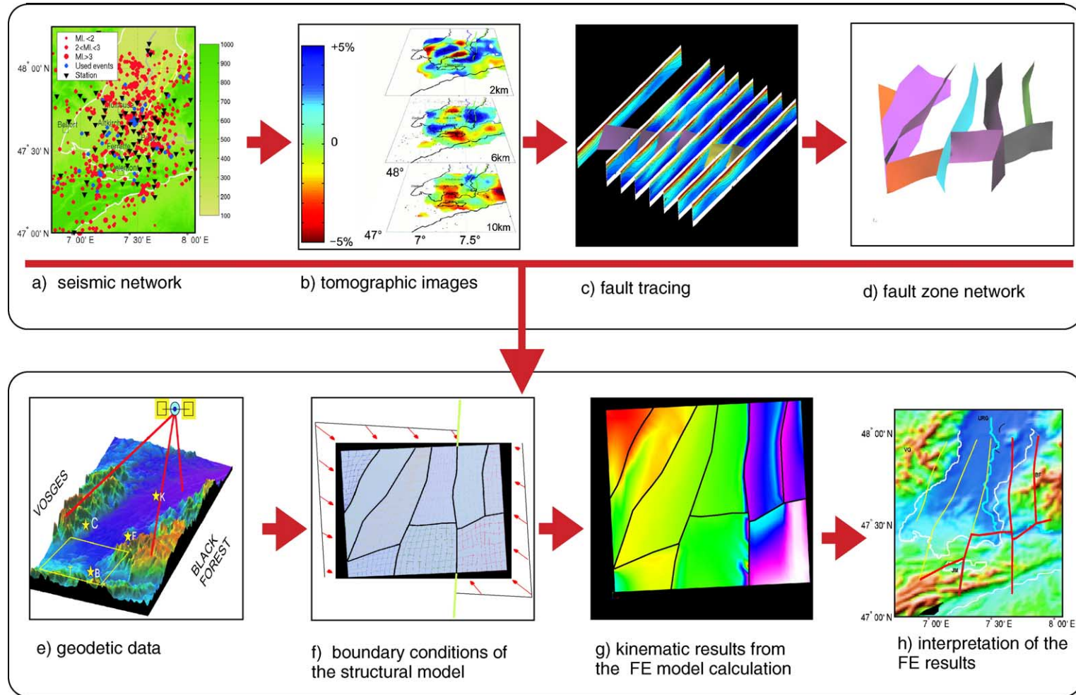
Fig. 2. Steps of the methodology used. Upper panel: synthesis of local earthquake tomography data to construct the structural domain (a) seismic network for tomographic data acquisition, (b) tomographic database, (c) tracing of fault zones through tomographic profiles, (d) final fault zone network. Lower panel: synthesis of regional boundary conditions based on geodetic constraints to be integrated with structural data in a finite element model, and its geological interpretation (e) geodetic data, (f) building of the structural domain and finite element mesh, (g) results from finite element calculation of northward displacement, (h) interpretation of results (active faults in red).
