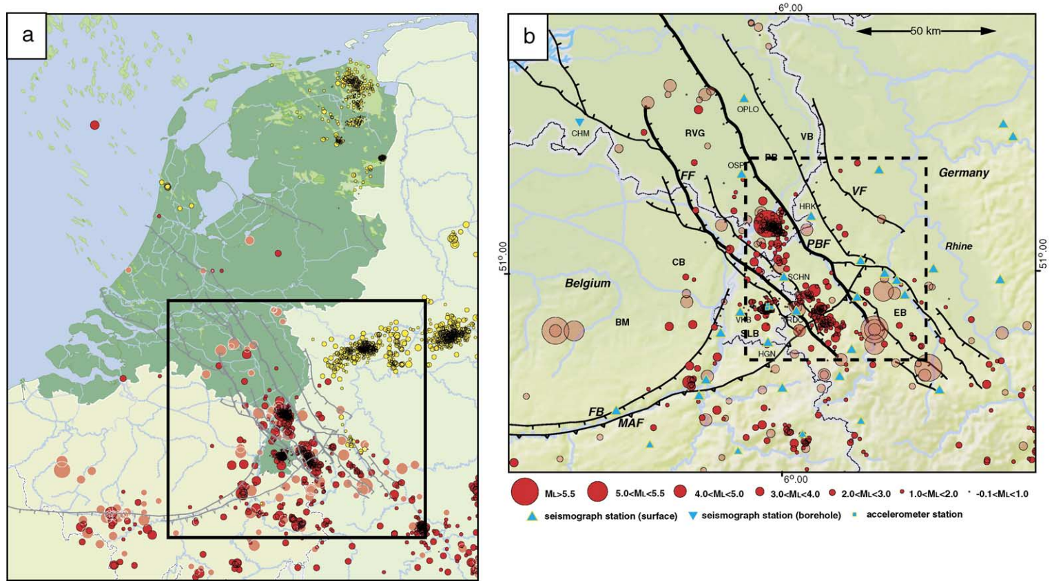
Fig. 43. (a) Distribution of seismicity since 1900 in the LRG and immediate surroundings, with red circles denoting natural seismicity and yellow circles denoting man-induced seismicity (after Van Eck et al., in press). The earthquakes are scaled according to magnitude. Gray lines indicate base-Tertiary faults. RVRS = Roer Valley Rift System; LRE = Lower Rhine Embayment; RB = Ruhr Basin; Box denotes area shown in Fig. 43b (modified after Van Eck et al., in press). (b) Epicentre map of natural seismicity in and around the Roer Valley Rift System for the period 1900–2005. Earthquakes are shown as red circles, scaled according to magnitude; events before 1980 in light red, after 1980 in dark red. Dashed box indicates area of Fig. 44. Tectonic structures: BM = Brabant Massif; RVG = Roer Valley Graben; PB = Peel Block; VB = Venlo Block; CB = Campine Block; EB = Erft Block; SLB = South Limburg Block; PBF = Peel Boundary Fault; FF = Feldbiss Fault; VF = Viersen Fault; FB = Faille Bordière; MAF = Midi-Aachen Thrust Fault (modified after Dost and Haak, in press).
