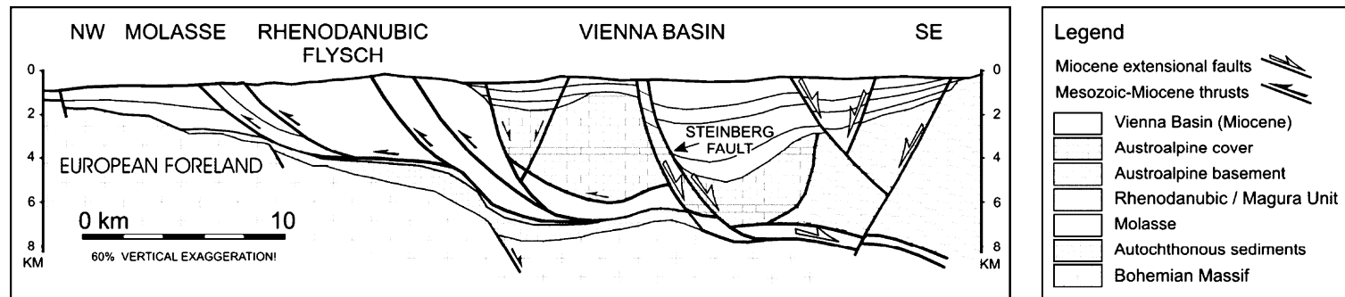
Fig. 15. Cross-section through the northern Vienna Basin (after Wessely, 1993). The major listric normal faults (Steinberg fault system, 5.6 km vertical throw) root in the Alpine–Carpathian sole thrust. Location of these major faults at the NW basin margin controls the asymmetrical geometry of the basin and the NW tilt of its sedimentary fill.
