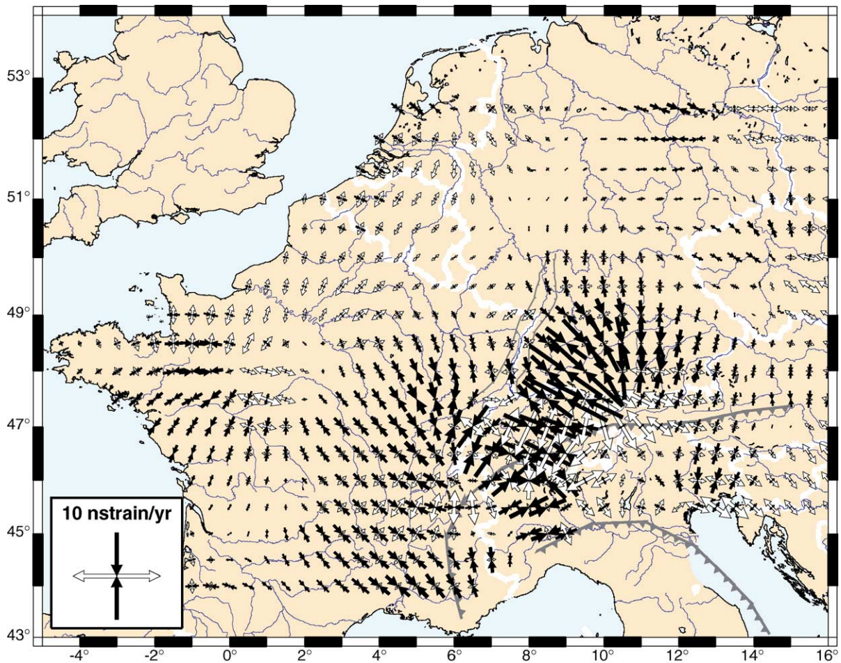
Fig. 11. Principal axes and values of strain rates obtained by the collocation method (Straub, 1996; Kahle et al., 2000). Covariance distance: 123 km; standard deviation sigma of signal: 0.85 mm/yr. Compressional and extensional axes are in black and in white, respectively. White contour lines denote the national borders. The formal error is between 4 and 7 nstrain/yr. For discussion, see text.
