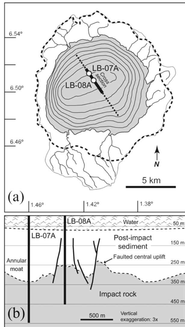
Fig. 2. a) Schematic map of Lake Bosumtwi, Ghana, showing lake drainage basin, lake bathymetry, present morphologic rim of the Bosumtwi impact crater (heavy dashed line), and location of ICDP deep drill cores LB-07A and LB-08A along seismic profile B2000-1, shown by thin dashed line across lake. The bathymetric contour interval is 10 m. b) Generalized interpreted geologic cross-section (heavy solid line at lake center, Fig. 2a) along seismic profile B2000-1, showing units penetrated by drill cores LB-07A and LB-08A. Modified from Jones et al. (1981), Scholz et al. (2002), Koeberl and Reimold (2005), and Milkereit et al. (2006).
