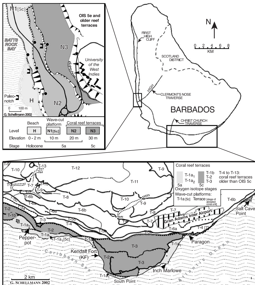
Fig. 1. The island of Barbados with MIS-5 reefs on the south and west coasts. Study sites are marked. On the south coast transect—Inch Marlowe Point (IM), Pepperpot (PEP), Kendall Fort (KF), Paragon Point (U18) and Salt Cave Point (U15). On the west coast transect—Batts Rock Bay (sites BRB1, BRB2, BRB3 and BRB4). More detailed site descriptions are given in the text. The U-series analyses for samples or sites recognised as not in situ (KF, BRB2) are included in Table 1 but not in the data summary (Fig. 2). Further details of mapping are given in [19–21].
