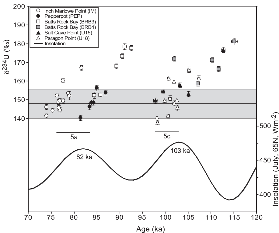
Fig. 2. Summary of U-series data for in situ, reef crest deposits (calculated age vs. \delta^{234}\text{U}_i ) from this study and comparison with July 65^\circ\text{N} insolation forcing curve [51]. Site BRB1, even though it is an in situ deposit, is not included here because it represents deep water growth and therefore its relationship to the timing of a sea-level highstand is not clear. The shaded region defines the generally accepted \pm 8\text{‰} band of \delta^{234}\text{U} values that define a reliable age (to within 2 ka). The age and \delta^{234}\text{U}_i data from each site display a rough linear correlation. A similar trend has also been described in previous studies, however in this case the trend is clearly identifiable even within the 8\text{‰} \delta^{234}\text{U} band, especially for the two younger deposits. If the oceanic \delta^{234}\text{U} at the time of deposition of these corals was equal to the present-day value, the timing of each event can be accurately and precisely determined by where the trend line intersects the modern \delta^{234}\text{U}_i value of 149\text{‰} . Summary of total data set, including samples not in growth position is given in Table 1. The timing of the peak sea level for the “classic” MIS-5a and 5c events at 84 and 101 ka coincide with or slightly postdate the associated insolation peak, consistent with the Milankovitch model of insolation forcing. The presence of an additional MIS-5a highstand, identified in this study at 77 ka BP, demonstrates that orbital forcing alone cannot account for the observed changes in ice volume during this period.
