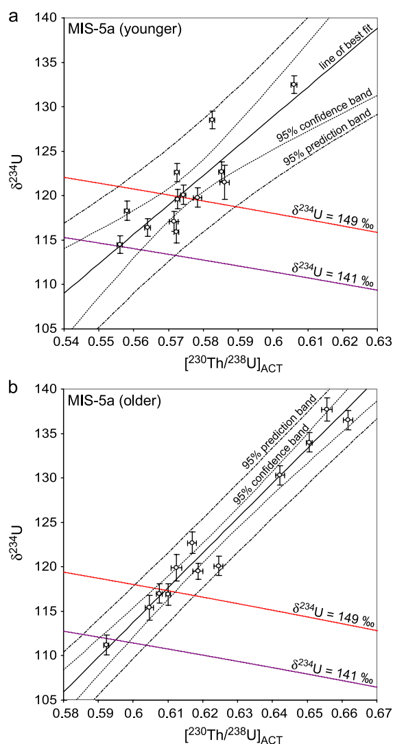
Fig. 3. Determination of line of best fit and 95% confidence and prediction bands for the younger (a) and older (b) MIS-5a features. The representative \delta^{234}\text{U}_m and [^{230}\text{Th}/^{238}\text{U}]_{\text{ACT}} values for each feature are determined by estimating where the line of best fit intersects the evolution curve for a chosen initial \delta^{234}\text{U} value. The uncertainties for the \delta^{234}\text{U}_m and [^{230}\text{Th}/^{238}\text{U}]_{\text{ACT}} parameters for each feature are determined using either the 95% confidence band or 95% prediction band and these errors are propagated through the U-series age equation to calculate a mean age or duration of deposition, respectively. The representative \delta^{234}\text{U}_m and [^{230}\text{Th}/^{238}\text{U}]_{\text{ACT}} , and hence age estimates, for these deposits change depending on the assumed initial \delta^{234}\text{U} value.
