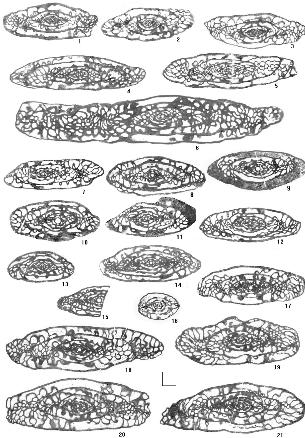
Plate 2. 1–3. Triticites aff. ishimbaji Rozovskaya. GIN 4781/ 29, GIN 4781/ 21, GIN 4781/30 accordingly, Samples AC14 and RL; 4–7. Triticites ex gr. ohioensis Thompson. GIN 4781/31, GIN 4781/1, GIN 4781/32, GIN 4781/33 accordingly, Sample C1; 8–10. Triticites aff. shikhanensis Rozovskaya. GIN 4781/34, GIN 4781/35, Sample C24; 11–15. Triticites karlensis Rozovskaya. GIN 4781/36, GIN 4781/37, GIN 4781/34, GIN 4781/35, GIN 4781/38 accordingly, Sample C24; 16. Triticites globoides Z. Mikhailova. GIN 4781/39, Sample AC14; 17, 18. Rauserites ex gr. postarcticus (Rauser-Chernousova). GIN 4781/40, GIN 4781/41, Samples RL2 and RL accordingly; 19–21. Rauserites variabilis Rozovskaya. GIN 4781/42, GIN 4781/43, GIN 4781/44 accordingly, Samples AC14 and RL. All figures – scale-bar = 0.5 mm.
