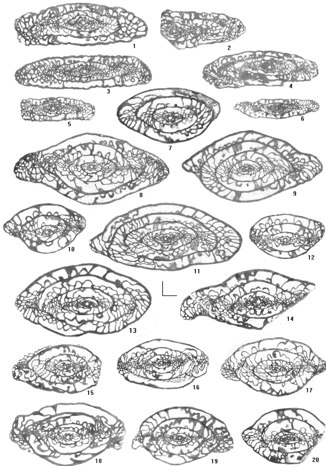
Plate 5. 1, 2. Rugosofusulina (?) iranica n. sp. GIN 4781/70 (holotype), GIN 4781/71, Sample AC14; 3–6. Rugosofusulina (?) elongata n. sp. GIN 4781/88 (holotype), GIN 4781/89, GIN 4781/90, GIN 4781/91 accordingly, Sample AC14; 7–9, 11, 13, 14, 18. Ultradaxina bosbytauensis distincta n. subsp. (7) GIN 4781/72, Sample AC29; (8, 9, 11) GIN 4781/77 (holotype), GIN 4781/78, GIN 4781/79 accordingly, Sample ML3; (13) GIN 4781/80, Sample P3; (14, 18) GIN 4781/81, GIN 4781/92, Sample P6; 10, 12, 19. Ultradaxina (?) kozui (Deprat). (10,12) GIN 4781/82, GIN 4781/83, Sample P4; (19) GIN 4781/84, Sample P8; 15, 16. Ultradaxina (?) kosvaensis (Echlov). GIN 4781/85, GIN 4781/86, Samples P3 and C accordingly; 17. Likharevites aff. paranitidus (Bensh). GIN 4781/87, Sample P4; 20. Likharevites esetensis (Davydov). GIN 4781/93, Sample P2. All figures – scale-bar = 0.5 mm.
