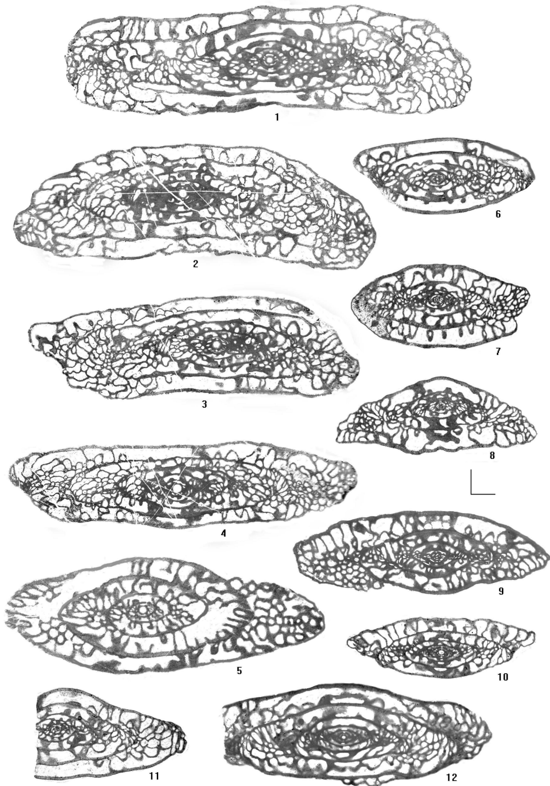
Plate 3. 1–4. Rauserites rossicus (Schellwien). GIN 4781/45, GIN 4781/46, GIN 4781/47, Sample RL1; 5. Jigulites cf. formosus Rozovskaya. GIN 4781/48, Sample C21; 6. Triticites aff. samaricus Rauser-Chernousova. GIN 4781/49, Sample RL2; 7–9. Rauserites (?) persicus n. sp. GIN 4781/50, GIN 4781/51, GIN 4781/52 (holotype) accordingly, Samples RL and AC14; 10. Rauserites sp. 1. GIN 4781/53, Sample RL; 11. Triticites ex gr. simplex (Schellwien). GIN 4781/54, Sample RL; 12. Triticites ex gr. secalicus Say. GIN 4781/55, Sample RL. All figures – scale-bar = 0.5 mm.
