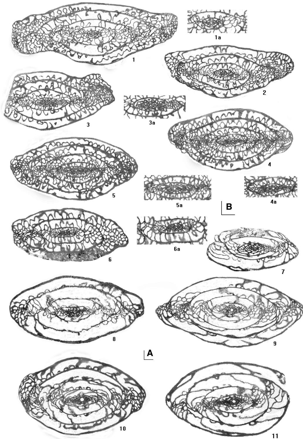
Plate 7. 1–3, 1a, 3a. Likharevites kokpectensis (Scherbovich). (1, 3) GIN 4781/105, GIN 4781/106, Sample R2; (2) GIN 4781/107, Sample RupA; 4, 4a, 5, 5a. Likharevites inglorius (Bensh). GIN 4781/108, GIN 4781/109, Sample C45; 6, 6a. Likharevites ex gr. inglorius (Bensh). GIN 4781/110, Sample C47; 7. Pseudoschwagerina ex gr. extensa F. et G. Kahler. GIN 4781/111, Sample P13; 8. Pseudoschwagerina sp. GIN 4781/112, Sample C45; 9–11. Pseudoschwagerina extensa F. et G. Kahler. GIN 4781/113, GIN 4781/114, GIN 4781/115, Samples C42, C45, and PR1 accordingly.
