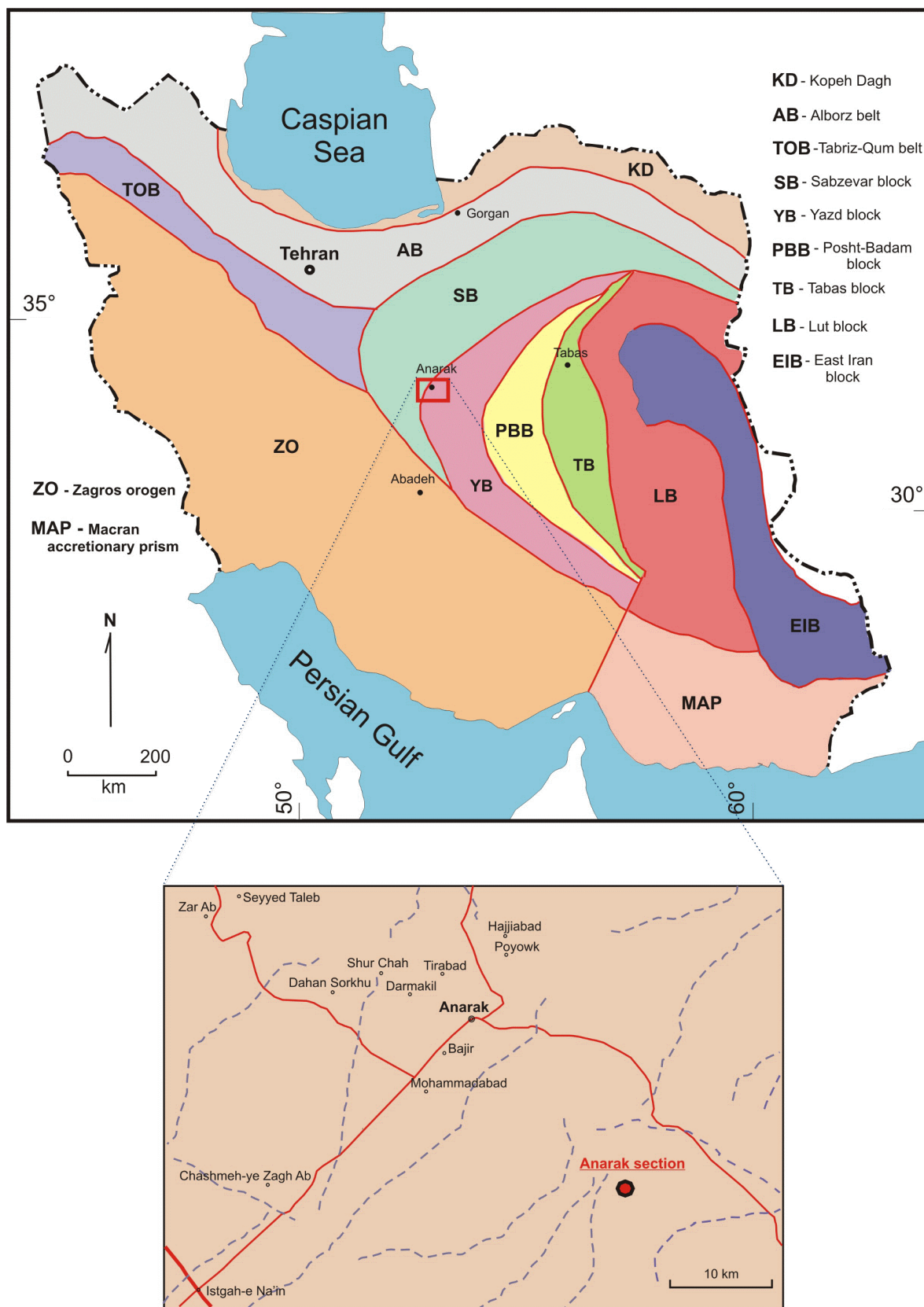
Figure 1. Area of investigation on the schematic tectonic map of Iran [Alavi, 1991].
