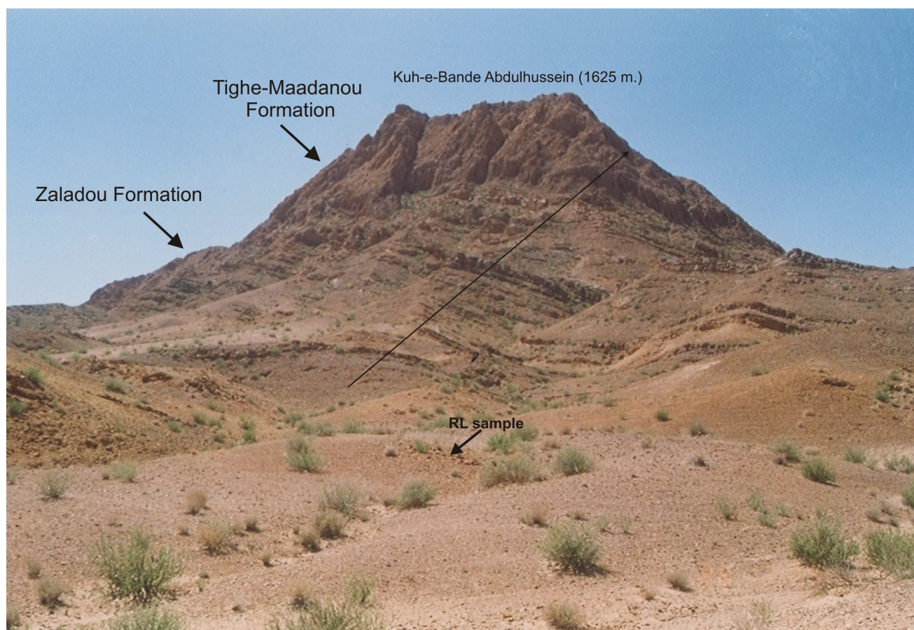
Figure 3. Anarak section.
