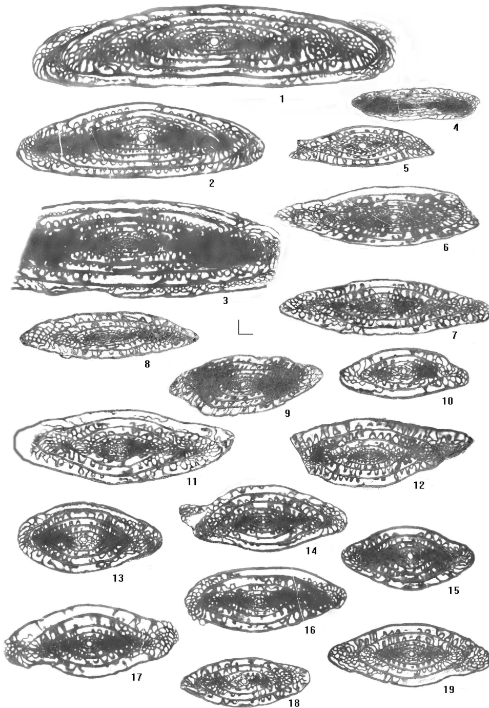
Plate 10. 1. Ruzhenzevites subcylindricus (Bensh). GIN 4781/138, Sample PR2; 2. Ruzhenzevites zaladuensis brevis Leven. GIN 4781/139, Sample PR2; 3. Ruzhenzevites zaladuensis zaladuensis Leven. GIN 4781/140, Sample P10; 4. Rugosochusenella sp. GIN 4781/141, Sample C46; 5. Pseudofusulina (?) sp. GIN 4781/142, Sample R2; 6, 7. Pseudofusulina (?) narjanmarica Konovalova. GIN 4781/143, GIN 4781/144, Samples Rup and C46; 8. Rugosochusenella paragregaria (Rauser-Chernousova). GIN 4781/145, Sample C47; 9. Praeskinnerella (?) huangchuigouensis Zhang et Xia. GIN 4781/146, Sample Rup; 10, 18. Anderssonites nanus (Sjomina). GIN 4781/147, GIN 4781/48, Sample P6; 11. Anderssonites (?) aff. zarjae Potievskaya. GIN 4781/149, Sample AC28; 12. Pseudofusulina aff. conspiqua Rauser-Chernousova. GIN 4781/150, Sample RupA; 13. Anderssonites anderssoni nibelensis Volozhanina. GIN 4781/151, Sample P3; 14, 19. Anderssonites pseudoanderssoni pseudoanderssoni (Sjomina). GIN 4781/152, GIN 4781/153, Samples P8 and RupA; 15. Anderssonites anderssoni (Schellwien). GIN 4781/154, Sample P8; 16. Anderssonites pseudoanderssoni latiterminosa (Sjomina). GIN 4781/155, Sample P1; 17. Anderssonites sp. 4781/156, Sample P1. All figures – scale-bar = 0.5 mm.
