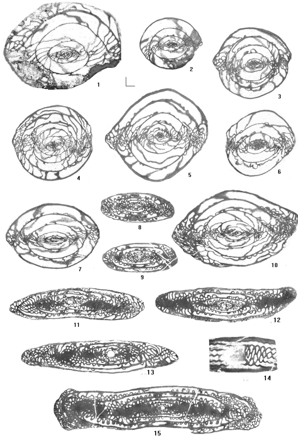
Plate 9. 1. Sphaeroschwagerina pavlovi (Scherbovich). GIN 4781/124, Sample C45; 2. Sphaeroschwagerina ex gr. spaerica (Scherbovich). GIN 4781/125, Sample C45; 3. Sphaeroschwagerina shamovi primitiva (Leven et Scherbovich). GIN 4781/126, Sample C45; 4. Sphaeroschwagerina moelleri (Rauser-Chernousova). GIN 4781/127, Sample P13; 5. Sphaeroschwagerina notabilis (Grozdilova). GIN 4781/128, Sample PR1; 6. Sphaeroschwagerina sp. 2. GIN 4781/129, Sample PR1; 7. Sphaeroschwagerina ellipsoidalis Rauser-Chernousova. GIN 4781/130, Sample PR1; 8, 9. Praepseudofusulina kljasmica (Sjomina). GIN 4781/131, GIN 4781/132, Sample P11; 10. Sphaeroschwagerina fusiformis (Krotowi). GIN 4781/133, Sample PR1; 11–13. Ruzhenzevites ferganensis (Dutkevitch). GIN 4781/134, GIN 4781/45, GIN 4781/10, Sample R3; 14, 15. Ruzhenzevites subcylindricus (Bensh). GIN 4781/136, GIN 4781/137, Sample PR2. All figures – scale-bar = 0.5 mm.
