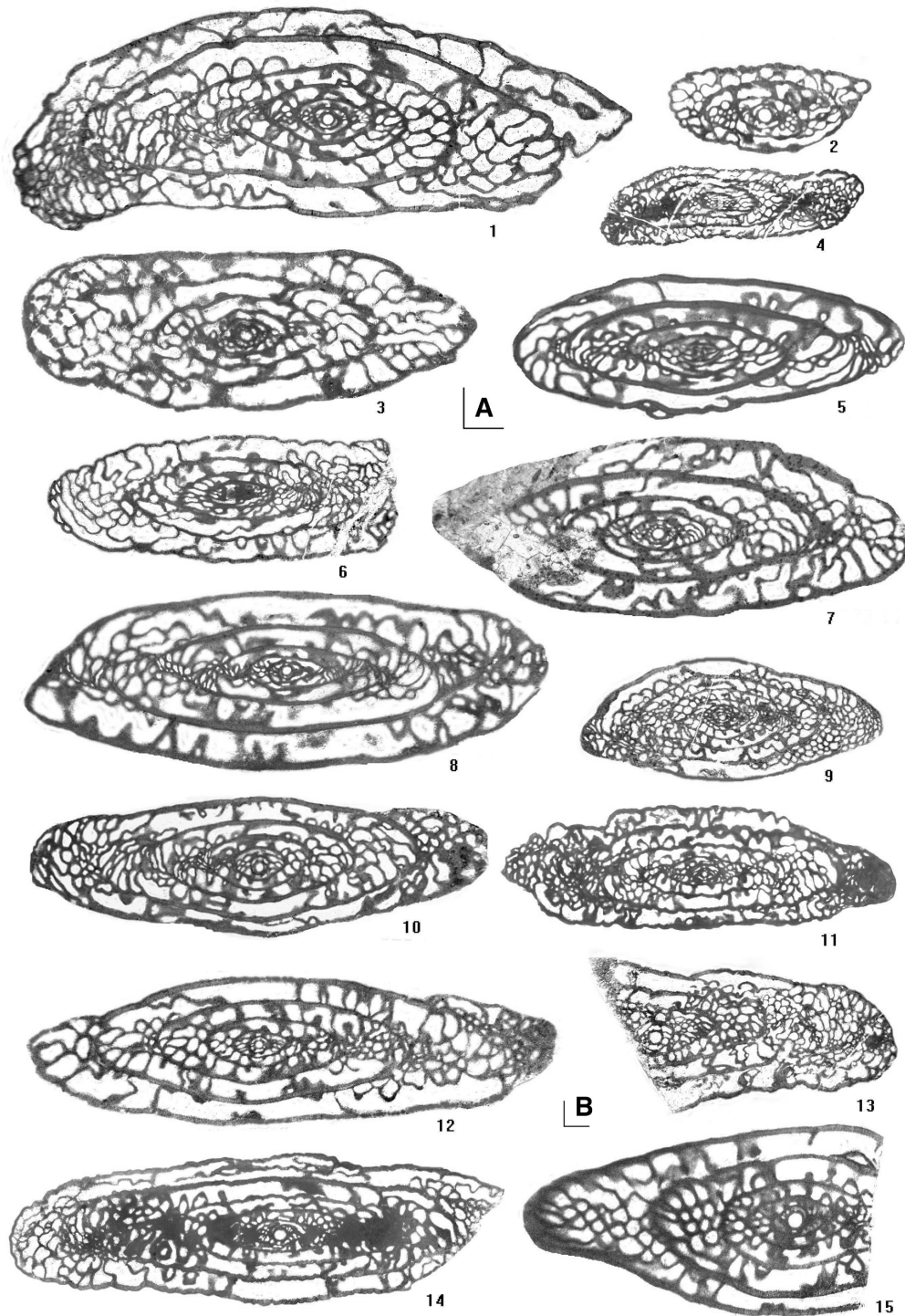
Plate 4. 1. Triticites nefandus Grozdilova. \times 15 . GIN 4781/56, Sample RL; 2. Rugosofusulina sp. 1. \times 10 . GIN 4781/41, Sample RL; 3. Triticites ex gr. nefandus Grozdilova. \times 15 . GIN 4781/57, Sample RL; 4. Rugosofusulina sp. 2. \times 10 . GIN 4781/58, Sample C45; 5, 7, 8. Rauserites stepanovi n. sp. \times 15 . GIN 4781/59, GIN 4781/61, GIN 4781/62 (holotype) accordingly, Sample C23; 6. Rugosofusulina aff. elliptica Rozovskaya. \times 10 . GIN 4781/60, Sample RL2; 9. Daixina aff. osimovkensis Scherbovich. \times 10 . GIN 4781/63, Sample C25; 10. Rauserites aff. postarcticus (Rauser-Chernousova). \times 15 . GIN 4781/23, Sample C23; 11. Rugosofusulina uralica Z. Mikhailova. \times 10 . GIN 4781/65, Sample C14; 12. Rauserites elongatissimus Rozovskaya. \times 15 . GIN 4781/66, Sample C20; 13. Rugosofusulina mutabilis Bensh. \times 10 . GIN 4781/ 67, Sample P9; 14. Rugosofusulina directa Bensh. \times 10 . GIN 4781/68, Sample P9; 15. Rauserites cf. erraticus Rozovskaya. \times 15 . GIN 4781/69, Sample C21. Figs. 1, 3, 5–8, 10, 12, 15 – scale-bar A = 0.5 mm, figs. 2, 4, 9, 11, 13, 14 – scale-bar B = 0.5 mm.
