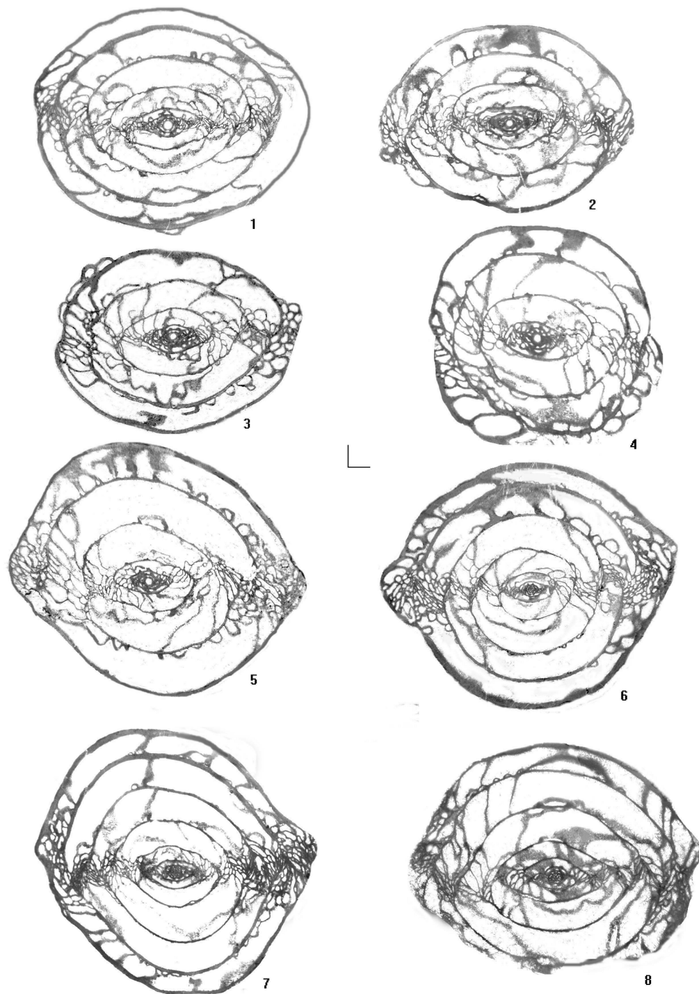
Plate 8. 1–3. Pseudoschwagerina turbida F. et G. Kahler. GIN 4781/116, GIN 4781/117, GIN 4781/118 accordingly, Sample C45; 4. Pseudoschwagerina ex gr. turbida F. et G. Kahler. GIN 4781/119, Sample PR1; 5. Pseudoschwagerina robusta (Meek). GIN 4781/120, Sample C47; 6, 7. Sphaeroschwagerina shamovi gerontica (Scherbovich). GIN 4781/121, GIN 4781/122, Samples C45 and PR1; 8. Sphaeroschwagerina sp. 1. GIN 4781/123, Sample P13. All figures – scale-bar = 0.5 mm.
