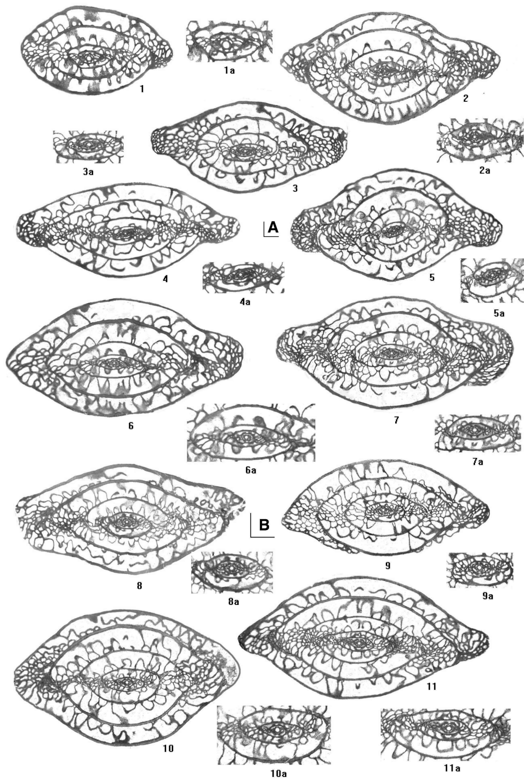
Plate 6. 1, 1a. Ultradaixina (?) kozui (Deprat). GIN 4781/94, Sample P8; 2–11, 2a–11a. Likharevites gracilis n. sp. (2, 2a) GIN 4781/95 (holotype), Sample C38; (3, 5, 8) GIN 4781/96, GIN 4781/98, GIN 4781/101, Sample RupA; (4, 12) GIN 4781/97, GIN 4781/102, Sample P12; (6, 7) GIN 4781/99, GIN 4781/100, Sample Rup2; (10, 11) GIN 4781/103, GIN 4781/104, Sample R2. Figs. 1 to 11 – scale-bar A = 0.5 mm, figs. 1a to 11a – scale-bar B = 0.5 mm.
