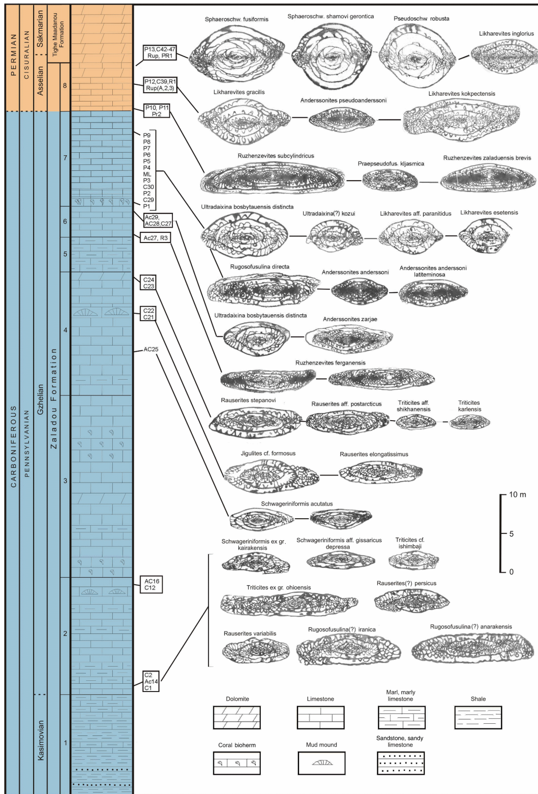
Figure 2. Stratigraphic column and fusulinid distribution.
