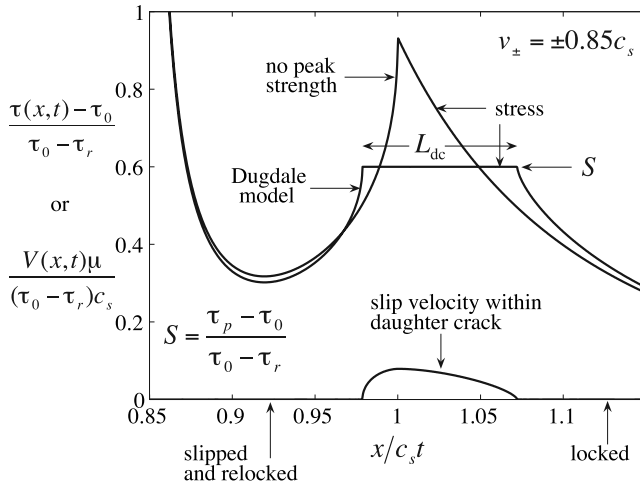
Figure 4. Solution to the self-similar Dugdale model, in which the stress field adjacent the S wave stress peak is limited to the peak strength, causing the formation of a daughter crack. Slip velocity within the daughter crack is also shown.
