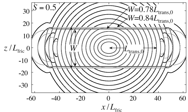
Figure 8. Rupture front contours illustrating the critical fault width ( W \approx 0.8 L_{\text{trans},0} ) for S = 0.5 . The contours, defined as the location at which slip reaches the weakening displacement, \Delta_u = d_0 , are plotted every 60 time steps [ = 3.6585 L_{\text{fric}}/c_s ] from t = 0 (the initial static solution). Shown are contours from ruptures on an unbounded fault (black) and on two finite-width faults (light and dark gray).
