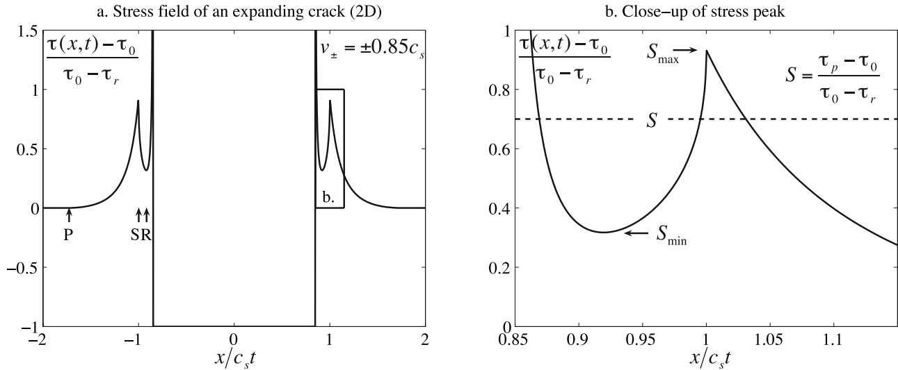
Figure 1. (a) Stress field surrounding a self-similarly expanding sub-Rayleigh rupture, with arrows marking the arrival of the P, S, and Rayleigh waves. (b) Close-up of the region near the S wave stress peak. Imposing a peak strength, \tau_p , (nondimensionally a value of the seismic S ratio, appearing graphically as a horizontal dashed line on this plot) forces the growth of a daughter crack. The length of the daughter crack, L_{dc} , can be estimated as the extent of the region for which \tau(x, t) > \tau_p . Formation of the daughter crack occurs only when S < S_{\max} ; S_{\max} is associated with the maximum value of \tau(x, t) propagating at the S wave speed. S_{\min} is similar value associated with the level of the local minimum between the main rupture front and the daughter crack.
