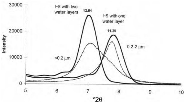
Figure 5. Comparison of XRD patterns of two different size fractions (0–0.2 and 0.2–2 \mu\text{m} ) recorded in an air-dried state with the Newmod ® computer model (bold lines) of mixed-layer I-S clay with one and two layers of water molecules in the expandable interlayers, respectively
