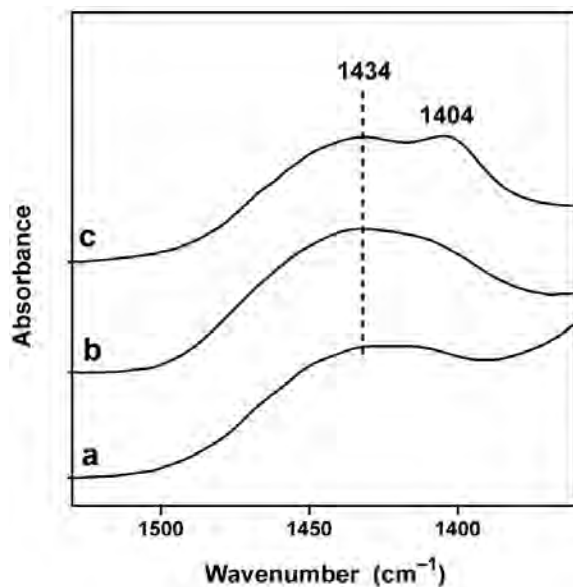
Figure 7. DRIFT spectrum of the undiluted sample (a); of the sample diluted with KBr and ground slightly (b); and of the sample heated at 300^\circ\text{C} overnight, diluted with KBr and ground (c).
