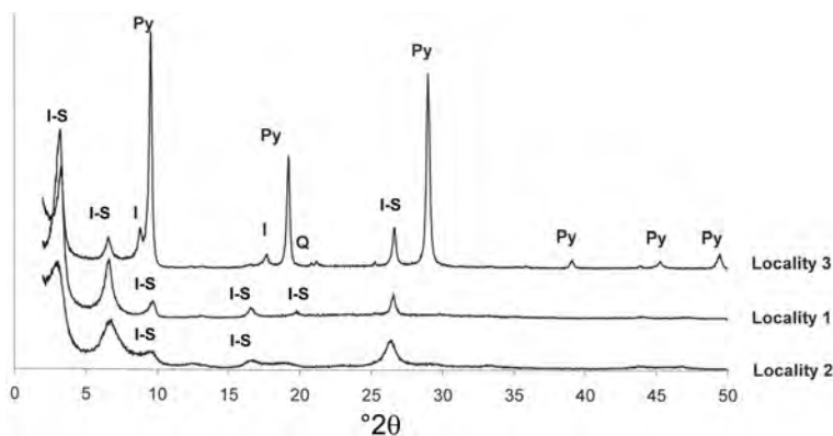
Figure 3. XRD patterns of the <2 µm clay fraction from oriented specimens saturated by EG from the studied localities. I-S – mixed-layer illite-smectite, Py – pyrophyllite, I – illite, Q – quartz.
