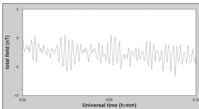
Fig. 2. Observed record from a free-floating magnetometer showing the individual magnetic signals of successive ocean swells, with a typical peak to peak range of 5 nT, from Lilley et al. (2004). Spectral analysis shows the signal to have a sharp spectral peak at 13 s, typical for swells along the south coast of Australia which are generated by storms in the Southern Ocean. According to equation (9), the observed signal indicates a wave height of about 2 m.
