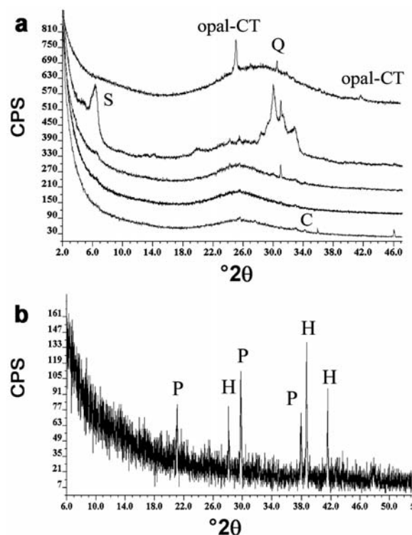
Figure 4. XRD patterns of sinter from each zone: (a) opal-A is represented by the broad central peak around 25^\circ 2\theta or 4.03 Å. The upper pattern is of the spicular zone, then altered, crustal, dark/light laminated, and dark laminated at the bottom. Opal-CT, smectite (S), quartz (Q), and calcite (C) were also identified. (b) Dark mm-sized grains of pyrite (P) and hematite (H) found within the altered zone. CoK\alpha radiation.
