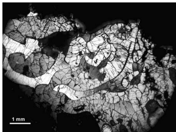
Fig. 6. Sinuous, quasi-granulitic texture of olivine and pyroxene grains in MET 78008. This is most likely a result of significant annealing. X-nicols.
