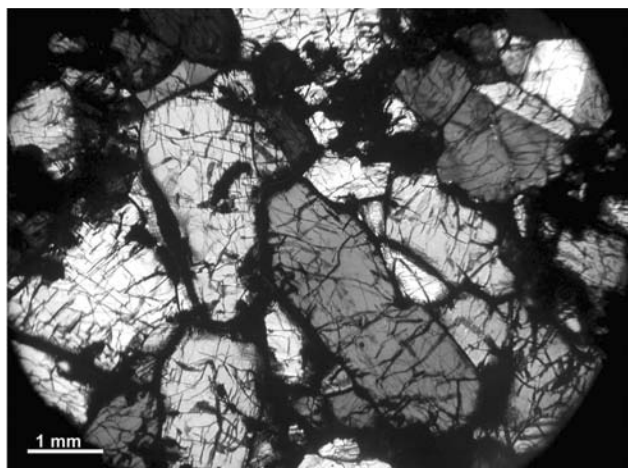
Fig. 1. Typical ureilite texture in ALH 77257 consisting of coarse olivine and pyroxene grains (light gray) with interstitial carbonaceous material (black). Many silicate grain boundaries form 120° triple junctions. X-nicols.
