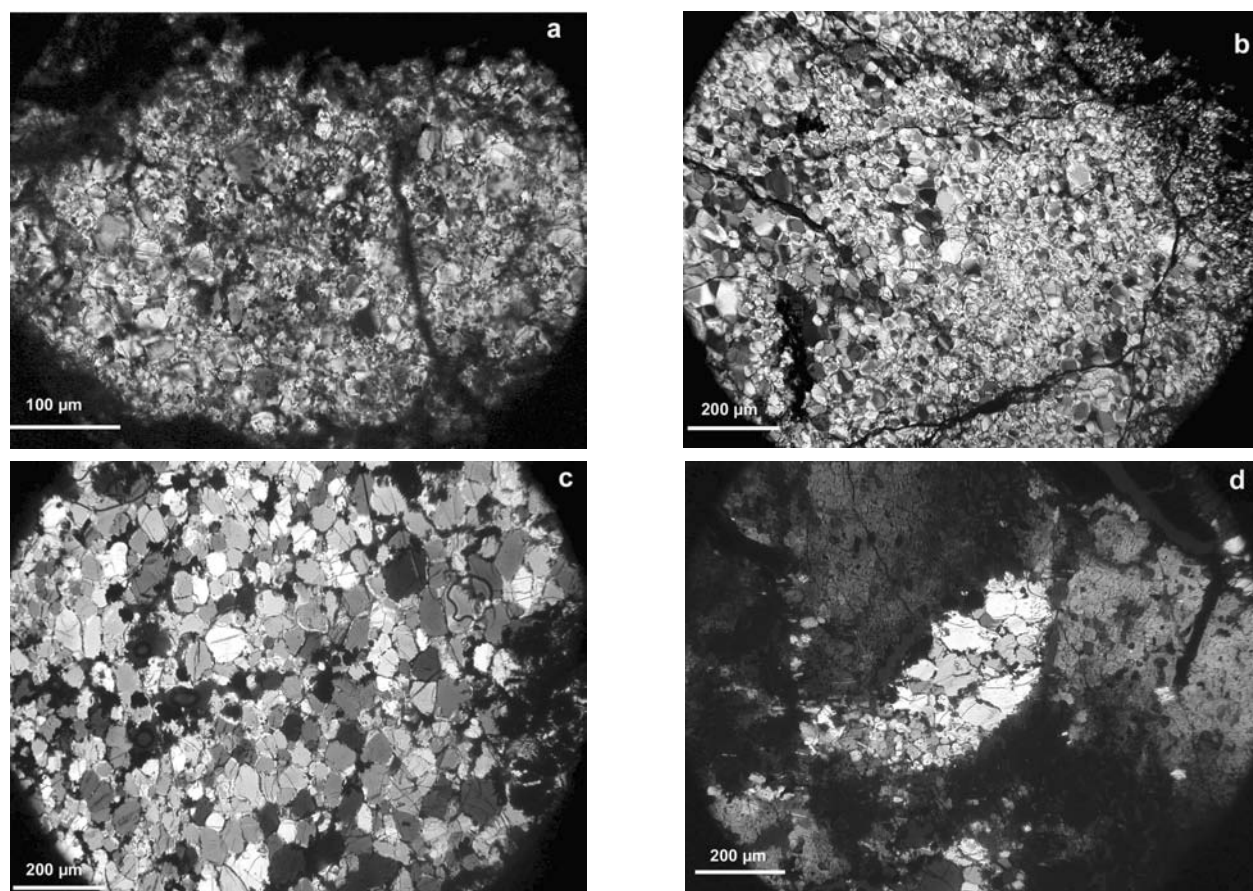
Fig. 4. Mosaicized olivine in ureilites. a) Olivine aggregate in EET 87720 formed from an annealed mosaicized olivine grain. Numerous relatively coarse individual unstrained crystals compose the aggregate. X-nicols. b) Olivine aggregate in GRA 95205 formed from an annealed mosaicized olivine grain. Numerous, randomly oriented, unstrained olivine crystals are evident. X-nicols. c) Numerous, moderately coarse unstrained olivine crystals with random orientations within a large olivine aggregate in ALH 81101. X-nicols. d) Small olivine aggregate (light gray; center) in ALH 81101 composed of unstrained individual olivine crystals. The aggregate formed from a mosaicized olivine grain. The aggregate is embedded within a large pigeonite grain with undulose extinction (dark to medium gray). X-nicols.
