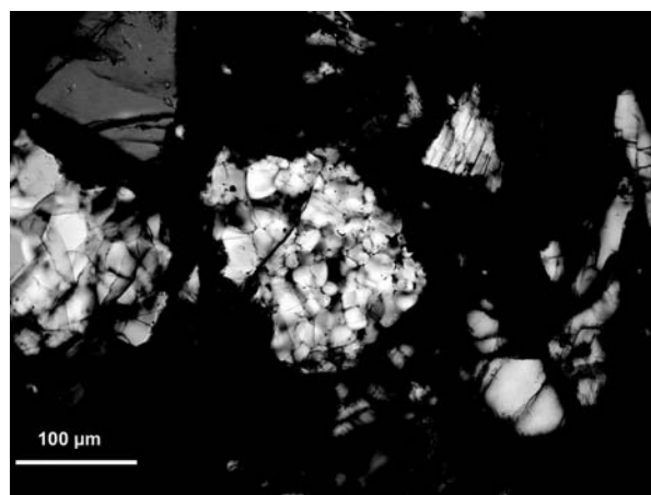
Fig. 7. Olivine aggregate in the clastic portion of the EET 83309 polymict breccia. The aggregate probably formed from a mosaicized olivine grain by annealing. Individual olivine crystals within the aggregate exhibit undulose extinction, indicating that the aggregate was shocked after it was annealed. X-nicols.
