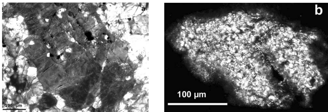
Fig. 3. Mosaicized olivine grains in ordinary chondrites. a) Mottled, mosaicized olivine grain in the shock stage S5 fall Alfianello (L6). The grain consists of small, poorly defined domains with slightly different extinction angles. X-nicols. b) Olivine aggregate embedded in the melt fraction of the Rose City H5 impact-melt breccia. The aggregate consists of small, individual unstrained olivine crystals and seems to have formed from a mosaicized olivine grain by annealing. X-nicols.
