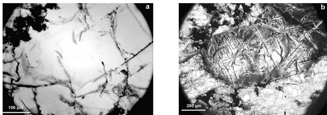
Fig. 5. By-products of annealing. a) Short curvilinear trails of tiny opaque blebs (black) sealed within healed fractures in an olivine grain (light gray) in Nova 001. Transmitted light. b) Reduction rims (dark, dusty regions) at the edges of an olivine grain (center) in ALH 84136. The reduced regions, which cover more than half of the grain, are composed of numerous tiny blebs of low-Ni metallic Fe. Transmitted light.
