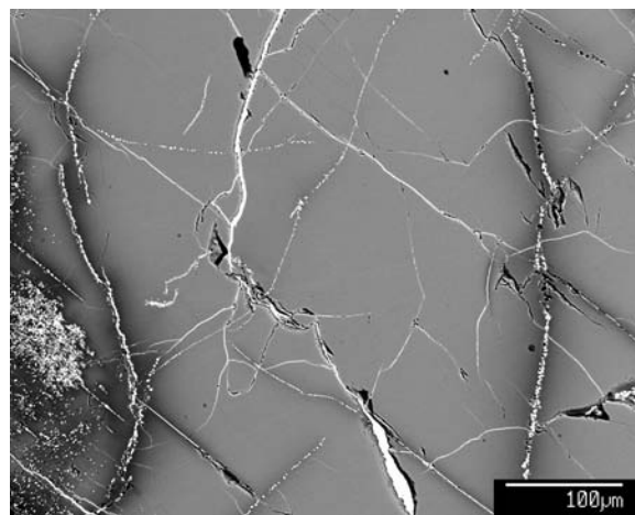
Fig. 2. Silicate darkening in a portion of a Fa13.8 olivine grain (light gray) in ALH 77257. The left edge of the grain is a reduction rim with numerous low-Ni metallic Fe blebs (white). Some curvilinear trails of metal blebs are flanked by dark-gray-shaded olivine of lower FeO content; these trails also seem to have formed by reduction. Many of the small opaque trails contain metal and rare sulfide grains; these trails formed by shock-injection of metal and sulfide into fractures in the olivine. The continuous white trails through the olivine are terrestrial weathering veins containing limonite. BSE image.
