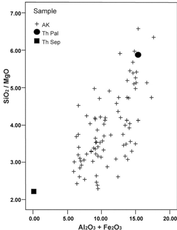
Figure 6. Chemical composition (ratio \text{SiO}_2/\text{MgO} vs. (\text{Al}_2\text{O}_3 + \text{Fe}_2\text{O}_3) (%)) of the particles analyzed by AEM. Theoretical formulae for palygorskite (●) and sepiolite (■) are also plotted.
