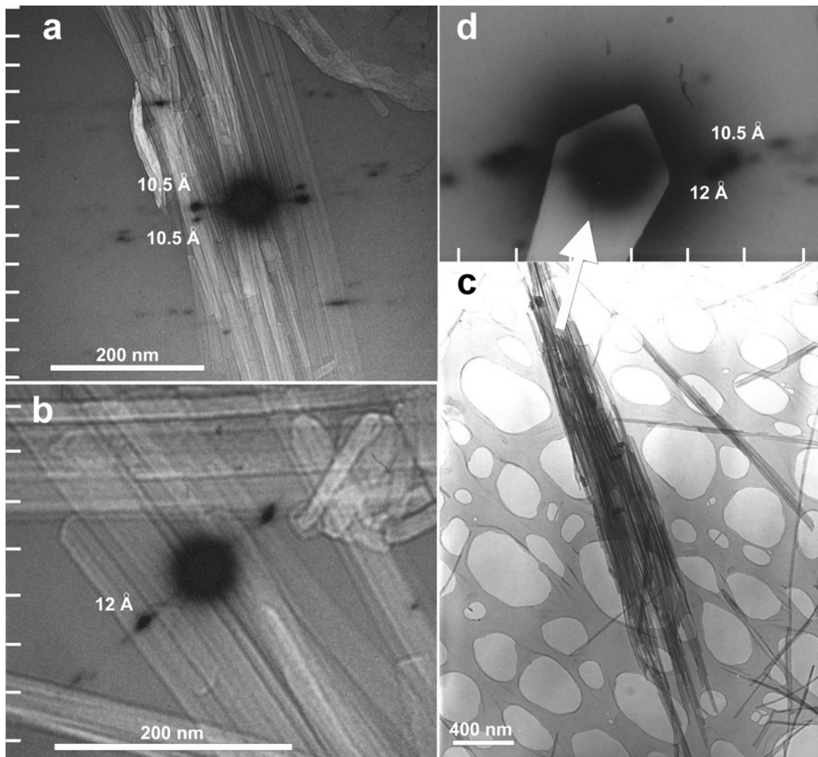
Figure 5. TEM images. (a,b) Superimposed negatives (TEM image and SAED spots) on the image. Camera length ( L ) = 800 mm, \lambda = 0.0025 nm. Camera constant ( L\lambda ) = 20.1 in all SAED images. There are two graphic scales: the vertical scale corresponds to the SAED image (1 mm between bars) and the horizontal scale corresponds to the TEM image. (a) There are two 110 electron diffraction spots corresponding to two different bundles of fibers (10.5 Å) of palygorskite which form a small angle, as can be seen in the image of the aggregate. (b) Bundle of fibers of sepiolite and 110 SAED spots from sepiolite fibers (12 Å). (d) Two different 110 SAED spots from sepiolite and palygorskite fibers (10.5 and 12 Å) corresponding to two contiguous fibers that form a small angle in a same bundle. Scale: 1 mm between bars. (c) Bundles of sepiolite palygorskite.
