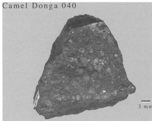
Fig. 12. Camel Donga 040, a unique mixture of pre- and post-metamorphic lithologies related to the CV chondrites.
