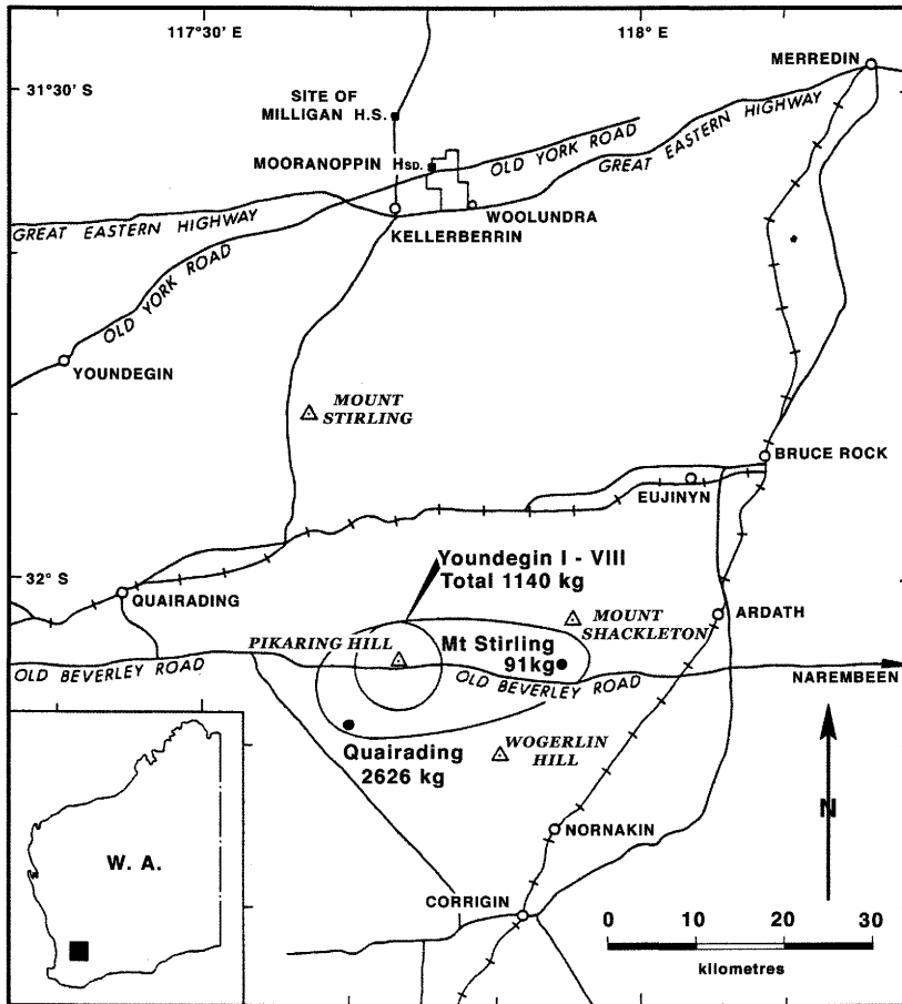
Fig. 1. Map showing the location of masses comprising the Youndegin meteorite shower in Western Australia (after Cleverly & Cleverly 1990).
