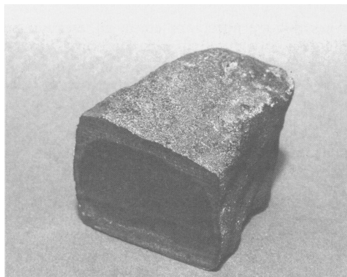
Fig. 8. Main mass of the unique Mulga (west) C5 chondrite, the first carbonaceous chondrite found in the Nullarbor.
