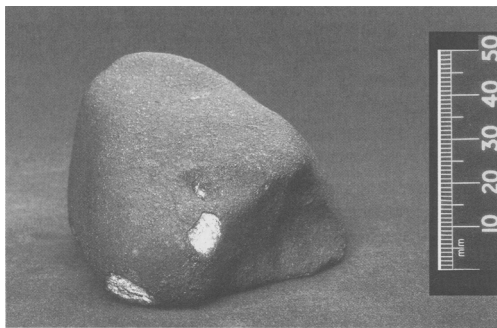
Fig. 6. The Binningup H5 chondrite (weighing 488.1 g) that fell at 10:10 a.m. on the 30 September 1984, after the appearance of a brilliant fireball accompanied by sonic phenomena.
