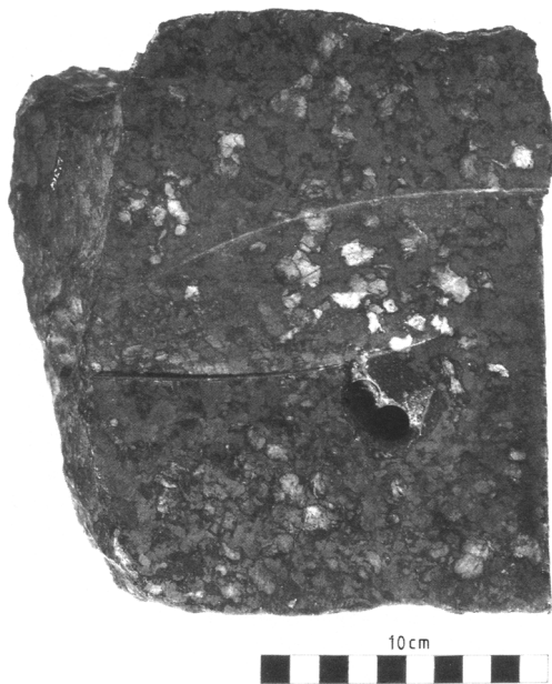
Fig. 4. Cut face of the first mass of Bencubbin found in 1930. A large ordinary chondritic inclusion (dark patch) has been sampled by coring.
