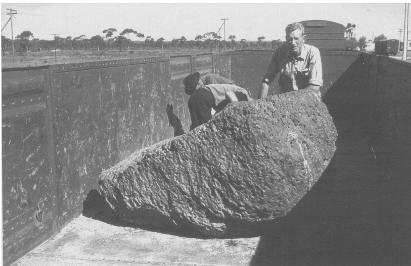
Fig. 7. Main mass (11.5 t) of the Mundrabilla meteorite on route to the Western Australian Museum (W.H. Cleverly centre).
