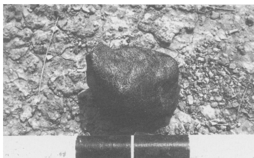
Fig. 9. Mass of the Camel Donga eucrite shower as found on the Nullarbor Plain (5 cm scale).
