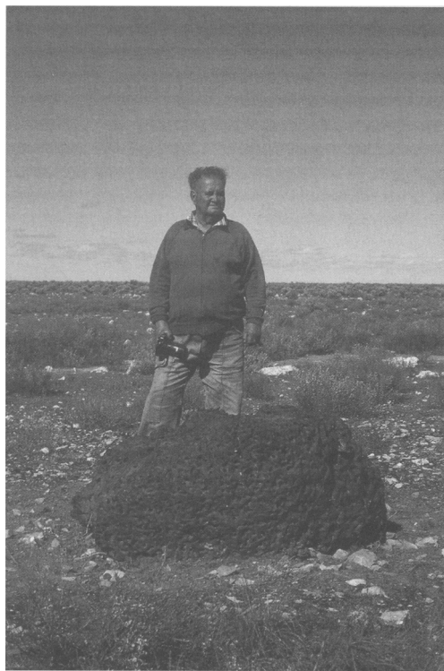
Fig. 10. The 3.5 t mass of the Mundrabilla meteorite found on the Nullarbor by A.J. Carlisle in 1988.
