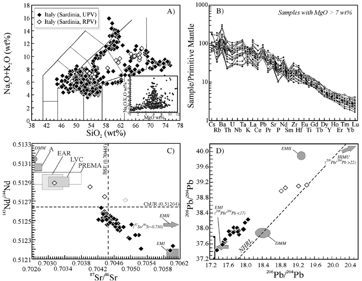
Fig. 8. A) Total alkali vs. silica diagram (TAS; le Maitre, 2002 ); B) primitive mantle ( Sun and McDonough, 1989 ) normalised incompatible element diagram; C) ^{143}\text{Nd}/^{144}\text{Nd} vs. ^{87}\text{Sr}/^{86}\text{Sr} diagram; D) ^{208}\text{Pb}/^{204}\text{Pb} vs. ^{206}\text{Pb}/^{204}\text{Pb} diagram for igneous rocks from Sardinia. UPV = unradiogenic Pb volcanic group (black diamonds; Lustrino et al., 2000 ); RPV = radiogenic Pb volcanic group (white diamonds; Lustrino et al., 2000 ). Data sources: UPV ( Brotzu et al., 1969 ; Beccaluva et al., 1973, 1974, 1975 ; Deriu et al., 1973 ; Assorgia et al., 1976 ; Cioni et al., 1982 ; Rutter, 1987 ; Di Battistini et al., 1990 ; Montanini et al., 1994 ; Lustrino et al., 1996, 2000, 2002, 2004a, 2007 ; Gasparini et al., 2000 ; Godano, 2000 ; Lustrino, 1999, 2000b ; Fedele et al., in press ; this study); RPV ( Brotzu et al., 1975 ; Lustrino et al., 2000, 2007 ). Abbreviations as in Fig. 2.
