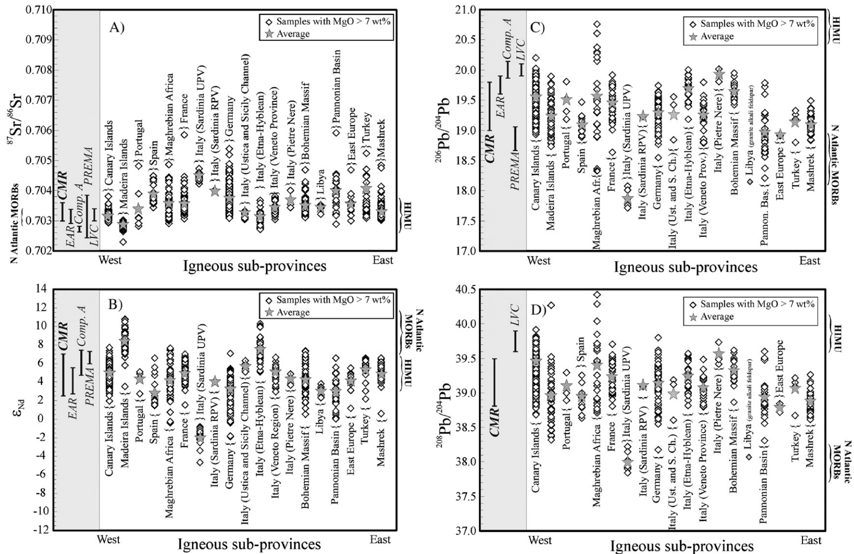
Fig. 14. a) ^{87}\text{Sr}/^{86}\text{Sr} ; b) \epsilon_{\text{Nd}} ; c) ^{206}\text{Pb}/^{204}\text{Pb} ; d) ^{208}\text{Pb}/^{204}\text{Pb} vs. geographic location for the most primitive (MgO > 7 wt.%) mafic magmatic rocks of the CiMACI province. Stars = average composition for each district. For data sources see the captions of Figs. 2–12. EAR = European Asthenospheric Reservoir (Granet et al., 1995); Comp. A = Component A (Wilson and Downes, 1991); PREMA = Prevalent Mantle (Wörner et al., 1986); LVC = Low Velocity Component (Hoernle et al., 1995); CMR = Common Mantle Reservoir.
