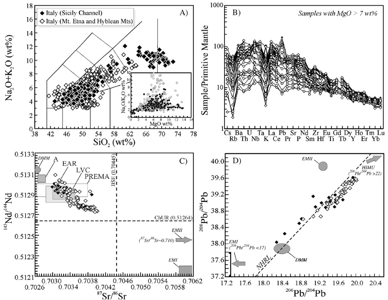
Fig. 7. A) Total alkali vs. silica diagram (TAS; le Maitre, 2002); B) primitive mantle (Sun and McDonough, 1989) normalised incompatible element diagram; C) ^{143}\text{Nd}/^{144}\text{Nd} vs. ^{87}\text{Sr}/^{86}\text{Sr} diagram; D) ^{208}\text{Pb}/^{204}\text{Pb} vs. ^{206}\text{Pb}/^{204}\text{Pb} diagram for igneous rocks from Mt. Etna and Hyblean Mts. (Italy; white diamonds), and the islands of Ustica, Pantelleria and Linosa in the Sicily Channel (Italy; black diamonds). Data sources: Mt. Etna (Carter and Civetta, 1977; Cristofolini et al., 1984, 1991; Tanguy and Clocchiatti, 1984; Armienti et al., 1988, 1989, 1994, 2004; Corsaro and Cristofolini, 1993, 1996; Finocchiaro, 1994; Treuil and Joron, 1994; Condomines et al., 1995; Tonarini et al., 1995; D'Orazio et al., 1997; Tanguy et al., 1997; Clocchiatti et al., 1998 this study); Hyblean Mts. (Carter and Civetta, 1977; Tonarini et al., 1996; Beccaluva et al., 1998; Trua et al., 1998; Bianchini et al., 1998, 1999; Di Grande et al., 2002); Ustica (Cinque et al., 1988; Trua et al., 2003; Peccerillo, 2005); Pantelleria (Romano, 1968; Civetta et al., 1984, 1998; Esperança and Crisci, 1995; Avanzinelli et al., 2004; Ferla and Meli, 2006); Linosa (Barberi et al., 1969; Calanchi et al., 1989; Rossi et al., 1996; Civetta et al., 1998; Bindi et al., 2002; Peccerillo, 2005); Sicily Channel (Beccaluva et al., 1981; Calanchi et al., 1989; Rotolo et al., 2007). Abbreviations as in Fig. 2.
