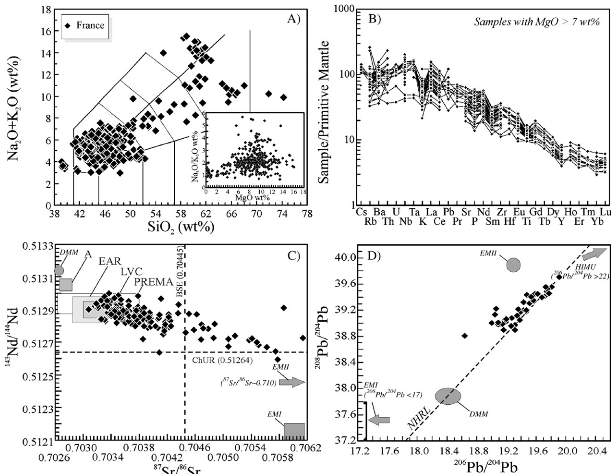
Fig. 5. A) Total alkali vs. silica diagram (TAS; le Maitre, 2002); B) primitive mantle (Sun and McDonough, 1989) normalised incompatible element diagram; C) 143 Nd/ 144 Nd vs. 87 Sr/ 86 Sr diagram; D) 208 Pb/ 204 Pb vs. 206 Pb/ 204 Pb diagram for igneous rocks from France. Data sources: Wimmenauer, 1964; Baubron and Demange, 1982; Alibert et al., 1983; Condomines et al., 1982; Downes, 1984, 1987; Chauvel and Jahn, 1984; Dautria and Liotard, 1990; Briot et al., 1991; Liotard et al., 1988, 1991, 1995, 1999; Wilson and Downes, 1991; Wilson et al., 1995a; Sørensen et al., 1999; Lenoir et al., 2000; Legendre et al., 2001; Wilson and Patterson, 2001; Pilet et al., 2002, 2005; Dautria et al., 2004; this study. Abbreviations as in Fig. 2.
