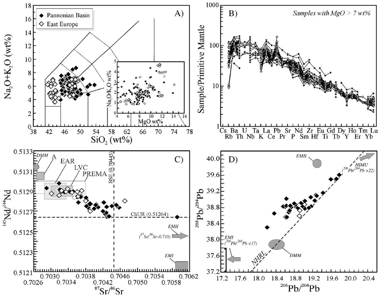
Fig. 11. A) Total alkali vs. silica diagram (TAS; le Maitre, 2002 ); B) primitive mantle ( Sun and McDonough, 1989 ) normalised incompatible element diagram; C) 143 Nd/ 144 Nd vs. 87 Sr/ 86 Sr diagram; D) 208 Pb/ 204 Pb vs. 206 Pb/ 204 Pb diagram for igneous rocks from Pannonian Basin (black diamonds) and East Europe (Serbia, Bulgaria and Macedonia; white diamonds). Data sources: Pannonian Basin ( Salters et al., 1988 ; Embey-Isztin et al., 1993 ; Ivan and Hovorka, 1993 ; Harangi et al., 1994, 1995a,b ; Dobosi et al., 1995 ; Downes et al., 1995a,b ; Rosenbaum et al., 1997 ; Seghedi et al., 2004b ); East Europe ( Marchev et al., 1992, 1997, 1998b ; Jovanovic et al., 2001 ; Cvetkovic et al., 2004 ). Abbreviations as in Fig. 2.
