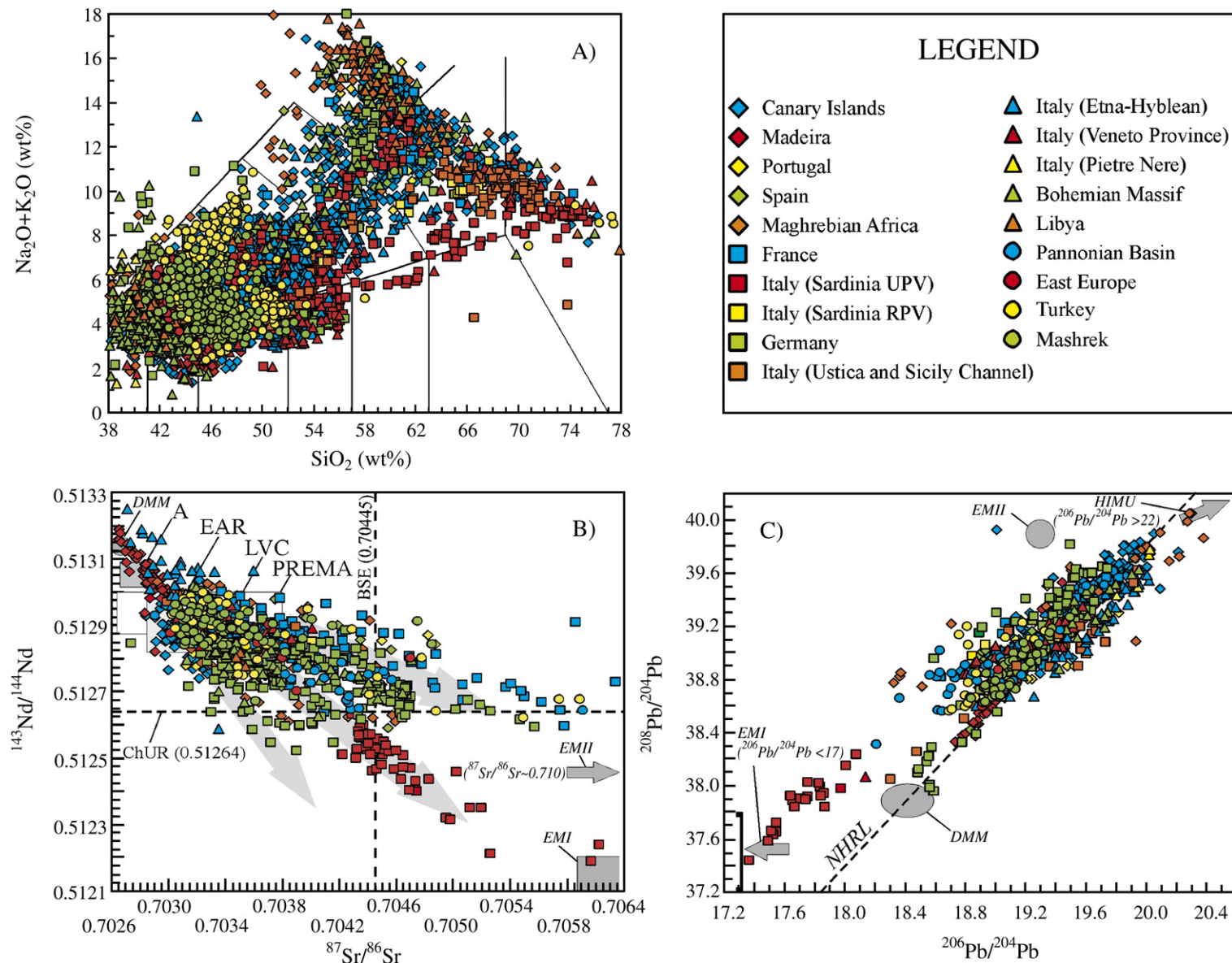
Fig. 13. a) Total alkali vs. silica diagram (TAS; le Maitre, 2002); b) ^{143}\text{Nd}/^{144}\text{Nd} vs. ^{87}\text{Sr}/^{86}\text{Sr} diagram; c) ^{208}\text{Pb}/^{204}\text{Pb} vs. ^{206}\text{Pb}/^{204}\text{Pb} diagram for the entire CiMACI province, including both primitive and differentiated magmatic rocks. For sources of data see the captions of Figs. 2–12.
