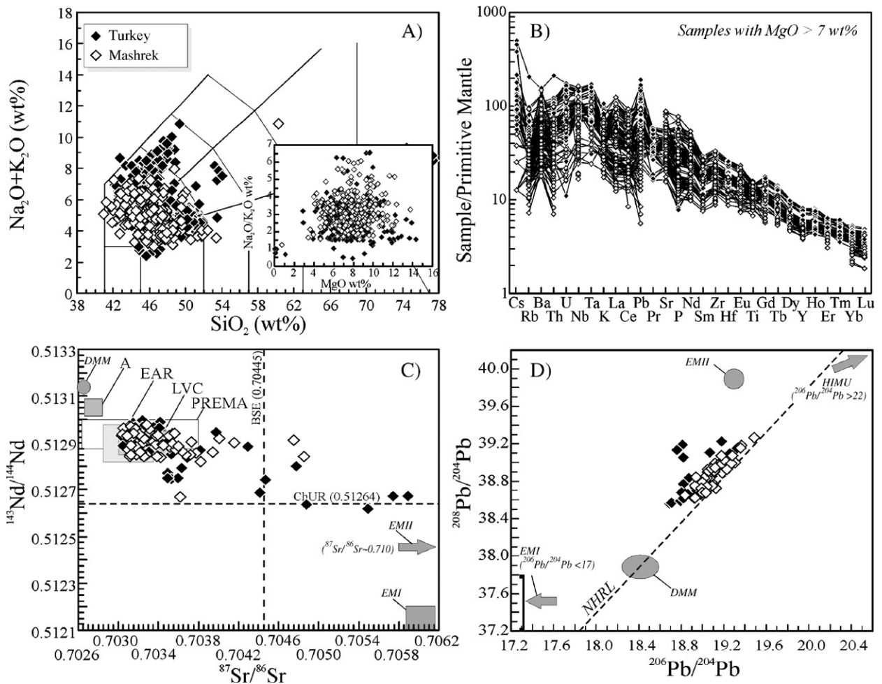
Fig. 12. A) Total alkali vs. silica diagram (TAS; le Maitre, 2002 ); B) primitive mantle ( Sun and McDonough, 1989 ) normalised incompatible elements diagram; C) 143 Nd/ 144 Nd vs. 87 Sr/ 86 Sr diagram; D) 208 Pb/ 204 Pb vs. 206 Pb/ 204 Pb diagram for igneous rocks from Turkey (black diamonds) and Mashrek (Jordan, Israel, Syria, Lebanon and Palestine; white diamonds). Data sources: Turkey ( Innocenti et al., 1982, 2005 ; Çapan et al., 1987 ; Pearce et al., 1990 ; Guleç, 1991 ; Aydar et al., 1995 ; Notsu et al., 1995 ; Parlak et al., 1997, 2001 ; Polat et al., 1997 ; Wilson et al., 1997 ; Genç, 1998 ; Yilmaz and Polat, 1998 ; Aldanmaz et al., 2000, 2006 ; Aldanmaz, 2002 ; Alici et al., 2001, 2002 ; Alici Sen et al., 2004 ; Agostini et al., 2007 ; this study); Mashrek ( Barberi et al., 1979 ; Altherr et al., 1990 ; Mouty et al., 1992 ; Stein and Hofmann, 1992 ; Sharkov et al., 1994, 1996 ; Weinstein et al., 1994, 2006 ; Fediuk and Al Fugha, 1999 ; Bertrand et al., 2003 ; Ibrahim et al., 2003 ; Shaw et al., 2003 ; Abdel-Rahman and Nassar, 2004 ; Ibrahim and Al-Malabeh, 2006 ; Krienitz et al., 2006 ; Lustrino and Sharkov, 2006 ). Abbreviations as in Fig. 2.
