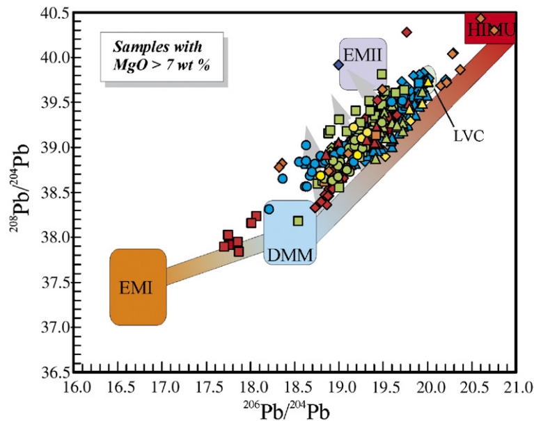
Fig. 17. Variation of ^{208}\text{Pb}/^{204}\text{Pb} vs. ^{206}\text{Pb}/^{204}\text{Pb} for the most primitive ( \text{MgO} > 7 \text{ wt.}\% ) mafic magmatic rocks of the CiMACI province. For data sources see the captions of Figs. 2–12. DMM = Depleted MORB Mantle [average North Atlantic compositions (PETDB database; http://beta.www.petdb.org/ ); Kramers and Tolstikhin, 1997]; HIMU = high MU [ (\text{MU} = \mu = ^{238}\text{U}/^{204}\text{Pb}) Zindler and Hart, 1986]; EMI = Enriched Mantle type I (Zindler and Hart, 1986; Lustrino and Dallai, 2003); EMII = Enriched Mantle type II (Zindler and Hart, 1986); EAR = European Asthenospheric Reservoir (Granet et al., 1995); Comp. A = Component A (Wilson and Downes, 1991); PREMA = Prevalent Mantle (Wörner et al., 1986); LVC = Low Velocity Component (Hoernle et al., 1995). The Pb isotopic composition of the most mafic CiMACI rocks requires the involvement of at least four mantle end-members: mixing between HIMU-like and DMM-like compositions is not able to explain the spread of isotopic data. The involvement of EM components is therefore required. As in Figs. 15 and 16, only the Sardinian rocks seem to reflect a mixing between DMM and EMI end-members, with very limited involvement of HIMU. Grey arrows indicate the effect of mixing between HIMU-DMM melts and EMII-like lithospheric components.
