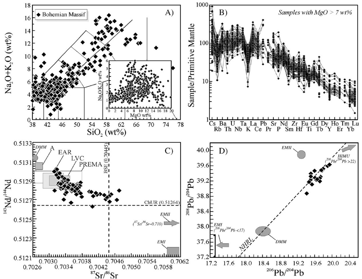
Fig. 10. A) Total alkali vs. silica diagram (TAS; le Maitre, 2002 ); B) primitive mantle ( Sun and McDonough, 1989 ) normalised incompatible element diagram; C) 143 Nd/ 144 Nd vs. 87 Sr/ 86 Sr diagram; D) 208 Pb/ 204 Pb vs. 206 Pb/ 204 Pb diagram for igneous rocks from Bohemian Massif. Data sources: Wimmenauer, 1964 ; Shrbeny, 1979, 1980, 1982 ; Alibert et al., 1983, 1987 ; Ulrych et al., 1988, 1998, 2000a,b, 2002, 2003 ; Blusztajn and Hart, 1989 ; Bendl et al., 1993 ; Vaneckova et al., 1993 ; Wilson et al., 1995b ; Ulrych and Pivec, 1997 ; Pivec et al., 2003, 2004 ; Ulrych, 1998 ; Randa et al., 2003 ; this study. Abbreviations as in Fig. 2.
