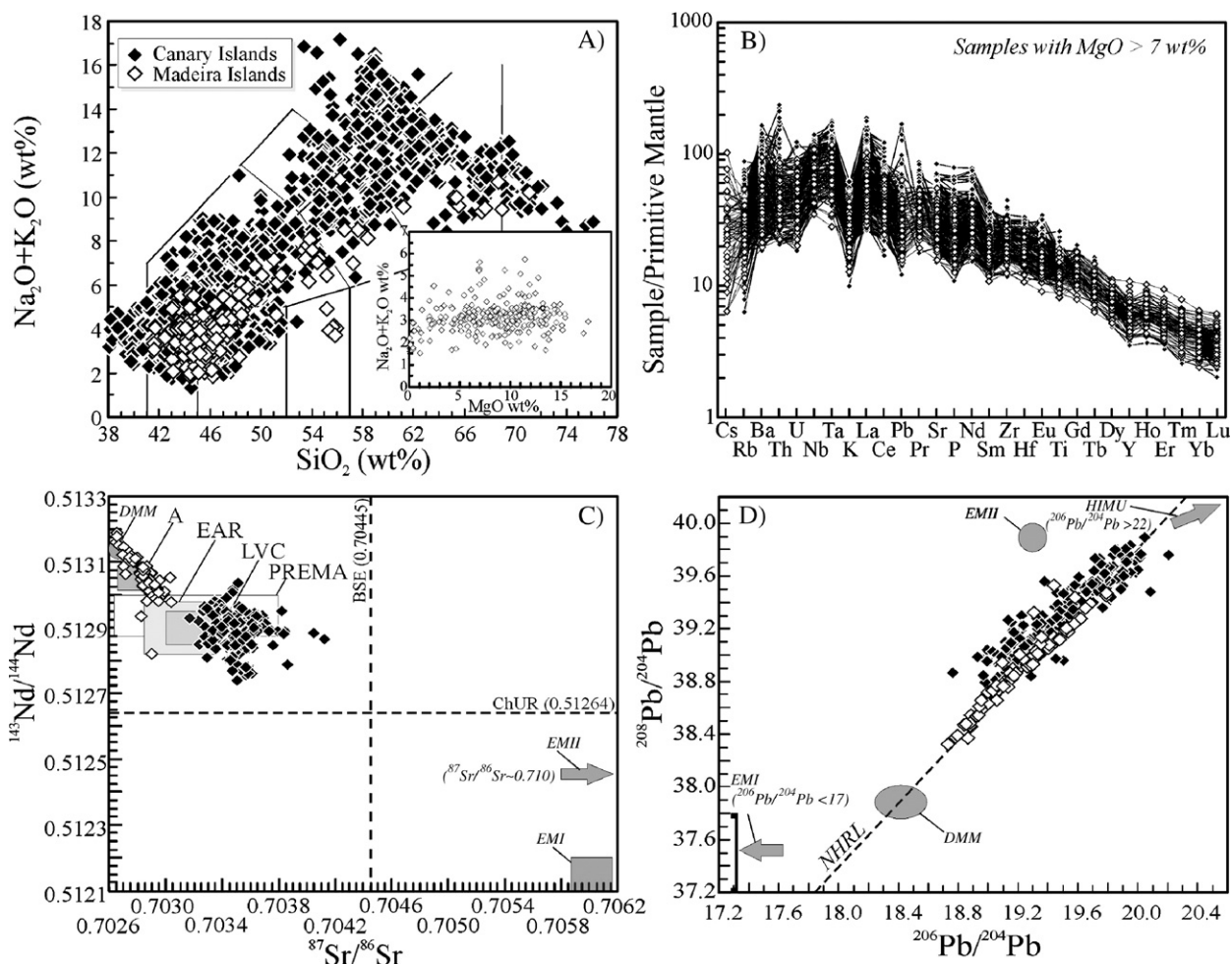
Fig. 2. A) Total alkali vs. silica diagram (TAS; le Maitre, 2002); B) primitive mantle (Sun and McDonough, 1989) normalised incompatible element diagram; C) ^{143}\text{Nd}/^{144}\text{Nd} vs. ^{87}\text{Sr}/^{86}\text{Sr} diagram; D) ^{208}\text{Pb}/^{204}\text{Pb} vs. ^{206}\text{Pb}/^{204}\text{Pb} diagram for igneous rocks from the Canary Islands and seamounts (black diamonds) and Madeira Islands and seamounts (white diamonds). Data for the Canary Islands and seamounts are from the GEOROC database ( http://georoc.mpch-mainz.gwdg.de/georoc/ ) and Geldmacher et al. (2005). References for Madeira islands and seamounts: Aires-Barros et al., 1980; Halliday et al., 1992; Mata et al., 1998; Geldmacher and Hoernle, 2000; Geldmacher et al., 2005; Schwarz et al., 2005. Abbreviations: DMM = Depleted MORB Mantle (Kramers and Tolstikhin, 1997; Workman and Hart, 2005); EMI = Enriched Mantle type 1 (Lustrino and Dallai, 2003); EMII = Enriched Mantle type 2 (Workman et al., 2004); HIMU = high- \mu (where \mu = ^{238}\text{U}/^{204}\text{Pb} ; Hofmann, 2004); A = Component A (Wilson and Downes, 1991); EAR = European Asthenospheric Reservoir (Granet et al., 1995; Wilson and Bianchini, 1999); LVC = Low Velocity Component (Hoernle et al., 1995); PREMA = Prevalent Mantle (Wörmel et al., 1986).
