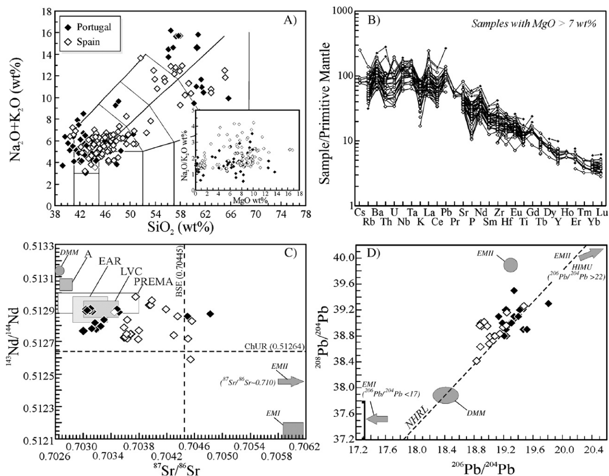
Fig. 3. A) Total alkali vs. silica diagram (TAS; le Maitre, 2002 ); B) primitive mantle ( Sun and McDonough, 1989 ) normalised incompatible element diagram; C) 143 Nd/ 144 Nd vs. 87 Sr/ 86 Sr diagram; D) 208 Pb/ 204 Pb vs. 206 Pb/ 204 Pb diagram for igneous rocks from Portugal (black diamonds) and Spain (white diamonds). Data sources: Portugal ( Rock, 1982 ; Bernard-Griffiths et al., 1997 ; Tavares Martins, 1999 ); Spain ( Alibert et al., 1983 ; Araña et al., 1983 ; Ancochea et al., 1984 ; Lopez Ruiz and Badiola, 1985 ; Capedri et al., 1989 ; Aparicio et al., 1991 ; Martí et al., 1992 ; Aparicio and Garcia, 1995 ; Cebrià and Lopez-Ruiz, 1995 ; Gimeno Torrente, 1995 ; Diaz et al., 1996 ; Neumann et al., 1999 ; Turner et al., 1999 ; Cebrià et al., 2000 ; Ancochea and Huertas, 2002 ; Beccaluva et al., 2004 ; Acosta et al., 2004 ; Duggen et al., 2005 ; this study). Abbreviations as in Fig. 2.
