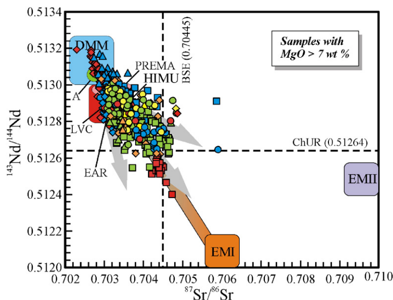
Fig. 15. Variation of ^{143}\text{Nd}/^{144}\text{Nd} vs. ^{87}\text{Sr}/^{86}\text{Sr} for the most primitive ( \text{MgO} > 7 wt.%) mafic magmatic rocks of the CiMACI province. For data sources see the captions of Figs. 2–12. DMM = Depleted MORB Mantle [average North Atlantic compositions (PETDB database; http://beta.www.petdb.org/ ); Kramers and Tolstikhin, 1997]; HIMU = high MU [ (\text{MU} = \mu = ^{238}\text{U}/^{204}\text{Pb}) Zindler and Hart, 1986]; EMI = Enriched Mantle type I (Zindler and Hart, 1986; Lustrino and Dallai, 2003); EMII = Enriched Mantle type II (Zindler and Hart, 1986); EAR = European Asthenospheric Reservoir (Granet et al., 1995); Comp. A = Component A (Wilson and Downes, 1991); PREMA = Prevalent Mantle (Wörner et al., 1986); LVC = Low Velocity Component (Hoernle et al., 1995). BSE = Bulk Silicate Earth estimate; ChUR = Chondritic Uniform Reservoir. Most of the CiMACI rocks are clustered in a relatively restricted Sr–Nd isotopic range (depleted quadrant). Only few mafic rocks have ^{143}\text{Nd}/^{144}\text{Nd} ratios lower than ChUR and virtually all of the CiMACI rocks have ^{87}\text{Sr}/^{86}\text{Sr} ratios lower than BSE. Grey arrows indicate the effect of interaction of asthenosphere-derived melts with lithospheric components characterized by radiogenic Sr and unradiogenic Nd isotopic compositions (pointing towards EMI and EMII end-members).
