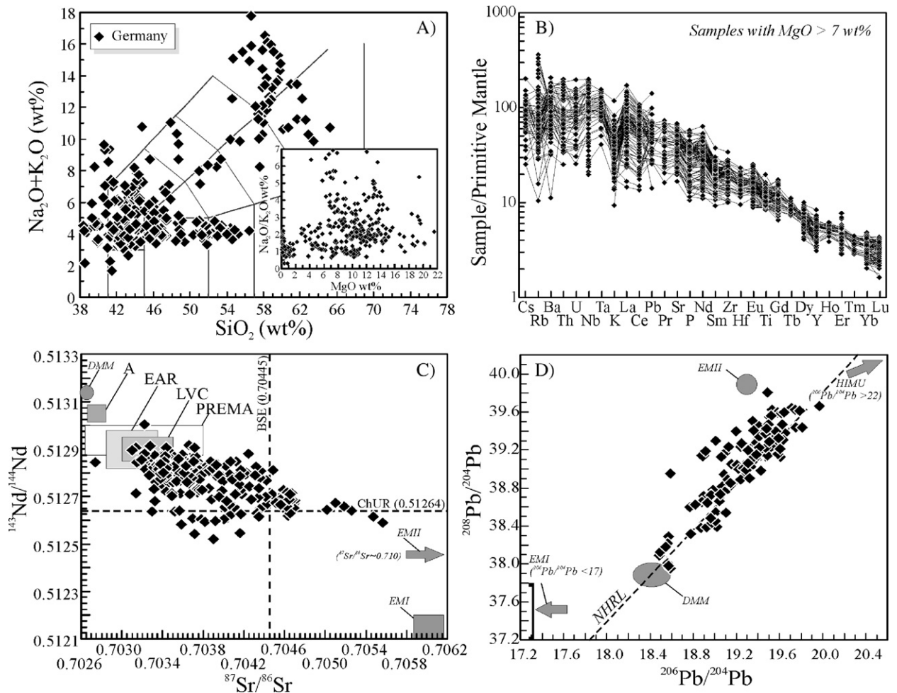
Fig. 9. A) Total alkali vs. silica diagram (TAS; le Maitre, 2002 ); B) primitive mantle ( Sun and McDonough, 1989 ) normalised incompatible element diagram; C) 143 Nd/ 144 Nd vs. 87 Sr/ 86 Sr diagram; D) 208 Pb/ 204 Pb vs. 206 Pb/ 204 Pb diagram for igneous rocks from Germany. Data sources: Wimmenauer, 1964 ; Hoefs and Wedepohl, 1968 ; Duda and Schmincke, 1978 ; Alibert et al., 1983 ; Wörner et al., 1983, 1986, 1987 ; Wörner and Schmincke, 1984 ; Mertes and Schmincke, 1985 ; Wedepohl, 1985, 2000 ; Harmon et al., 1987 ; Hubberten et al., 1988 ; Kramm and Wedepohl, 1990 ; Schleicher et al., 1990, 1991 ; Ehrenberg et al., 1994 ; Wedepohl et al., 1994 ; Hegner et al., 1995 ; Jung, 1995 ; Wilson et al., 1995b ; Dunworth and Wilson, 1998 ; Jung and Masberg, 1998 ; Riley et al., 1999 ; Schreiber et al., 1999 ; Wedepohl and Baumann, 1999 ; Jung and Hoernes, 2000 ; Meyer et al., 2002 ; Bogaard and Wörner, 2003 ; Haase et al., 2004 ; Jung et al., 2005, 2006 ; Fekiacova et al., in press-a,b . Abbreviations as in Fig. 2.
