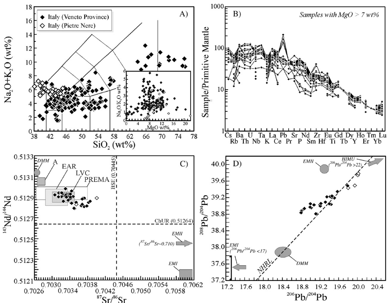
Fig. 6. A) Total alkali vs. silica diagram (TAS; le Maitre, 2002 ); B) primitive mantle ( Sun and McDonough, 1989 ) normalised incompatible element diagram; C) ^{143}\text{Nd}/^{144}\text{Nd} vs. ^{87}\text{Sr}/^{86}\text{Sr} diagram; D) ^{208}\text{Pb}/^{204}\text{Pb} vs. ^{206}\text{Pb}/^{204}\text{Pb} diagram for igneous rocks from Veneto, Italy (black diamonds) and Punta delle Pietre Nere, Italy (white diamonds). Data sources: Veneto ( De Vecchi et al., 1976 ; De Vecchi and Seda, 1995 ; Milani et al., 1999 ; Macera et al., 2003 ; Beccaluva et al., 2007a ); Punta delle Pietre Nere ( Vollmer, 1976 ; Vollmer and Hawkesworth, 1980 ; De Fino et al., 1981 ; De Astis et al., 2006 ). Abbreviations as in Fig. 2 .
