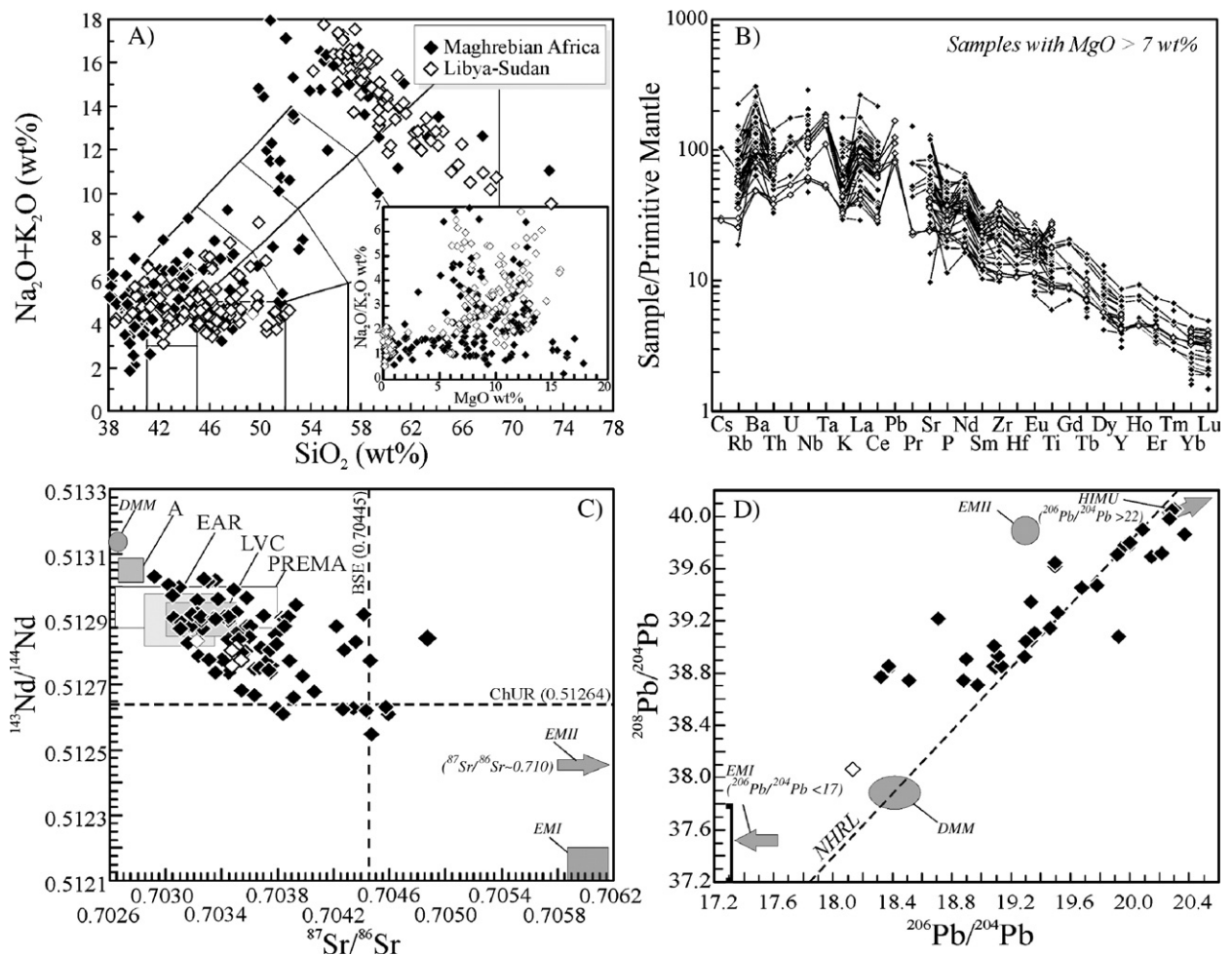
Fig. 4. A) Total alkali vs. silica diagram (TAS; le Maitre, 2002); B) primitive mantle (Sun and McDonough, 1989) normalised incompatible element diagram; C) ^{143}\text{Nd}/^{144}\text{Nd} vs. ^{87}\text{Sr}/^{86}\text{Sr} diagram; D) ^{208}\text{Pb}/^{204}\text{Pb} vs. ^{206}\text{Pb}/^{204}\text{Pb} diagram for igneous rocks from Maghrebian Africa (black diamonds) and Libya (white diamonds). Data sources: Maghrebian Africa (Hernandez and Lepvrier, 1979; Allègre et al., 1981; Berrahma and Hernandez, 1985; Rachdi et al., 1985; Bouabdli et al., 1988; Mokhtari and Velde, 1988; Velde and Rachdi, 1988; Bernard-Griffiths et al., 1991; Bouabdli and Liotard, 1992; Dautria et al., 1992; Berrahma et al., 1993; Semroud et al., 1994; Belanteur et al., 1995; Rachdi et al., 1997; El Bakkali et al., 1998; Maza et al., 1998; El Azzouzi et al., 1999; Ait-Hamou et al., 2000; Coulon et al., 2002; Wagner et al., 2003; Duggen et al., 2005; this paper); Libya (Piccoli, 1970; Almond, 1974; Almond et al., 1974; Busrewil and Wadsworth, 1980a, 1980b; Andre et al., 1991; Atherton et al., 1991; Busrewil and Oun, 1991; Flinn et al., 1991; Conticelli et al., 1995; this study). Abbreviations as in Fig. 2.
