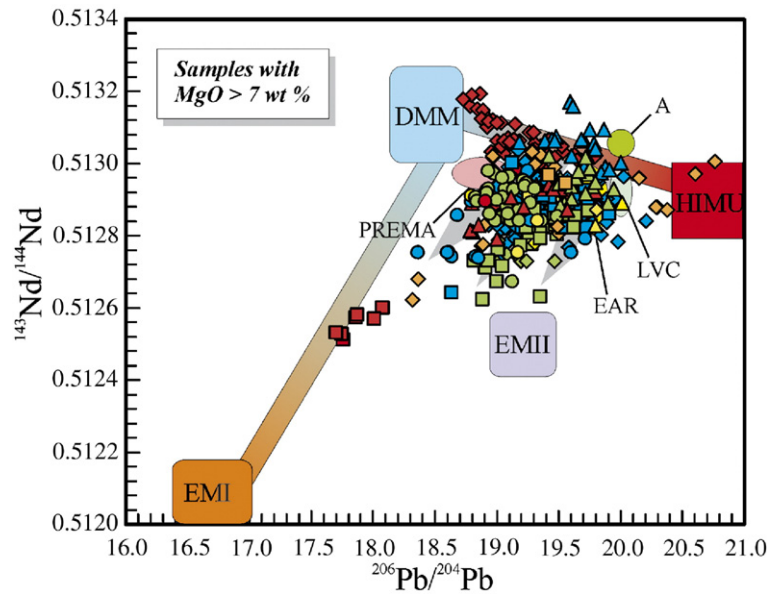
Fig. 16. ^{143}\text{Nd}/^{144}\text{Nd} vs. ^{206}\text{Pb}/^{204}\text{Pb} diagram for the most primitive ( \text{MgO} > 7 \text{ wt } \% ) mafic magmatic rocks of the CiMACI province. References to data sources are given in the captions of Figs. 2–12. DMM = Depleted MORB Mantle [average North Atlantic compositions (PETDB database; http://beta.www.petdb.org/ ); Kramers and Tolstikhin, 1997]; HIMU = high MU [ (\text{MU} = \mu = ^{238}\text{U}/^{204}\text{Pb}) Zindler and Hart, 1986]; EMI = Enriched Mantle type I (Zindler and Hart, 1986; Lustrino and Dallai, 2003); EMII = Enriched Mantle type II (Zindler and Hart, 1986) EAR = European Asthenospheric Reservoir (Granet et al., 1995); Comp. A = Component A (Wilson and Downes, 1991); PREMA = Prevalent Mantle (Wörner et al., 1986); LVC = Low Velocity Component (Hoernle et al., 1995). The range of Nd and Pb isotopic compositions of the most mafic CiMACI rocks indicates the involvement of at least four mantle components: mixing between HIMU-like and DMM-like compositions is not able to explain the spread of isotopic data. The involvement of EM components is therefore required. Only the Sardinian rocks seem to reflect a mixing between DMM and EMI end-members, with very limited involvement of HIMU. Grey arrows indicate the effects of interaction of HIMU-DMM melts with lithospheric components characterized by unradiogenic Nd and mildly radiogenic Pb isotopic compositions (pointing towards EMI and EMII end-members).
