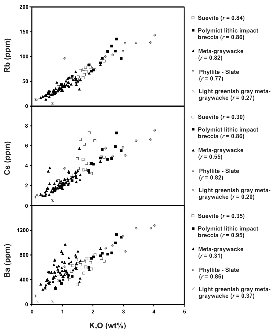
Fig. 5. Binary diagrams comparing the abundances of the trace elements Ba, Cs, and Rb (in ppm) with those of K 2 O content (in wt%), showing the degree of correlation between the abundances of these elements for the different lithologies present in core LB-08A ( r = correlation coefficient).
