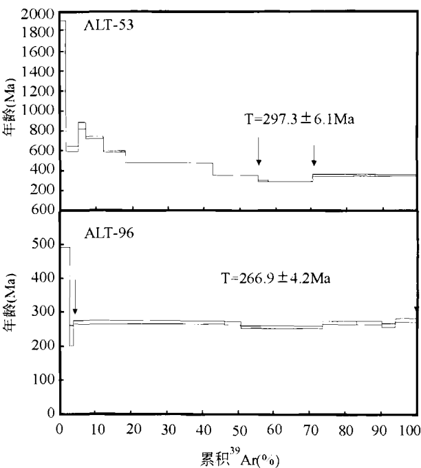
图 2 斜长角闪岩和辉长岩的 40 Ar- 39 Ar 表观年龄 Fig. 2 Plots of the age spectrum of amphibolites and gabbros based on 40 Ar- 39 Ar dating results
