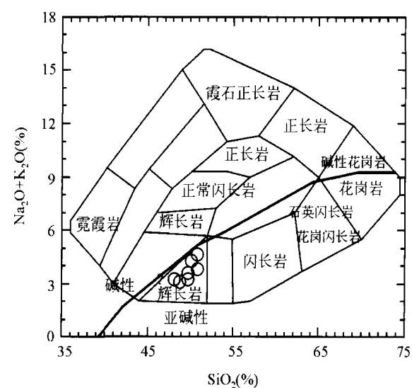
图6 塔尔浪辉长岩 (Na 2 O + K 2 O)-SiO 2 图解 (Cox, 1979) Fig. 6 Na 2 O + K 2 O vs. SiO 2 diagram of Tarlang gabbros
