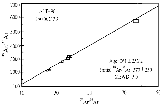
图 3 辉长岩 40 Ar- 39 Ar 等时线年龄 Fig. 3 The isochron age of gabbros based on 40 Ar- 39 Ar dating results
