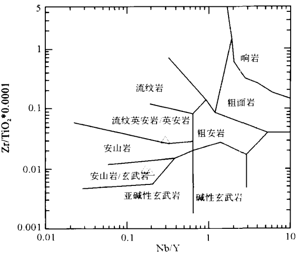
图 5 塔尔浪斜长角闪岩 Zr/TiO 2 -Nb/Y 图解 (Winchester and Floyd, 1976) Fig. 5 Zr/TiO 2 vs. Nb/Y diagram of Tarlang amphibolites
