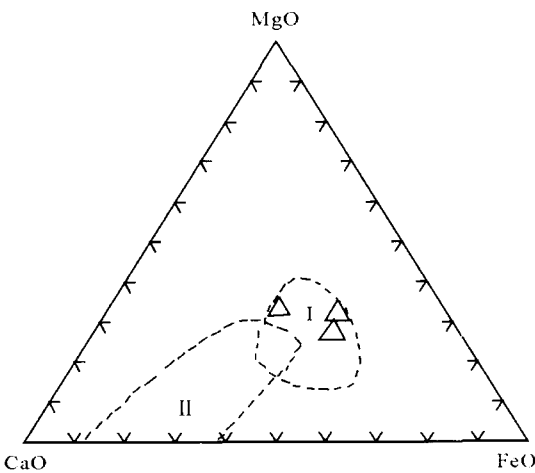
图 4 塔尔浪斜长角闪岩 MgO-CaO-FeO (Walker et al. , 1960) (其中, I 为正斜长角闪岩; II 为负斜长角闪岩) Fig. 4 MgO-CaO-FeO diagram of amphibolites in Tarlang area
