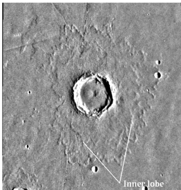
Fig. 7. An impact crater with an uprange forbidden zone ( 18.0^{\circ}\text{N} , 142.5^{\circ}\text{E} , D = 25 km, A = 81^{\circ} ). If erosion resulted in preservation of only the inner lobe of ejecta, then we would probably have classified this crater as type “offset.”
