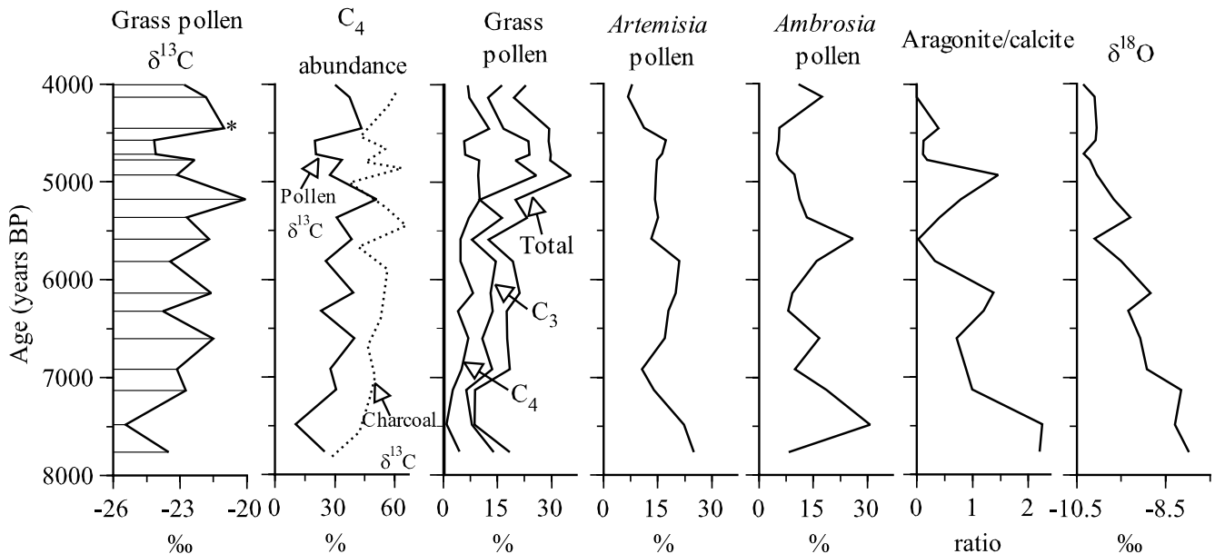
Figure 3 Multiproxy data from the sediments of West Olaf Lake and calcite \delta^{18}\text{O} data from Steel Lake, \sim 120 km east of West Olaf Lake (Nelson et al. , 2004). The grass-pollen \delta^{13}\text{C} data point labelled with * is below the sample/blank \text{CO}_2 area ratio threshold
