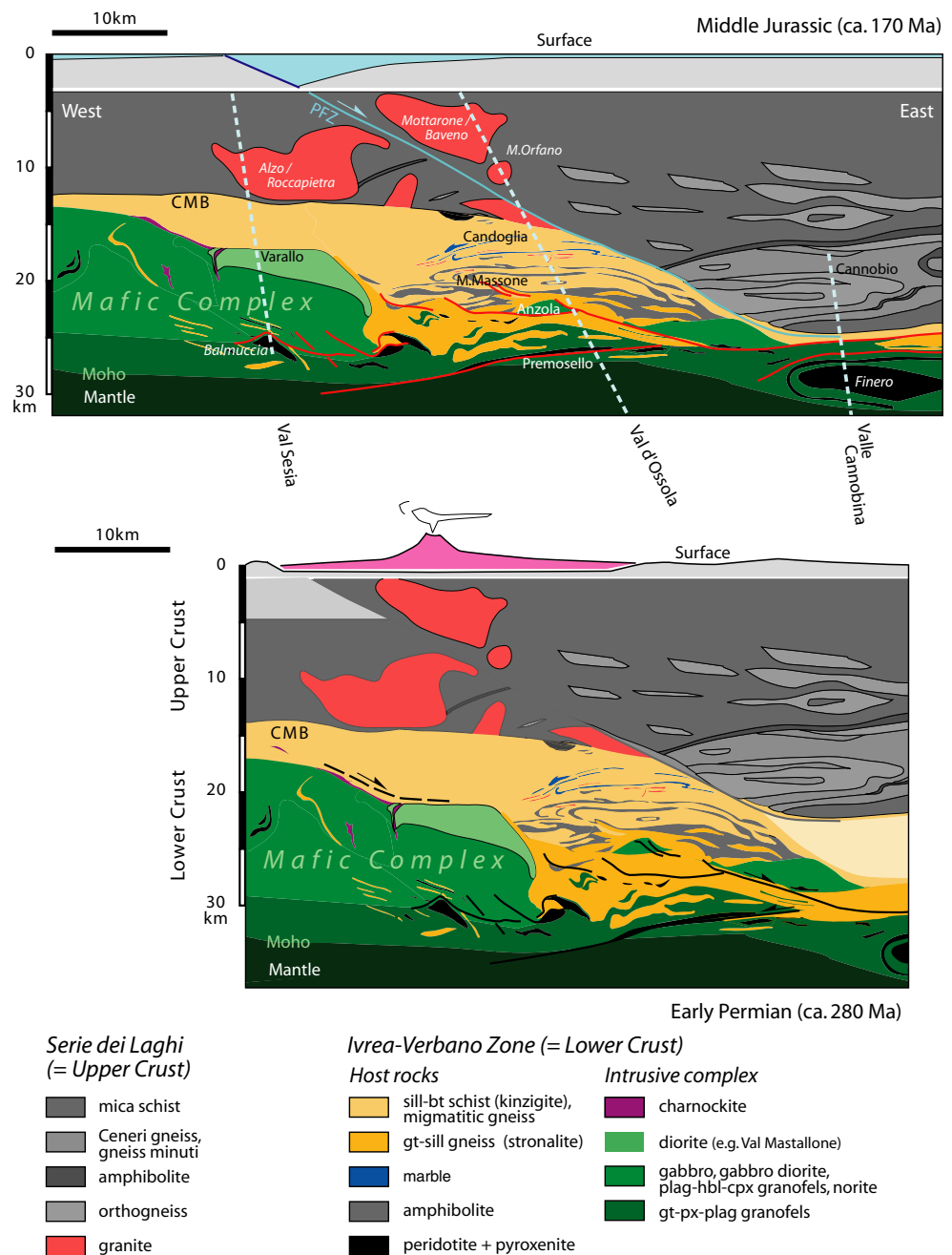
Fig. 5 Tentative schematic reconstruction of Permian crust of the Ivrea-Verbano Zone—Laghi area obtained by retrodeformation of a simplified (reflected) version of the restored cross section in Rutter et al. (1999, 2003). See Fig. 6 for the removal of pre-Alpine deformation
