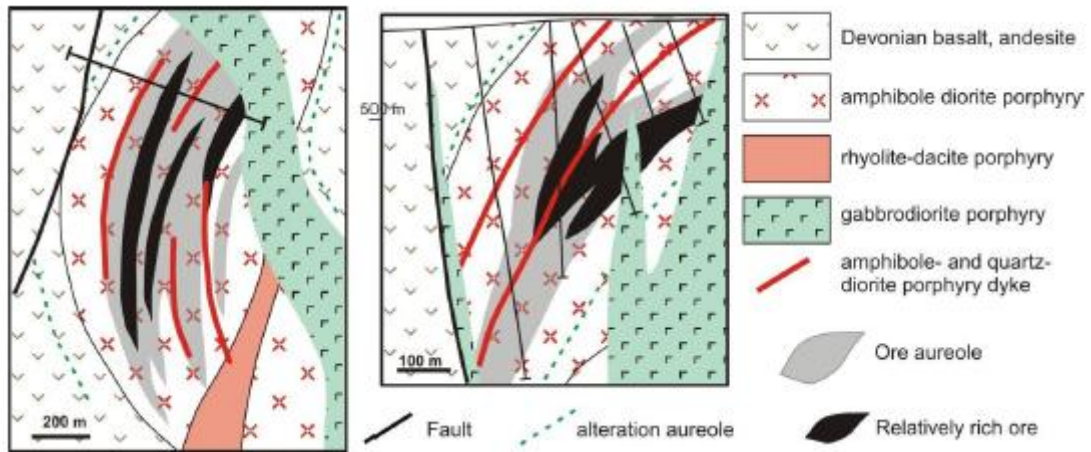
Fig. 2. The Salavat deposit: simplified geological map of the +500m horizon (A) and a cross-section (B), after (Minina, 1982)
