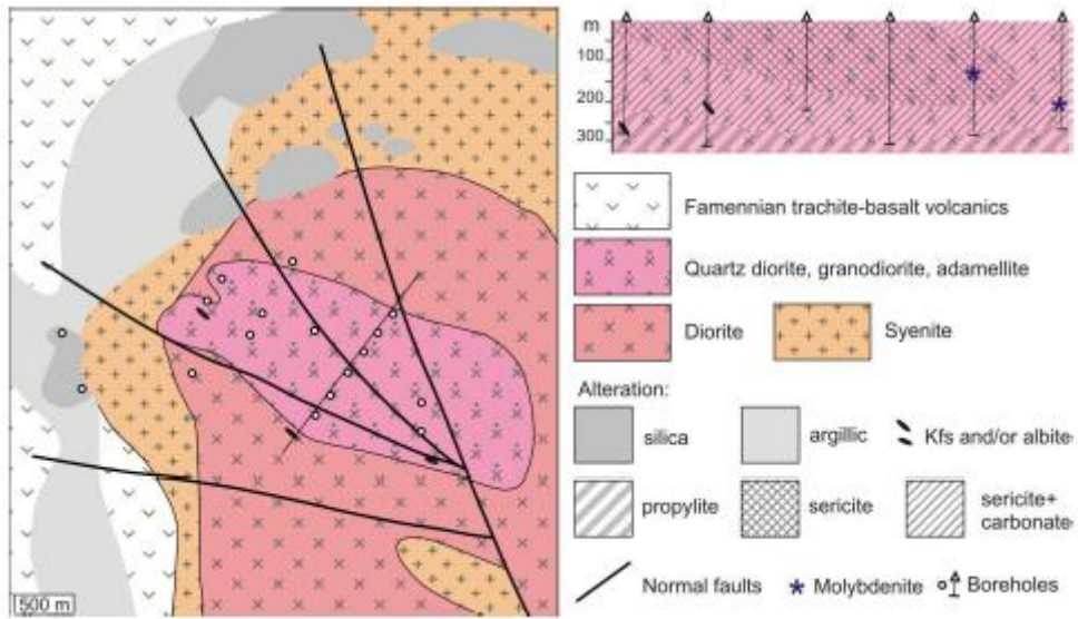
Fig. 5. Schematic geological map (A) and a cross-section (B) of the Verkhneuralskoe Mo-porphyry occurrence, after (Grabezhev and Belgorodsky, 1992).
