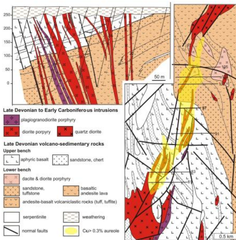
Fig. 8. Geological scheme of the Mikheevskoe deposit after (Shargorodskii et al., 2005) and a cross-section along A-B line adapted from Russian Copper Company.
