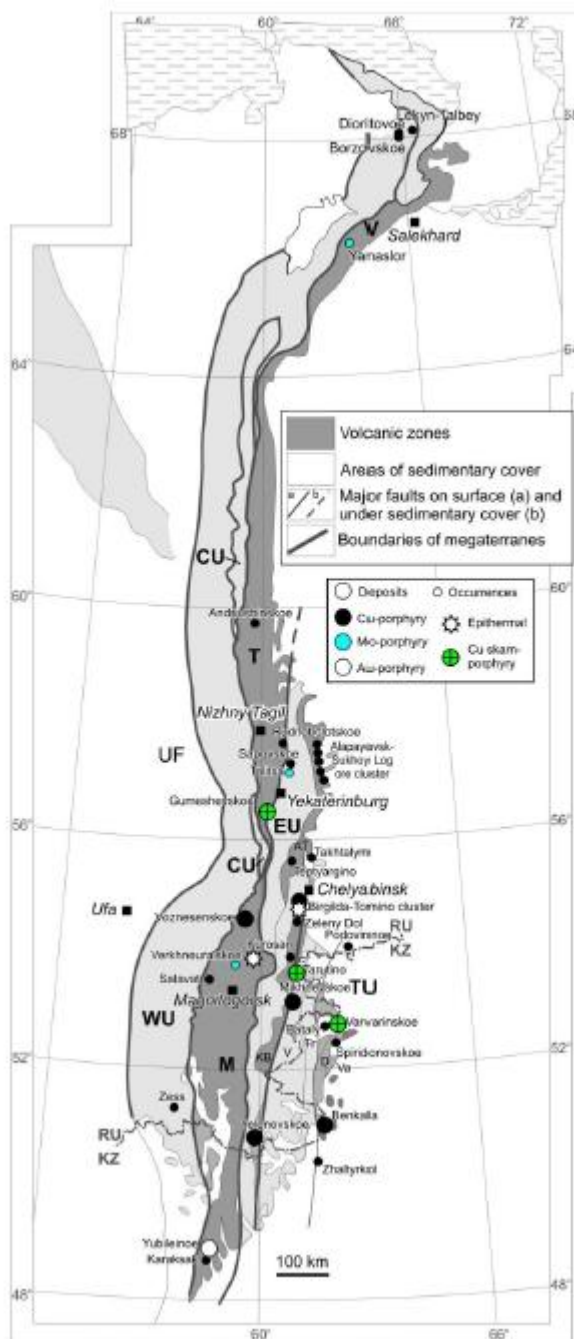
Fig 1. Simplified tectonic scheme of the Urals and locations of porphyry and porphyry related deposits, prospects and occurrences. Modified after (Petrov et al., 2007). Megaterranes: UF – Ural Foredeep, WU – West Uralian; CU – Central Uralian; M – Magnitogorsk; EU – East Uralian with Alapaevsk-Techa (AT) and Kosobrodka-Bredy (KB) volcanic terranes, TU – Trans Uralian megaterrane with Varna (Var), Troitsk (Tr), Alexandrov (A), Denisov (D) and Valerianovka (Val) terranes.
