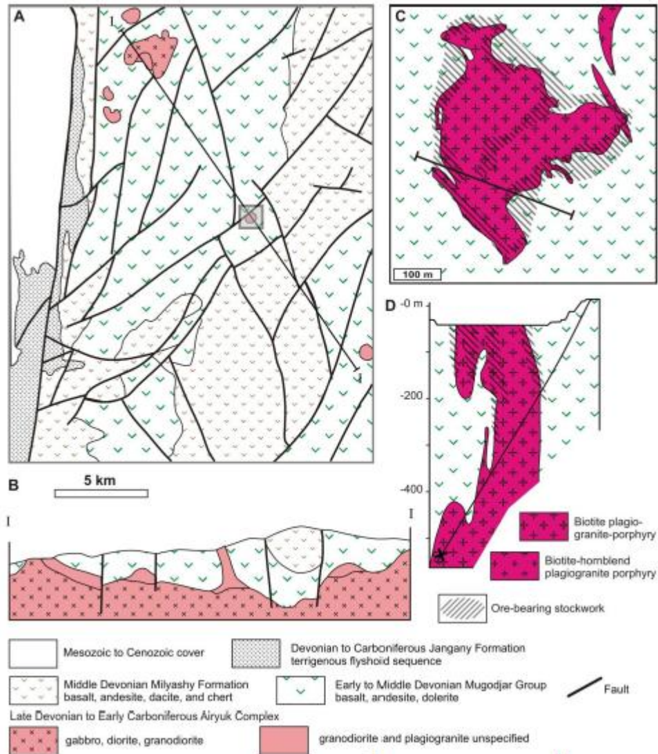
Fig. 3. Geological scheme of the Yubileinoe deposit area (A), cross-section along I–I line (B) and map of the Yubileinoe deposit. A and B are derived from (Seltmann et al., 2014), C– adapted from (Narvait et al., 1974), D – simplified from (Grabezhev and Belgorodskii, 1992).
