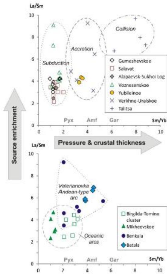
Fig. 16. La/Sm versus Sm/Yb diagram for intrusions associated with porphyry mineralization from Magnitogorsk megaterrane (a) and East- and Trans- Uralian megaterranes (b). Modified from (Kay and Mpodozis, 2001; Zarasvandi et al., 2016)
