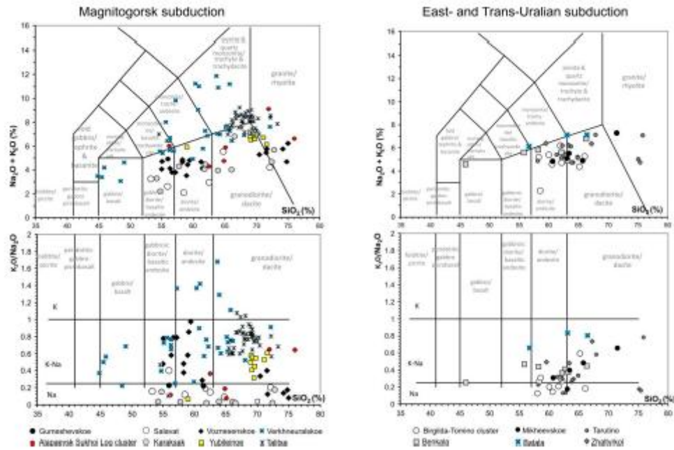
Fig. 11 K+Na – SiO 2 (a) and K/Na – SiO 2 diagrams for the least altered porphyry rocks of the Tagil-Magnitogorsk (A,C) and East- and Trans-Uralian megaterranes (B,D). Data from the Appendix A.
