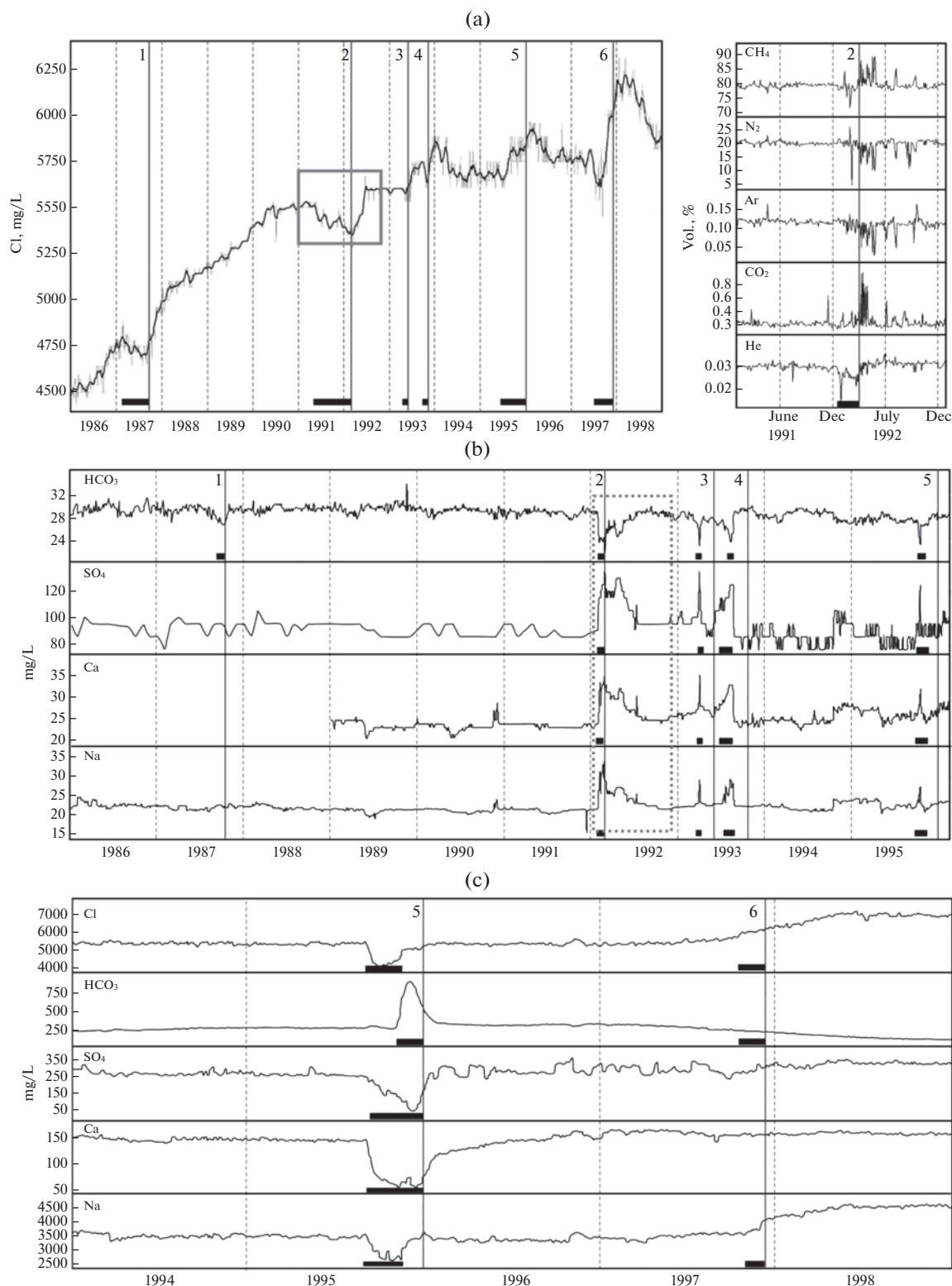
Fig. 2. Pre-earthquake anomalous variations (bold horizontal lines) in the parameters of the ionic and gas composition of ground-water from the wells: (a) GK-1, (b) M-1, (c) G-1. Vertical lines show the 1987–1997 earthquakes, earthquake numbers correspond to Table 2. The grey rectangle highlights variations in the concentration of \text{Cl}^- in the water from GK-1 Well, the grey dashed rectangle highlights variations in the concentration of \text{HCO}_3^- , \text{SO}_4^{2-} , \text{Ca}^{2+} and the concentration of \text{Na}^+ in the water from M-1 Well due to the March 2, 1992 earthquake (Table 2) (according to (Kopylova and Boldina, 2020; 2021; Kopylova et al., 2022)).
