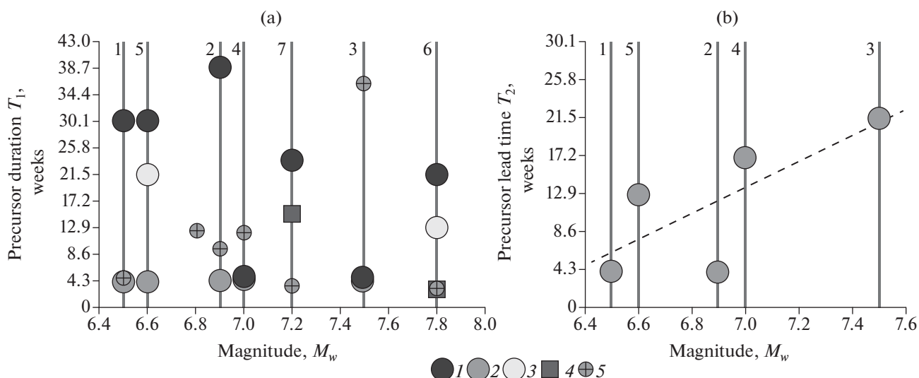
Fig. 4. (a) Distribution of the precursor duration T_1 in the observation wells: 1 – GK-1, 2 – M-1, 3 – G-1, 4 – YUZ-5, 5 – E-1, depending on the magnitude M_w of earthquakes No. 1–7 in Table 2; the earthquakes are shown with grey vertical lines. (b) Distribution of the lead time T_2 of the hydrogeochemical precursor in M-1 Well (Fig. 2b), depending on the magnitude M_w of earthquakes No. 1–5 (linear correlation coefficient 0.74).
