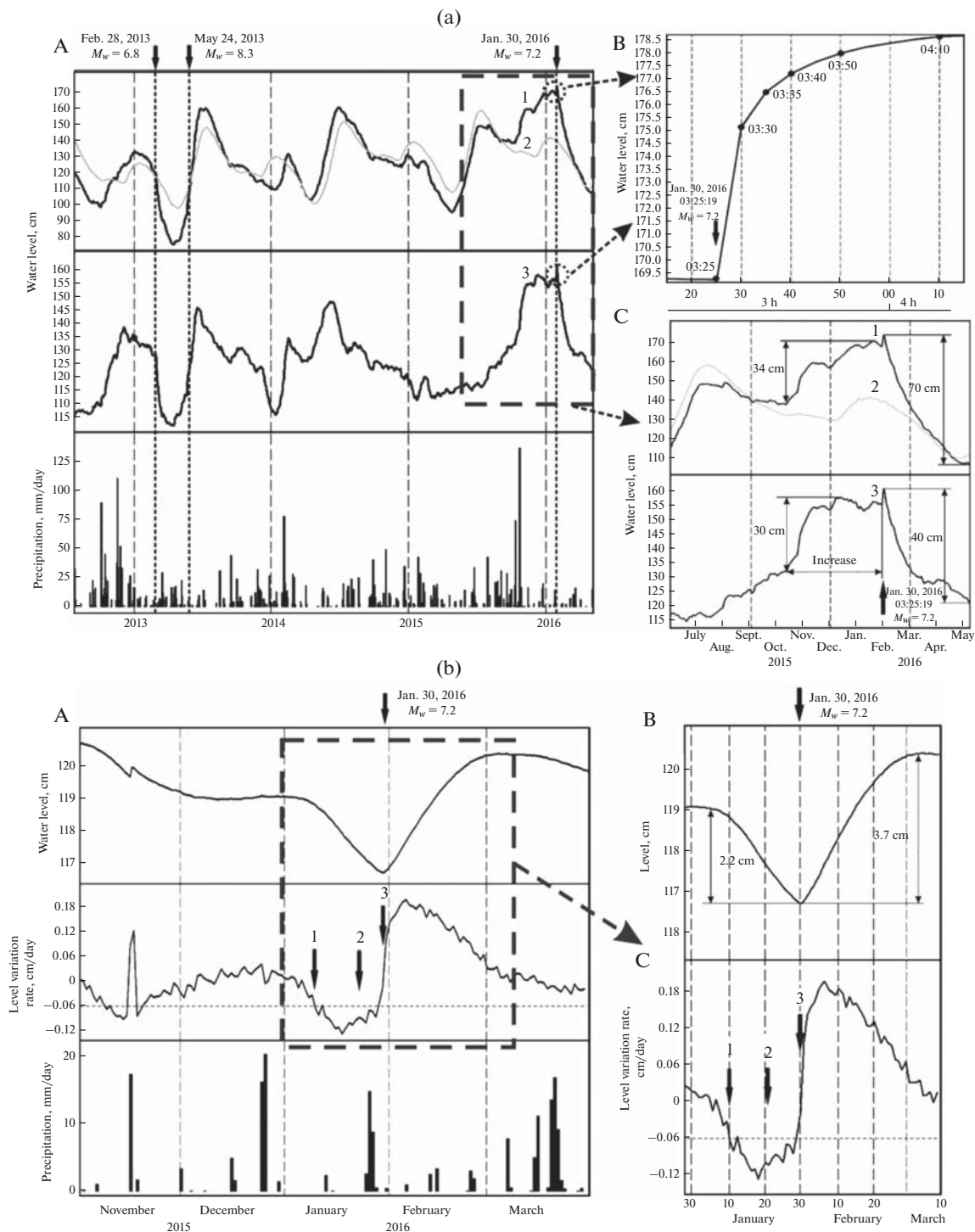
Fig. 1. Variations in the water level in YUZ-5 (a) and E-1 (b) Wells due to the M_w = 7.2 Zhupanovsky earthquake (below - ZhE) of January 30, 2016 (Table 2). Variations in the water level in YUZ-5 Well: A—water level variations in July 2012—May 2016, against precipitation and M_w \geq 6.5 earthquakes (indicated with arrows): 1—hourly average observational data with compensated barometric variations; 2—seasonal water level variations; 3—residuals in the water level variations after compensation of the annual seasonality and trend: the bold dashed line indicates the fragment of graphs during ZhE, see Fig. c); b—a coseismic increase in the water level after the onset of seismic waves (03:25); c—precursor and postseismic water level variations. Variations in the water level and its daily average rate in E-1 Well: A—from November 2015 to March 2016, against precipitation; ZhE is indicated with an arrow. In the graph of the daily average rate of water level variations, numbers show: January 1—10—the onset of the hydrogeodynamic precursor, January 2—21—the date of submission of a forecast report on a potential strong earthquake to KB REC, January 3—30—ZhE; the dashed line indicates the threshold water level decrease rate -0.06 cm/day; the bold dashed line outlines the fragment of water level variations, shown in the figures: B—water level variations from December 30, 2015 to March 10, 2016, including a hydrogeodynamic precursor and a postseismic increase; C—change in the daily average water level variations rate against its threshold -0.06 cm/day (according to (Boldina and Kopylova, 2017)).
